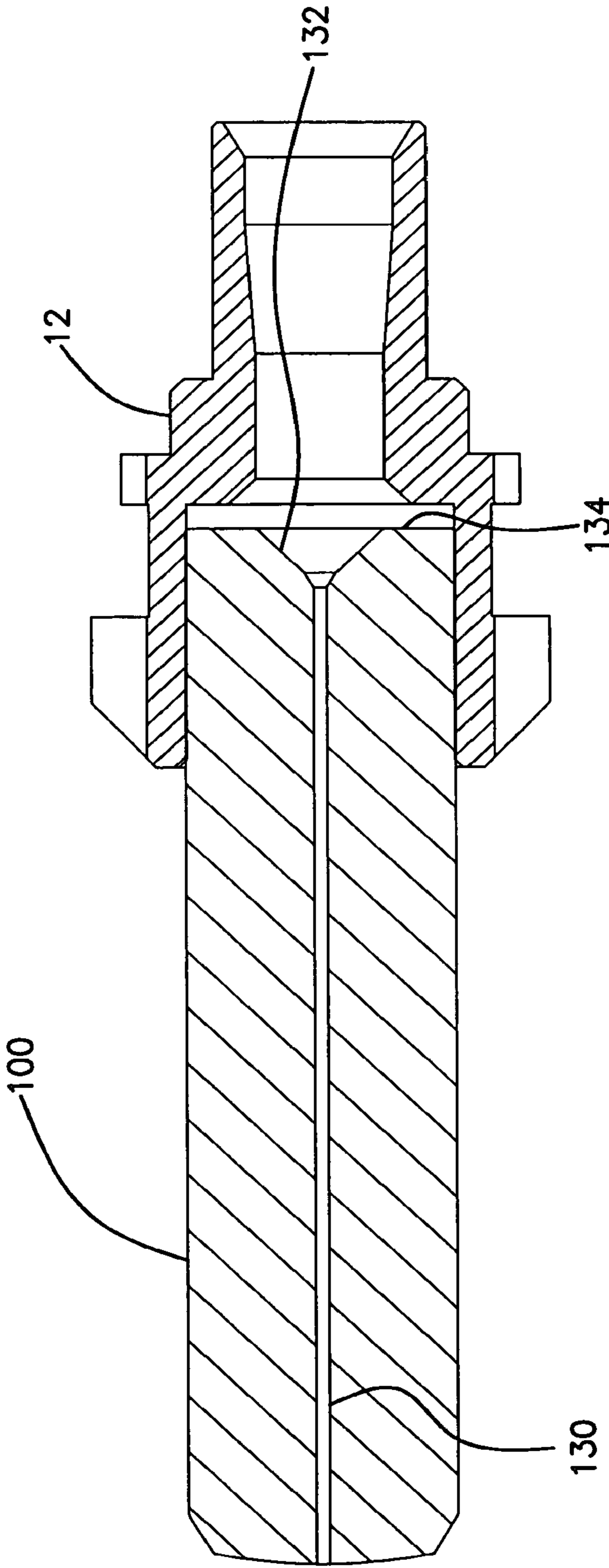
FIG. 8 PRIOR ART
