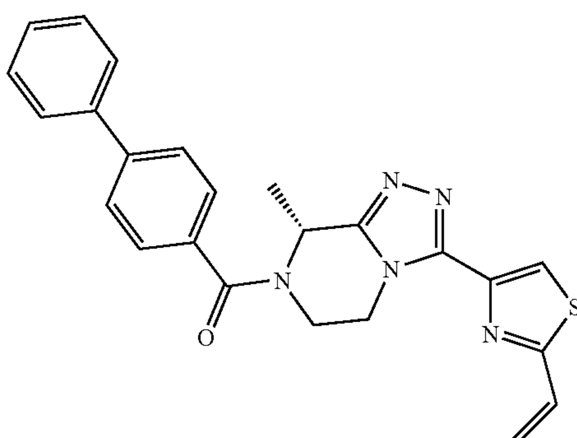
(R)-[1,1'-biphenyl]-4-yl(8-methyl-3-(2-vinylthiazol-4-yl)-5,6-dihydro-[1,2,4]triazolo[4,3-a]pyrazin-7(8H)-yl)methanone
