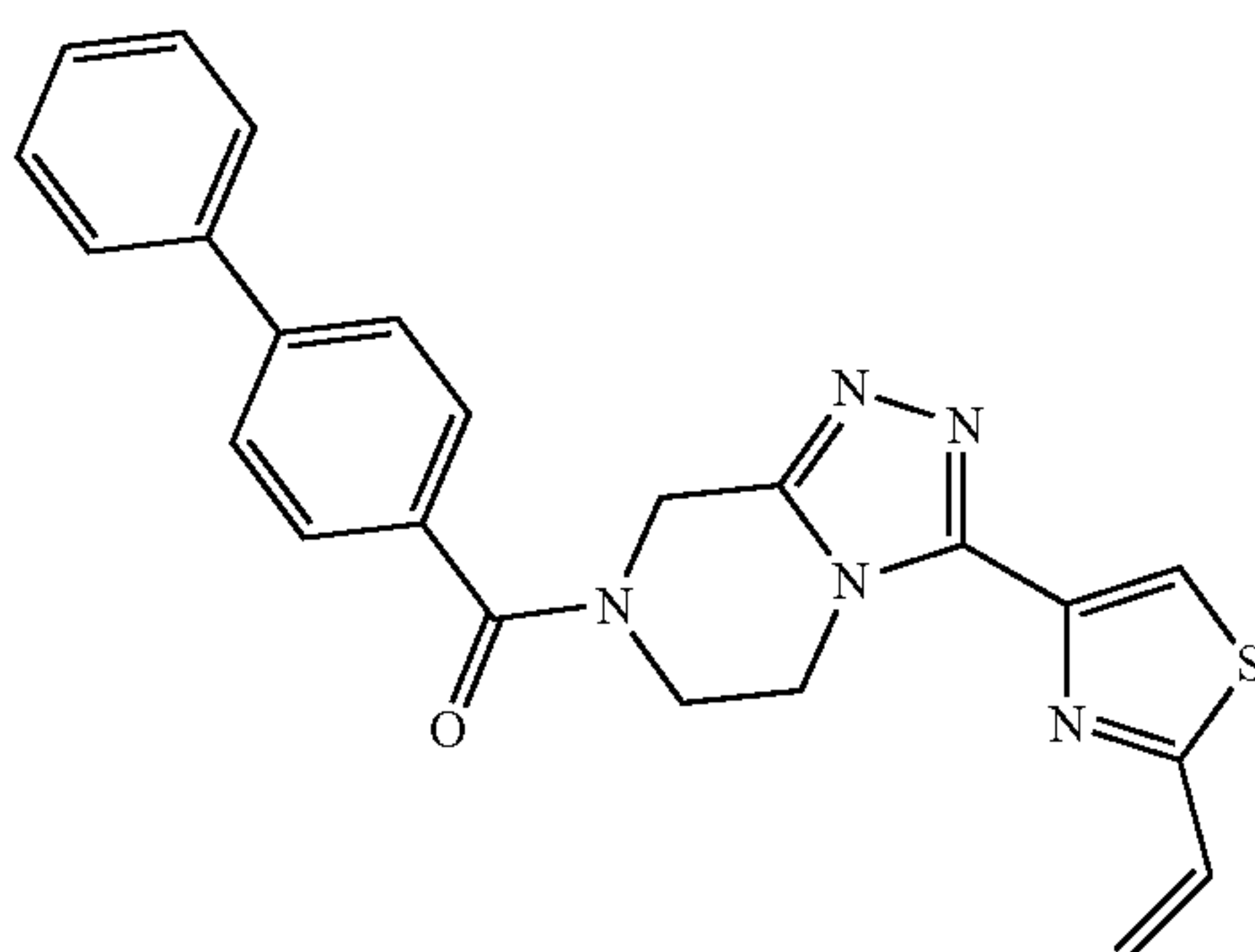
[1,1'-biphenyl]-4-yl(3-(2-vinylthiazol-4-yl)-5,6-dihydro-[1,2,4]triazolo[4,3-a]pyrazin-7(8H)-yl)methanone
