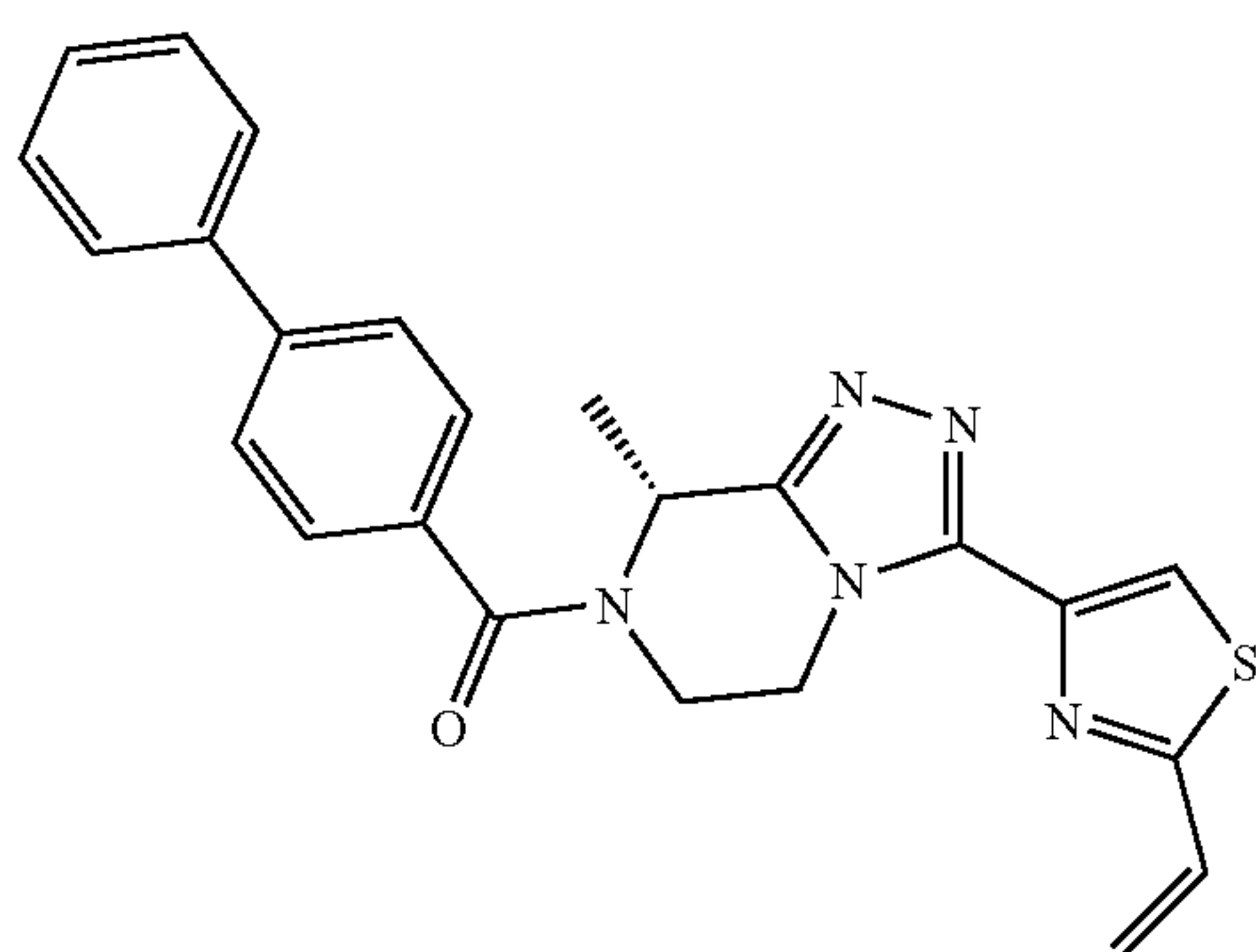
(R)-[1,1'-biphenyl]-4-yl(8-methyl-3-(2-vinylthiazol-4-yl)-5,6-dihydro-[1,2,4]triazolo[4,3-a]pyrazin-7(8H)-yl)methanone
