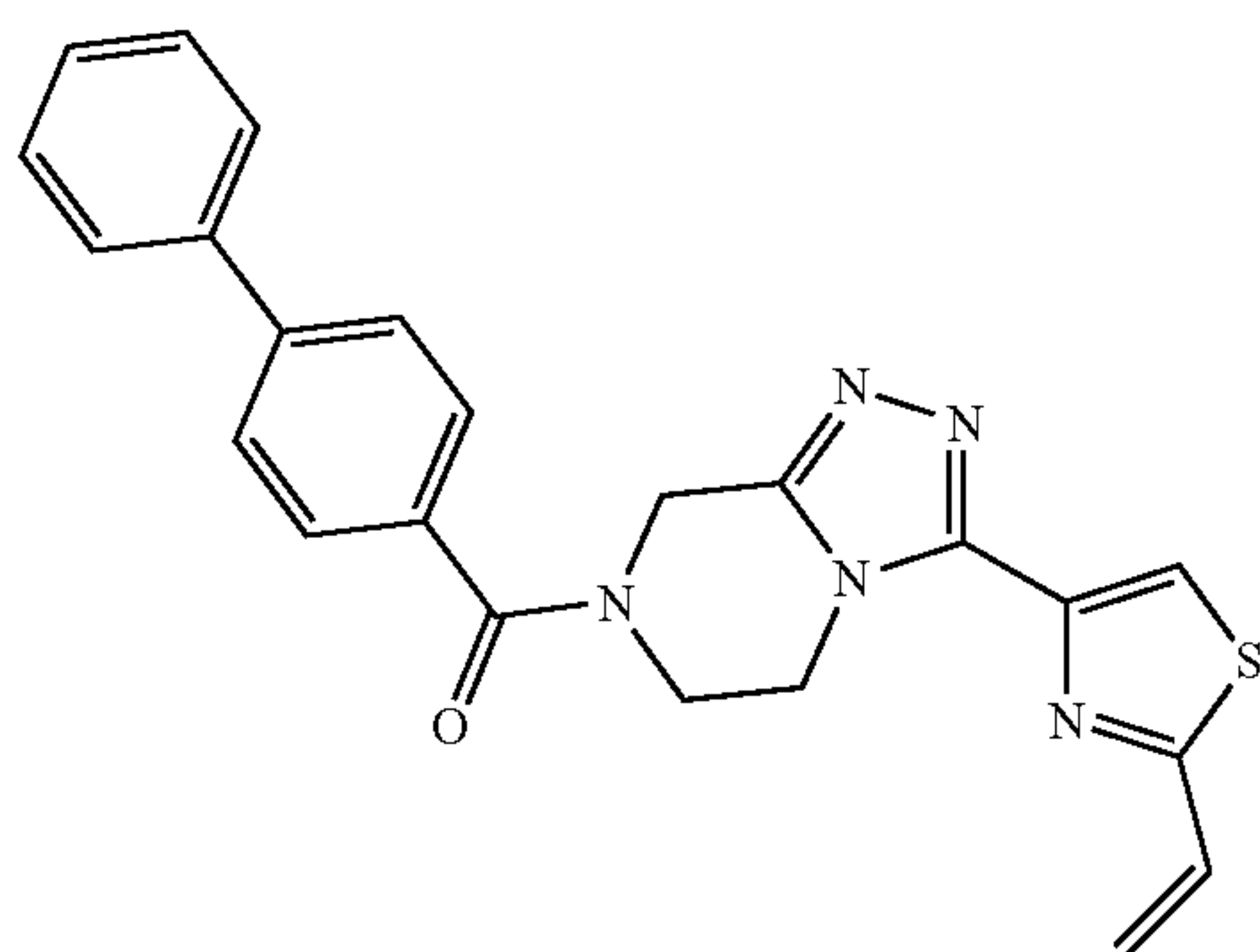
[1,1'-biphenyl]-4-yl(3-(2-vinylthiazol-4-yl)-5,6-dihydro-[1,2,4]triazolo[4,3-a]pyrazin-7(8H)-yl)methanone
