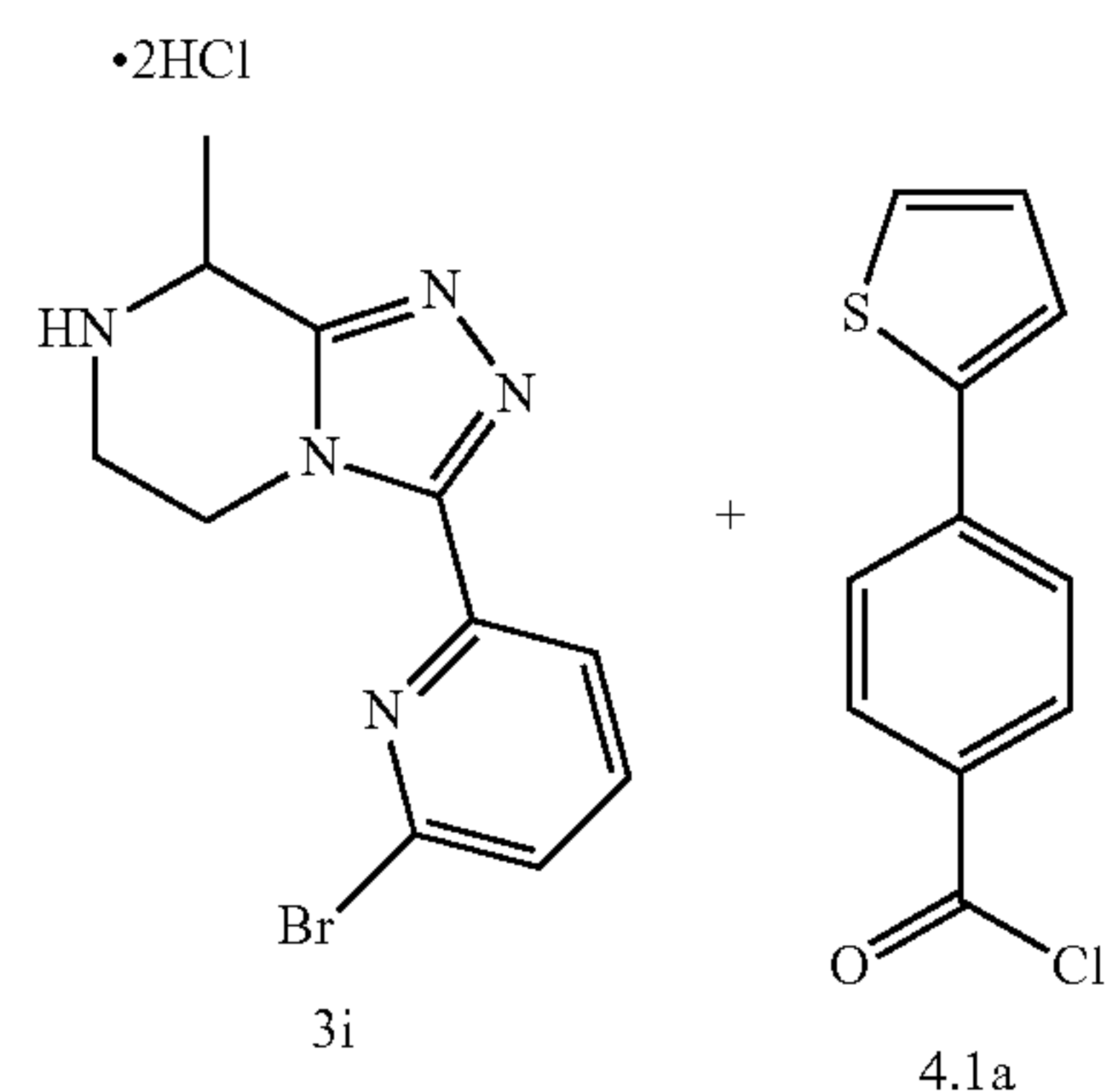
Scheme 29: Synthesis of compound n°33.
