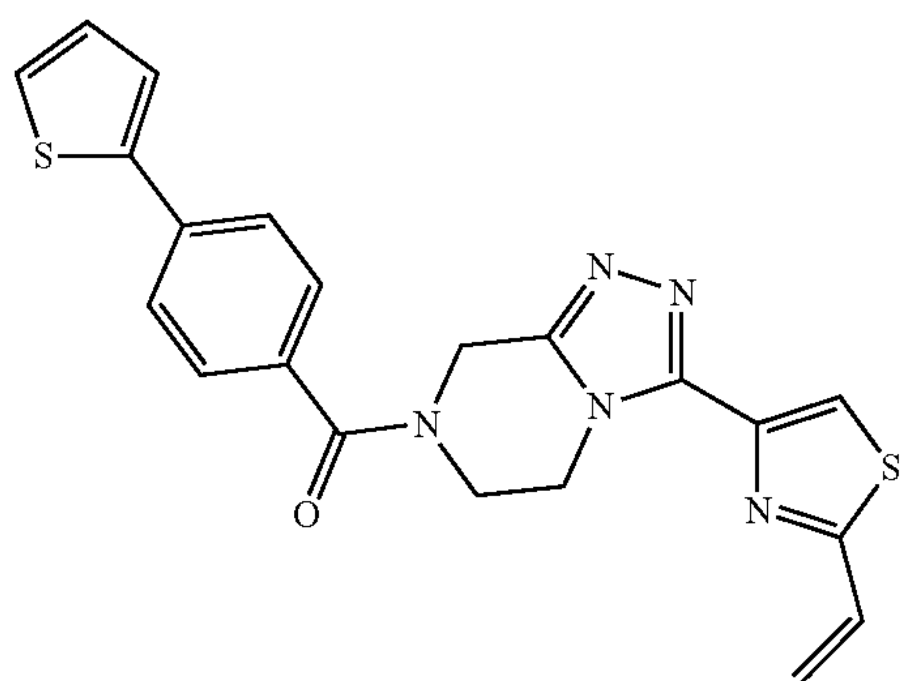
(4-(thiophen-2-yl)phenyl)(3-(2-vinylthiazol-4-yl)-5,6-dihydro-[1,2,4]triazolo[4,3-a]pyrazin-7(8H)-yl)methanone
