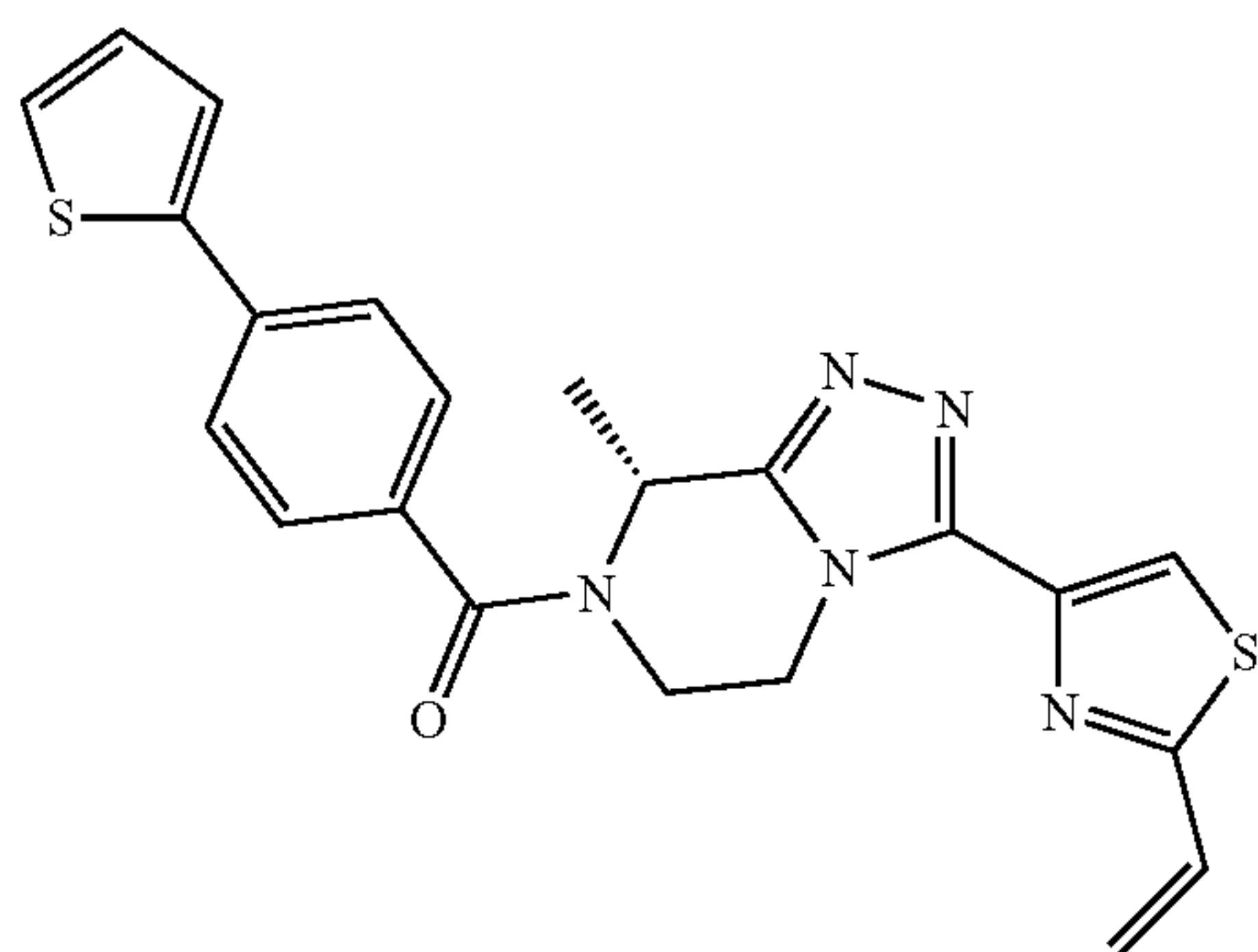
(R)-(8-methyl-3-(2-vinylthiazol-4-yl)-5,6-dihydro-[1,2,4]triazolo[4,3-a]pyrazin-7(8H)-yl)(4-(thiophen-2-yl)phenyl)methanone
