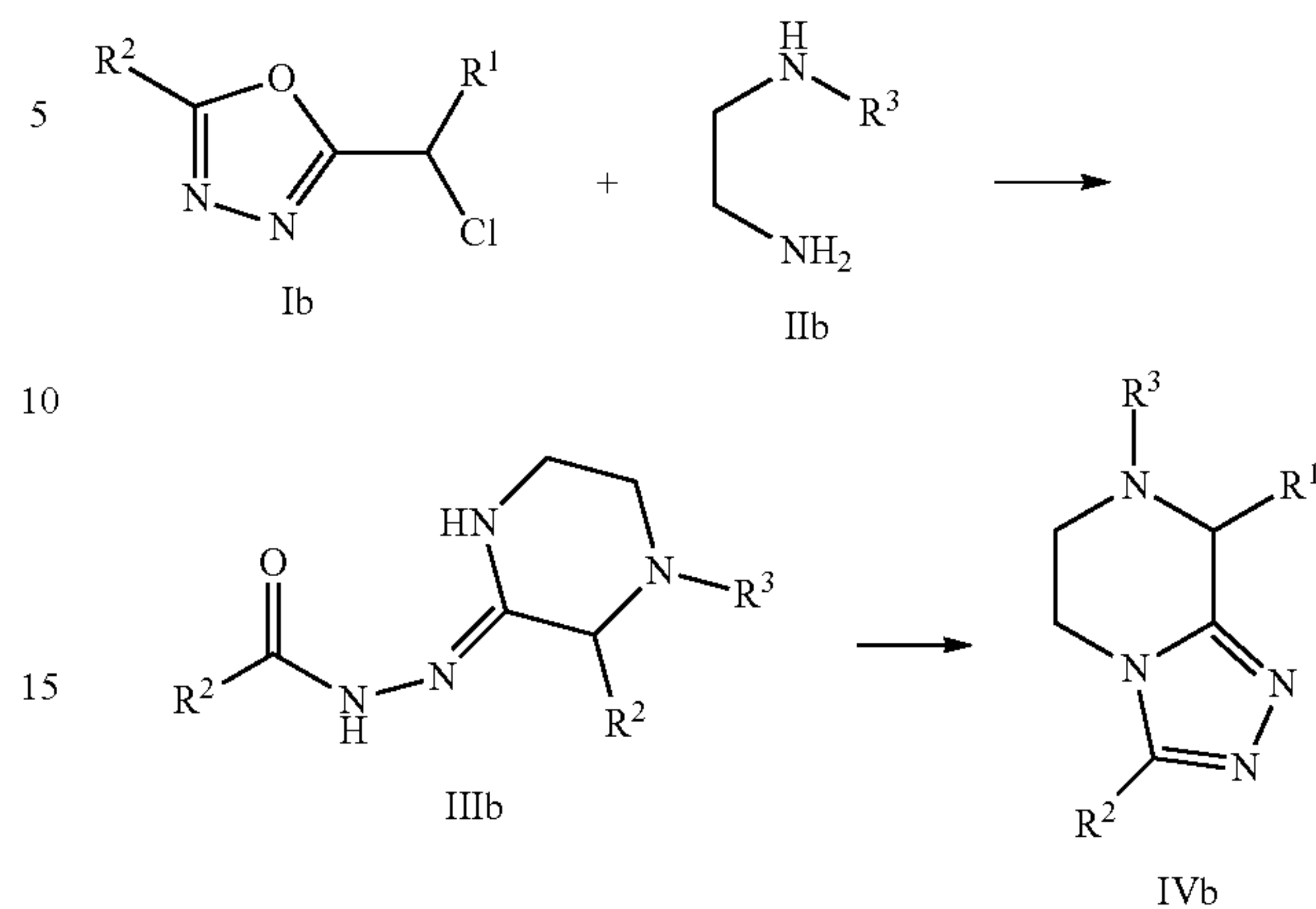
Scheme C: Method B
