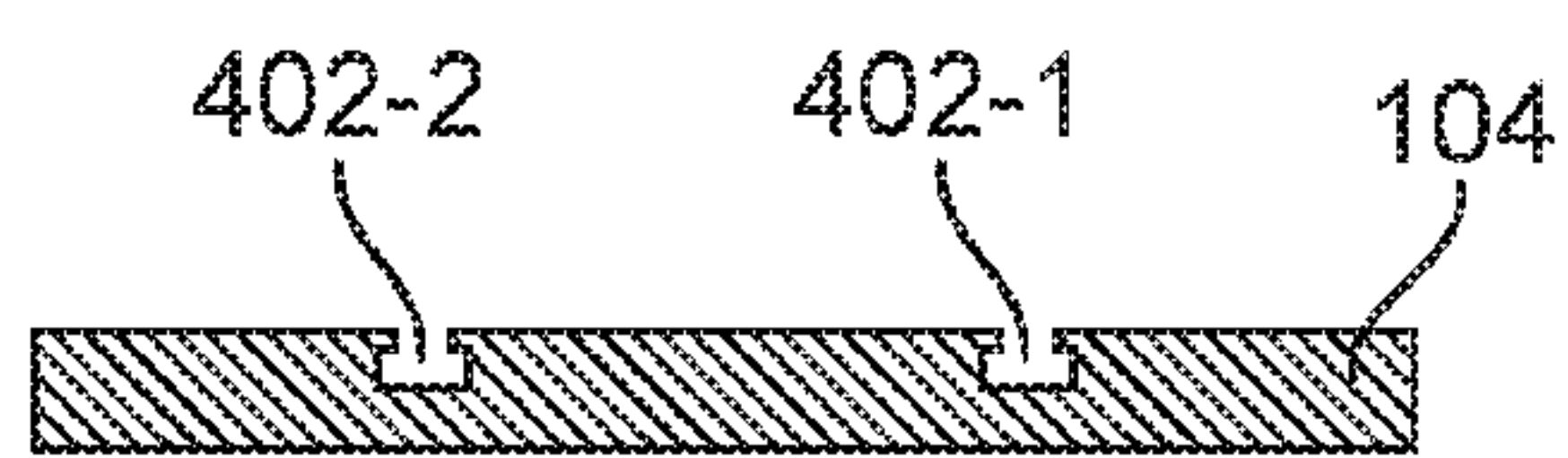
SECTION B-B
