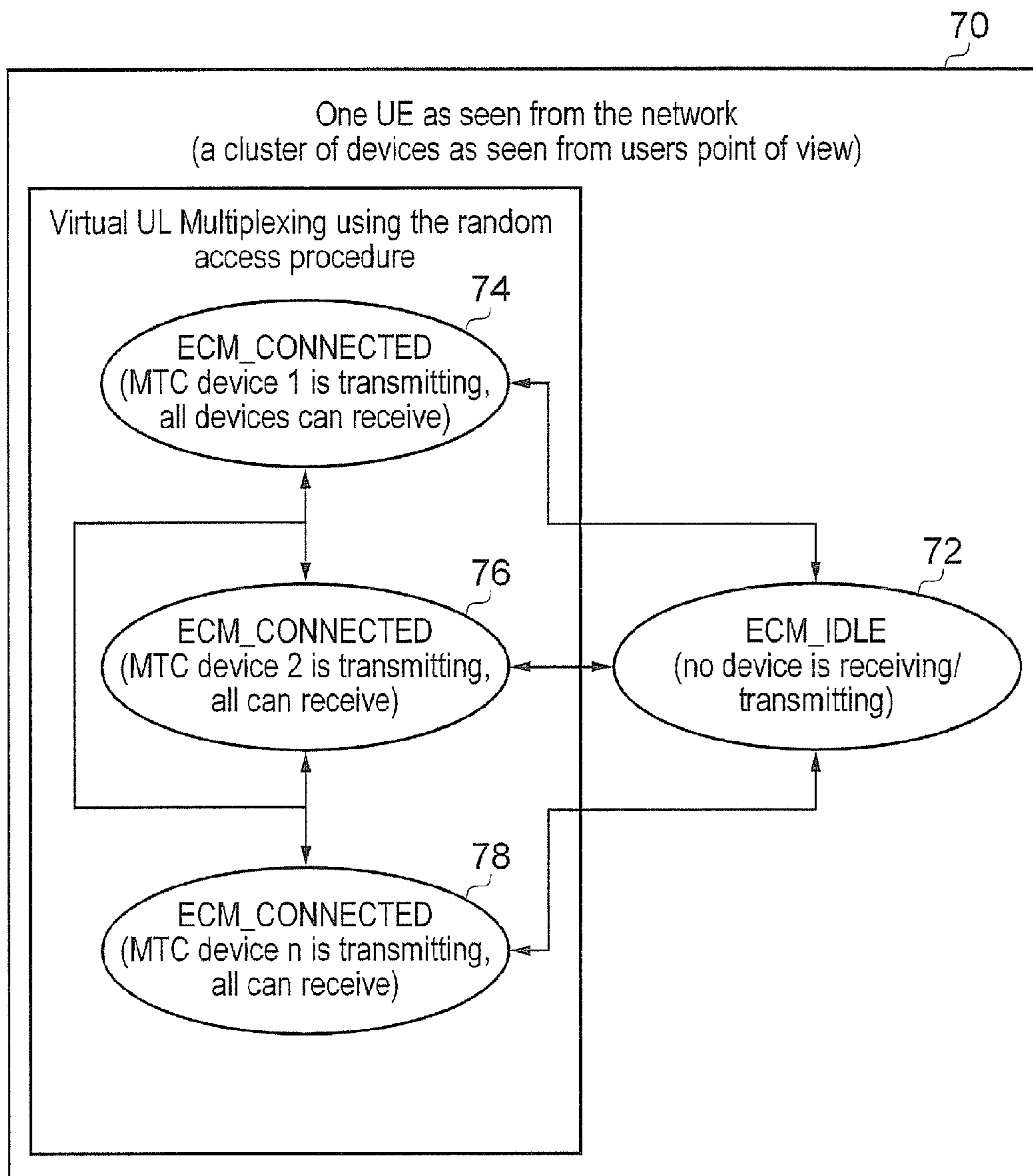
UL virtual multiplexing
