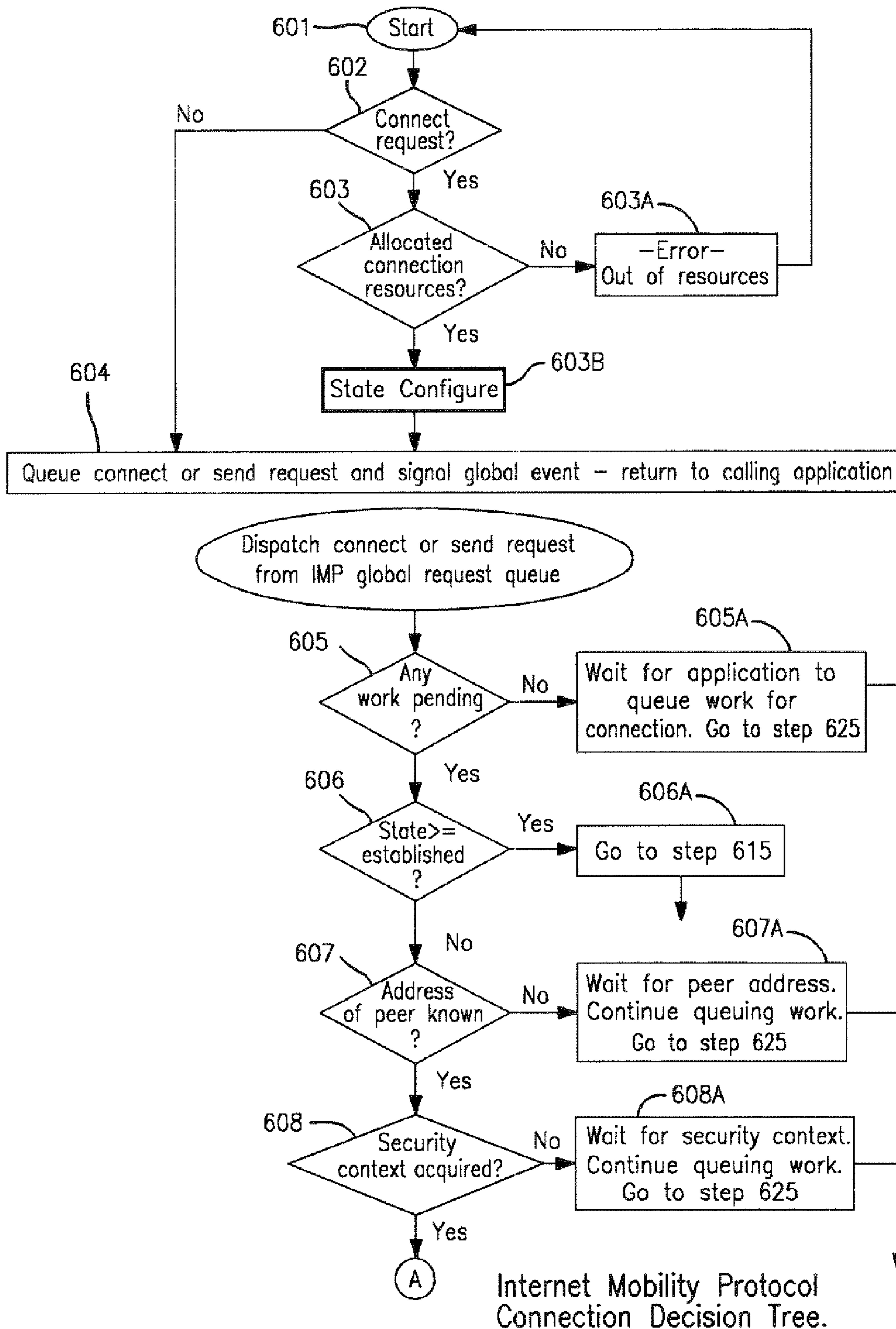
FIG. 10A Connect and Send request logic
