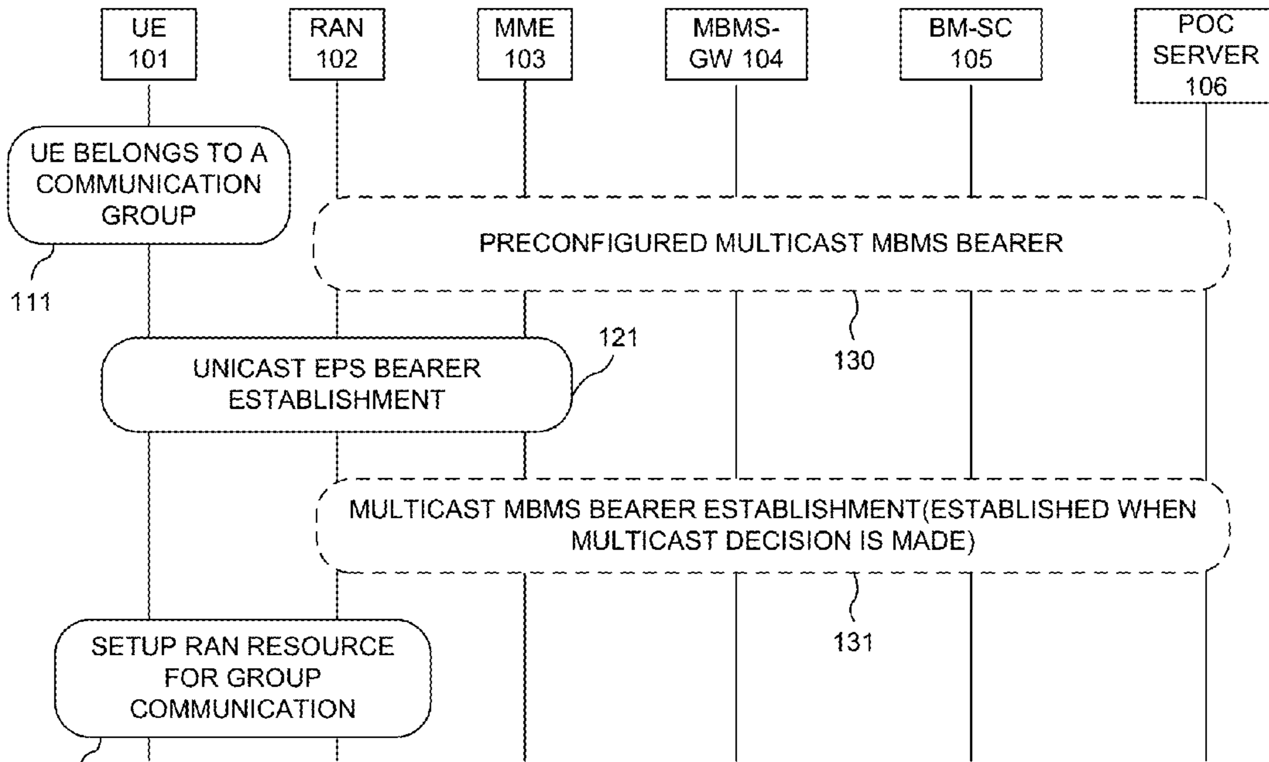
POC DL TRAFFIC MULTICASTING USING MBMS FIG. 1
