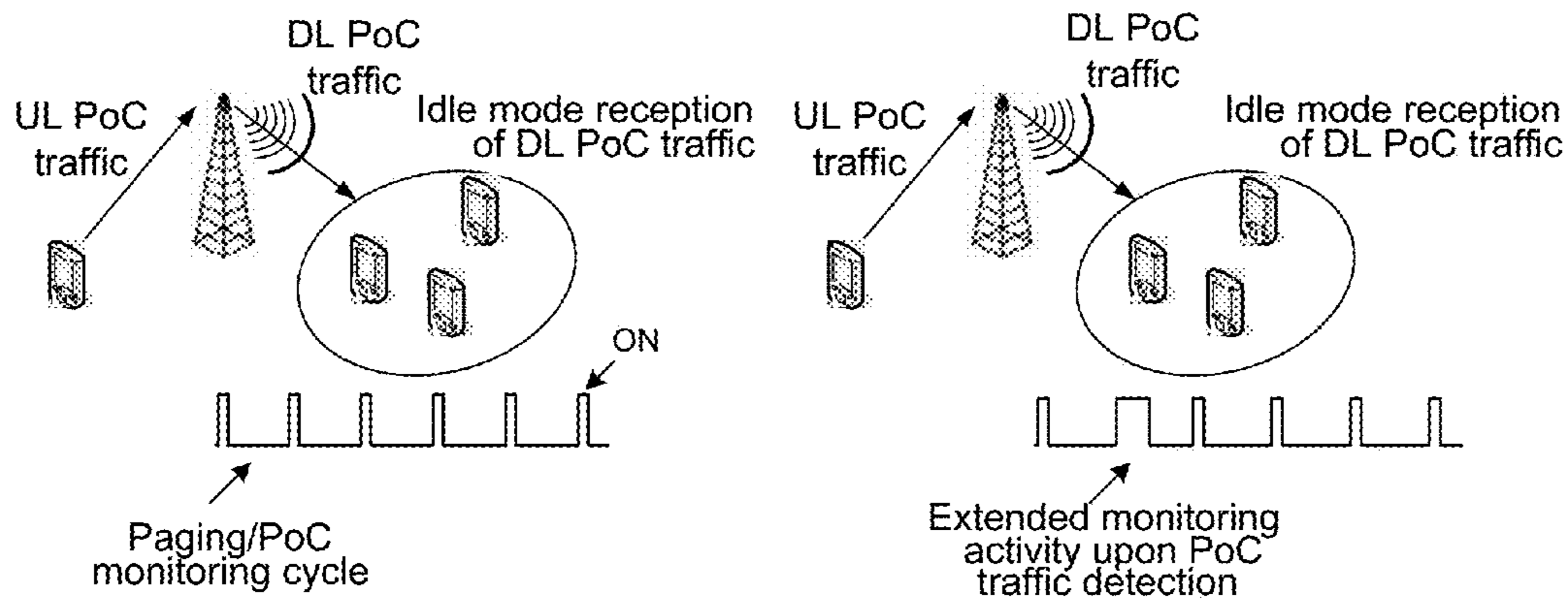
IDEL MODE RECEPTION FOR POC TRAFFIC
