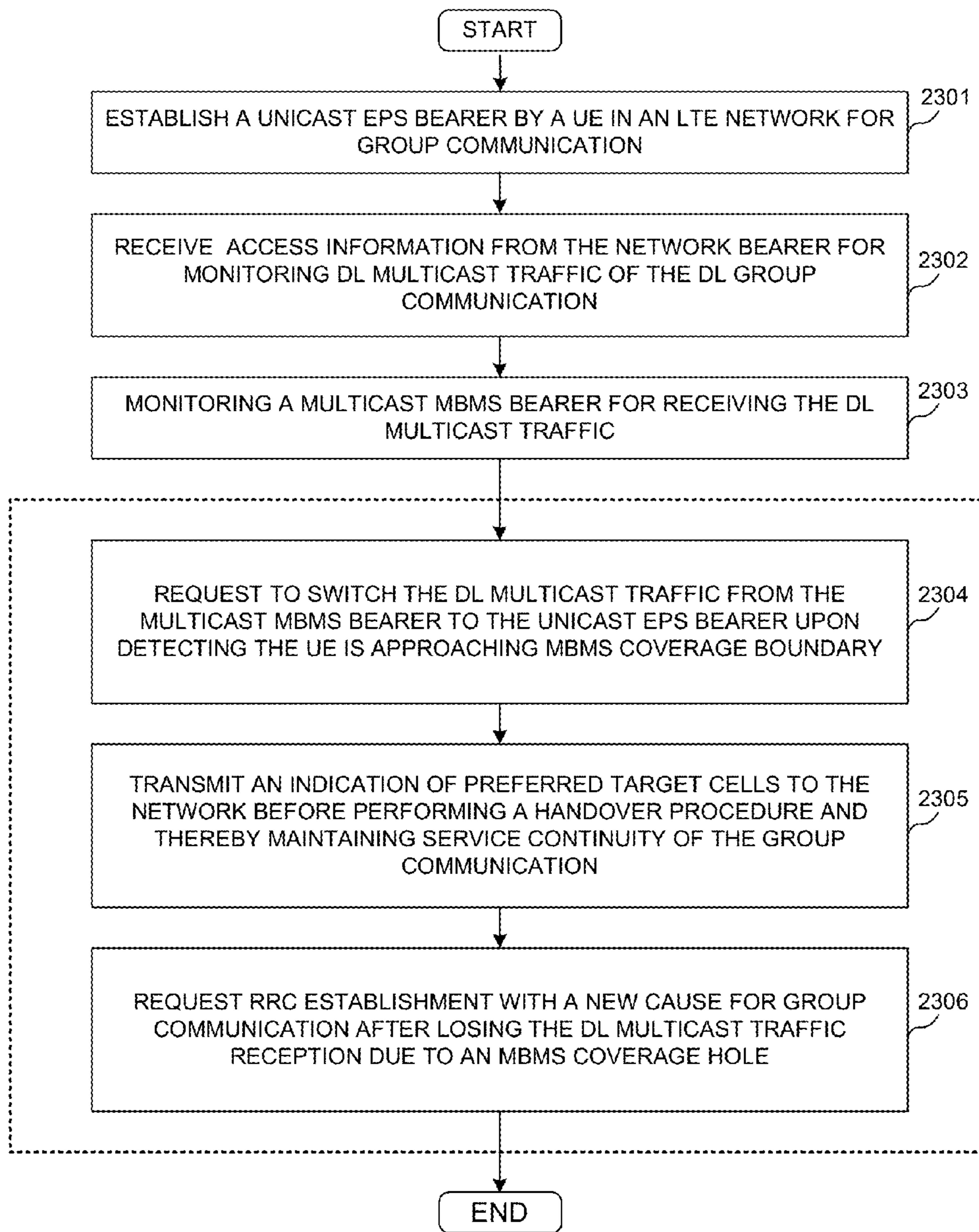
POC MULTICAST TRAFFIC SERVICE CONTINUITY FIG. 23
