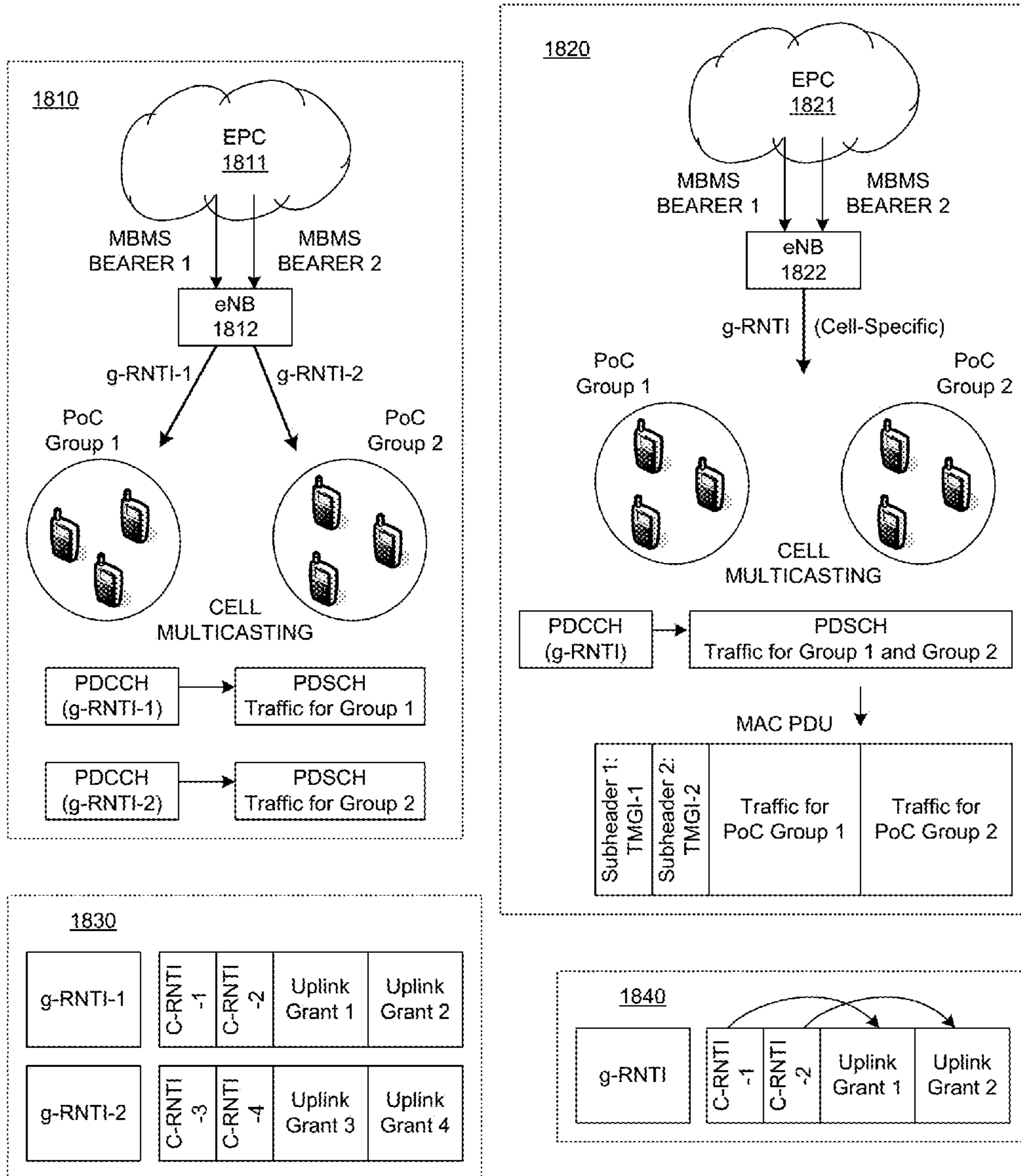
CONTROL SIGNAL REDUCTION FOR SCHEDULING POC TRAFFIC VIA CELL MULTICASTING FIG. 18
