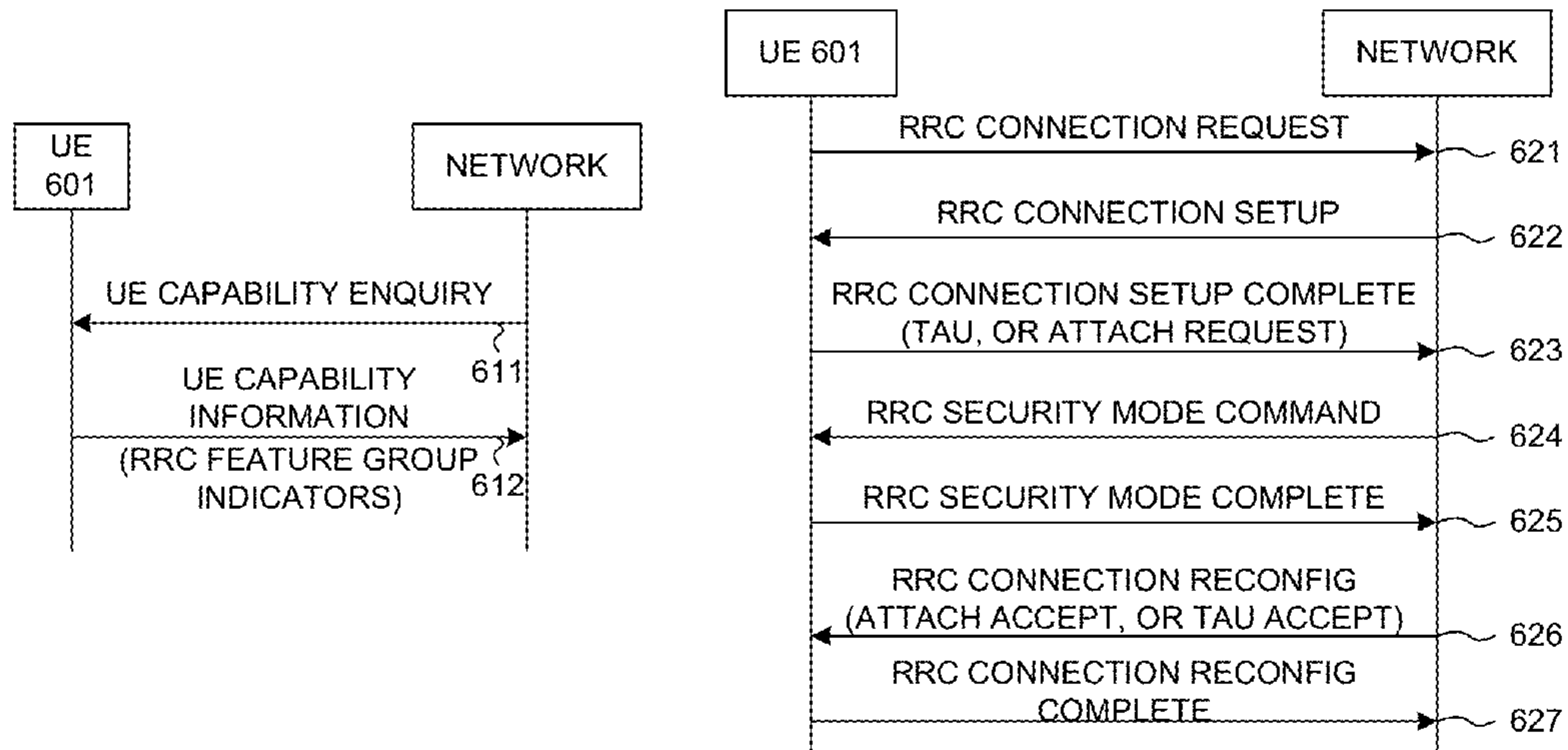
MBMS CAPABILITY INDICATION FIG. 6
