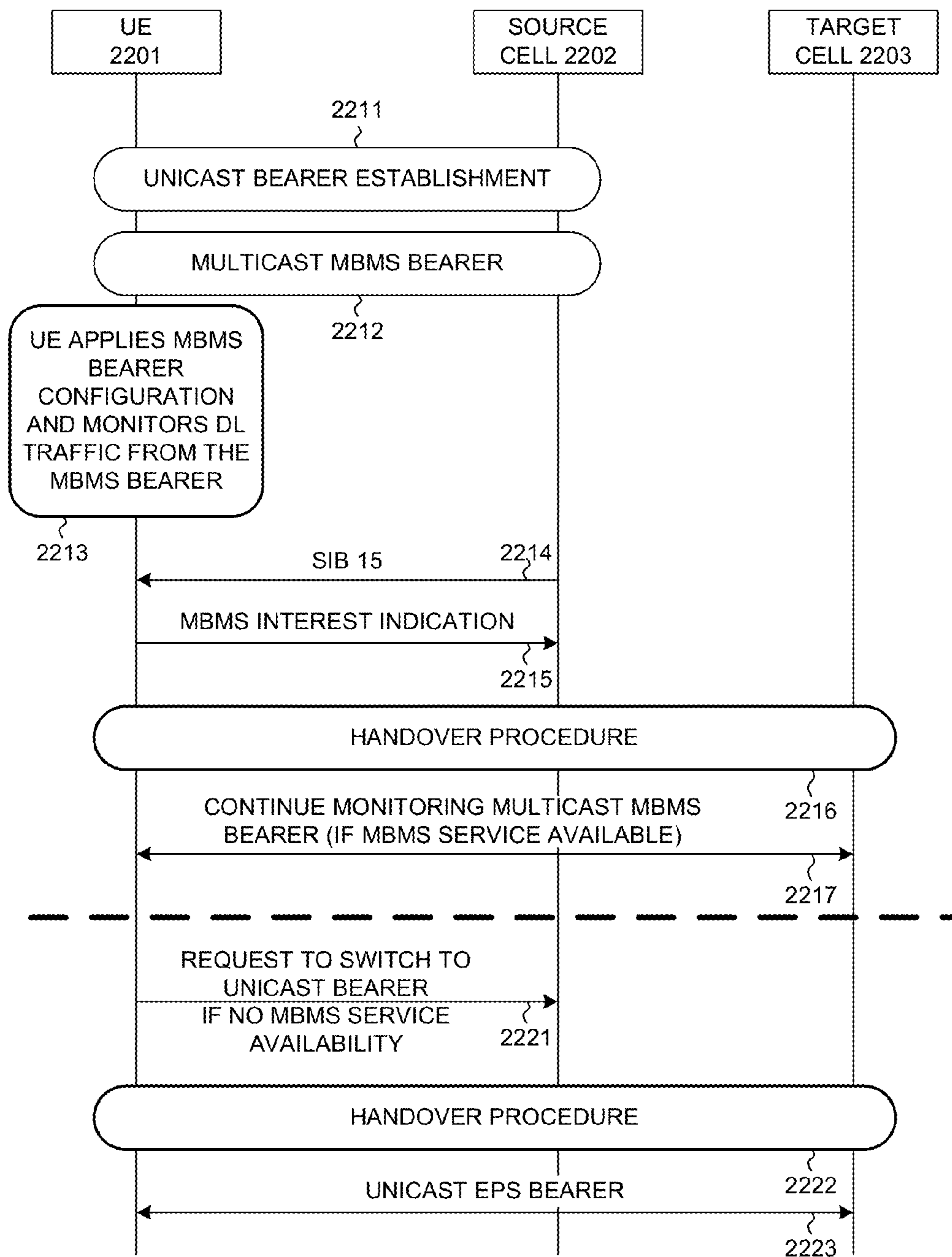
POC MULTICAST SERVICE CONTINUITY
