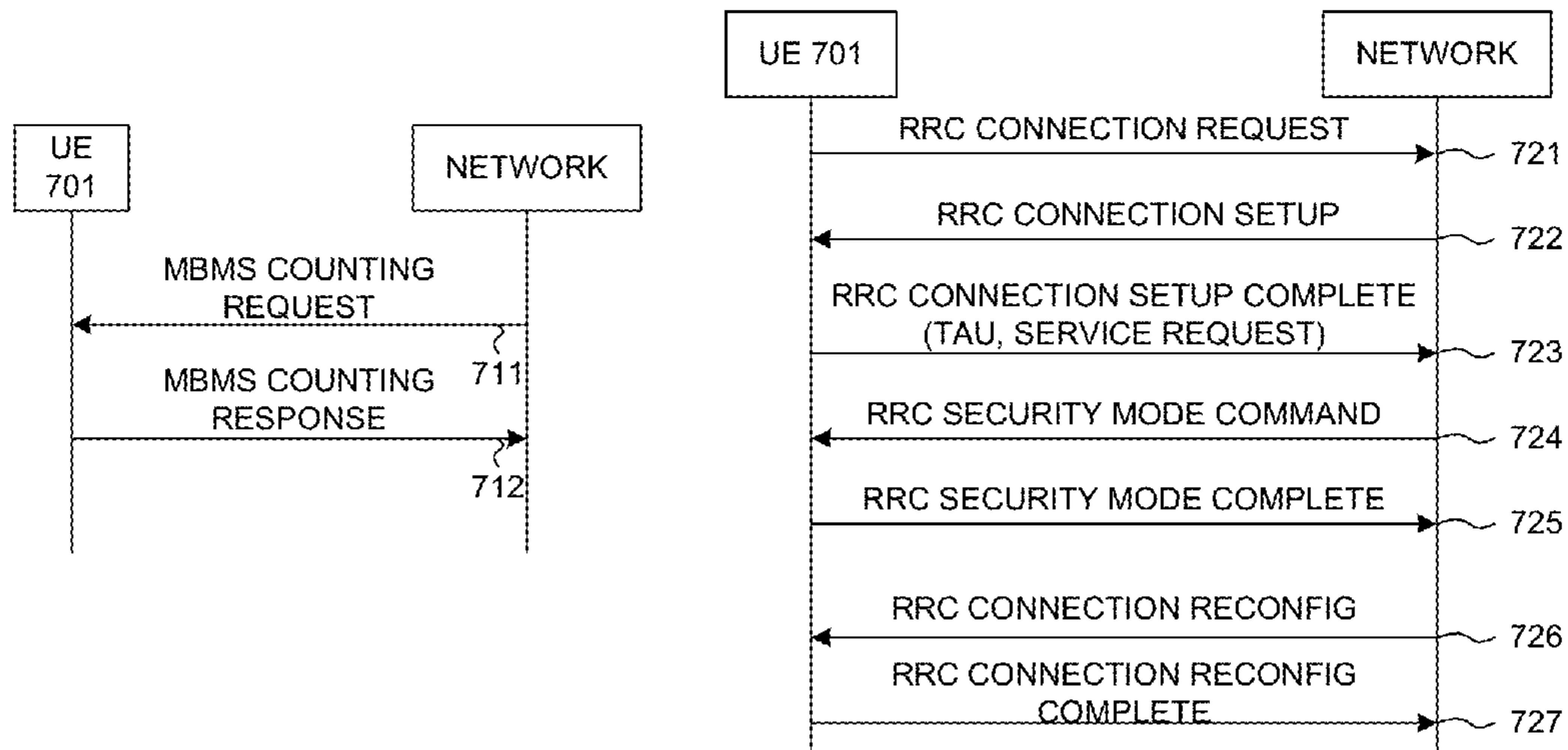
MBMS RECEPTION STATUS INDICATION FIG. 7
