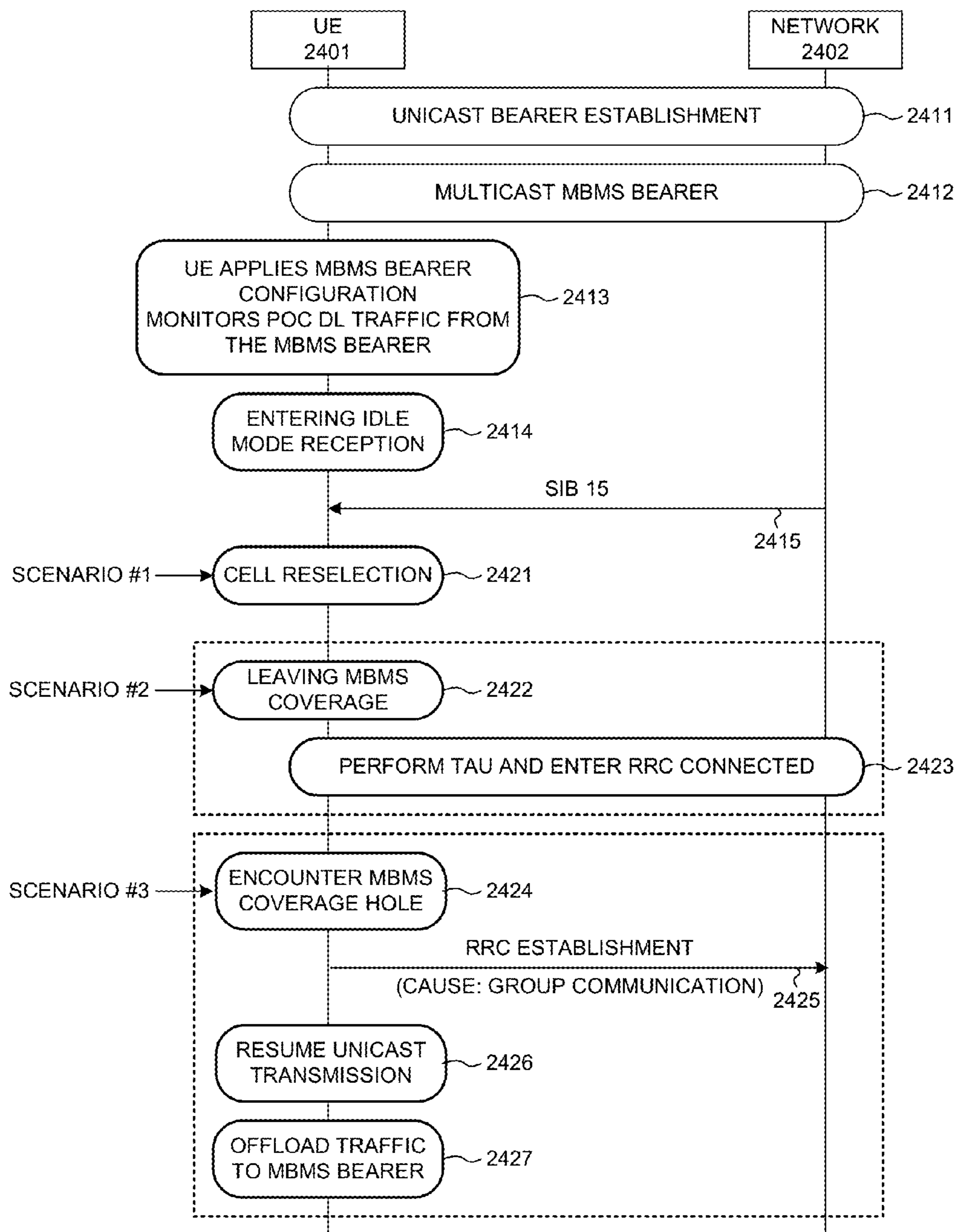
IDLE MODE RECEPTION FOR POC TRAFFIC FIG. 24
