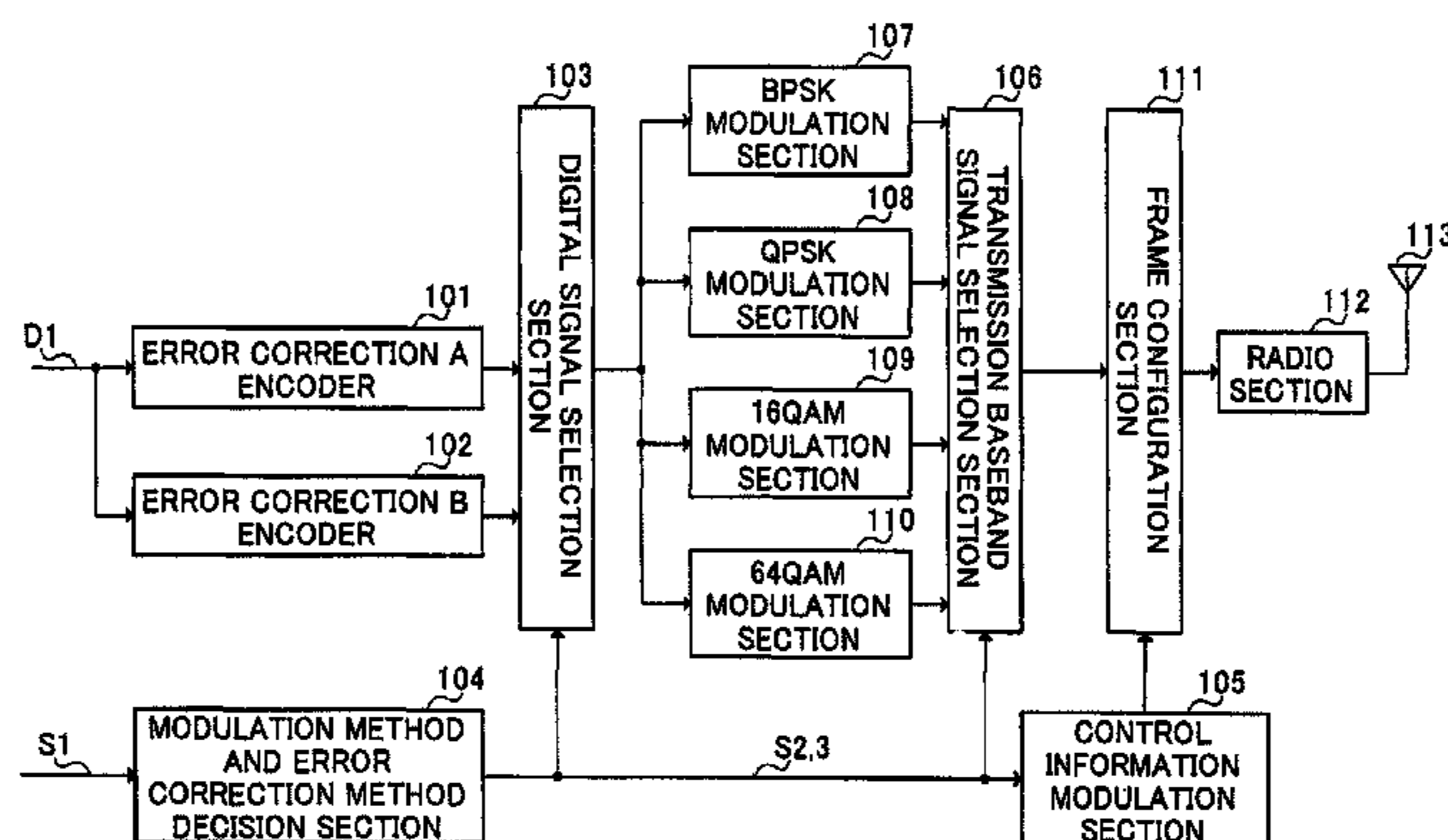
100 TRANSMITTING APPARATUS
