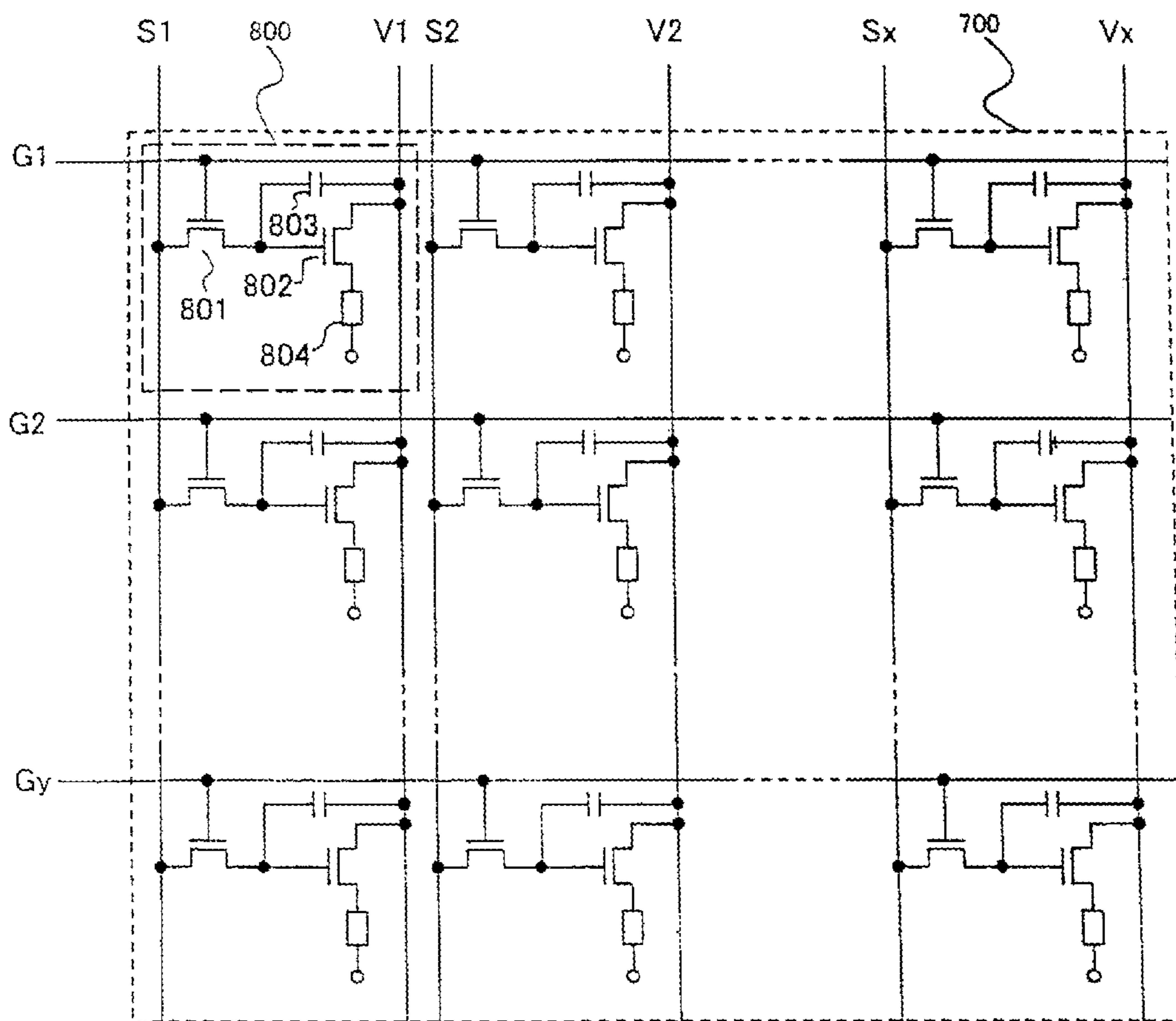
Fig.7 (PRIOR ART)
