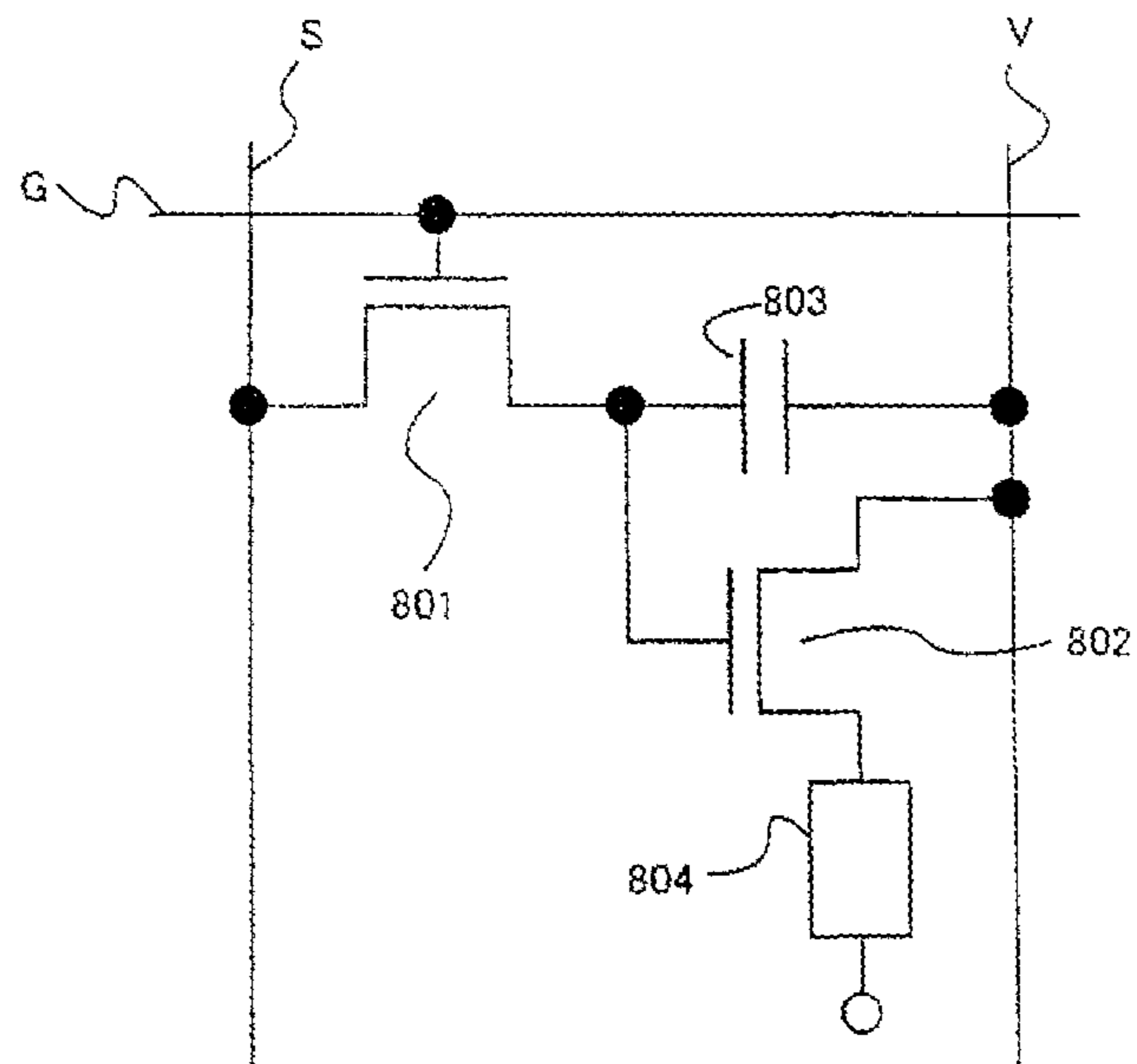
Fig.8 (PRIOR ART)
