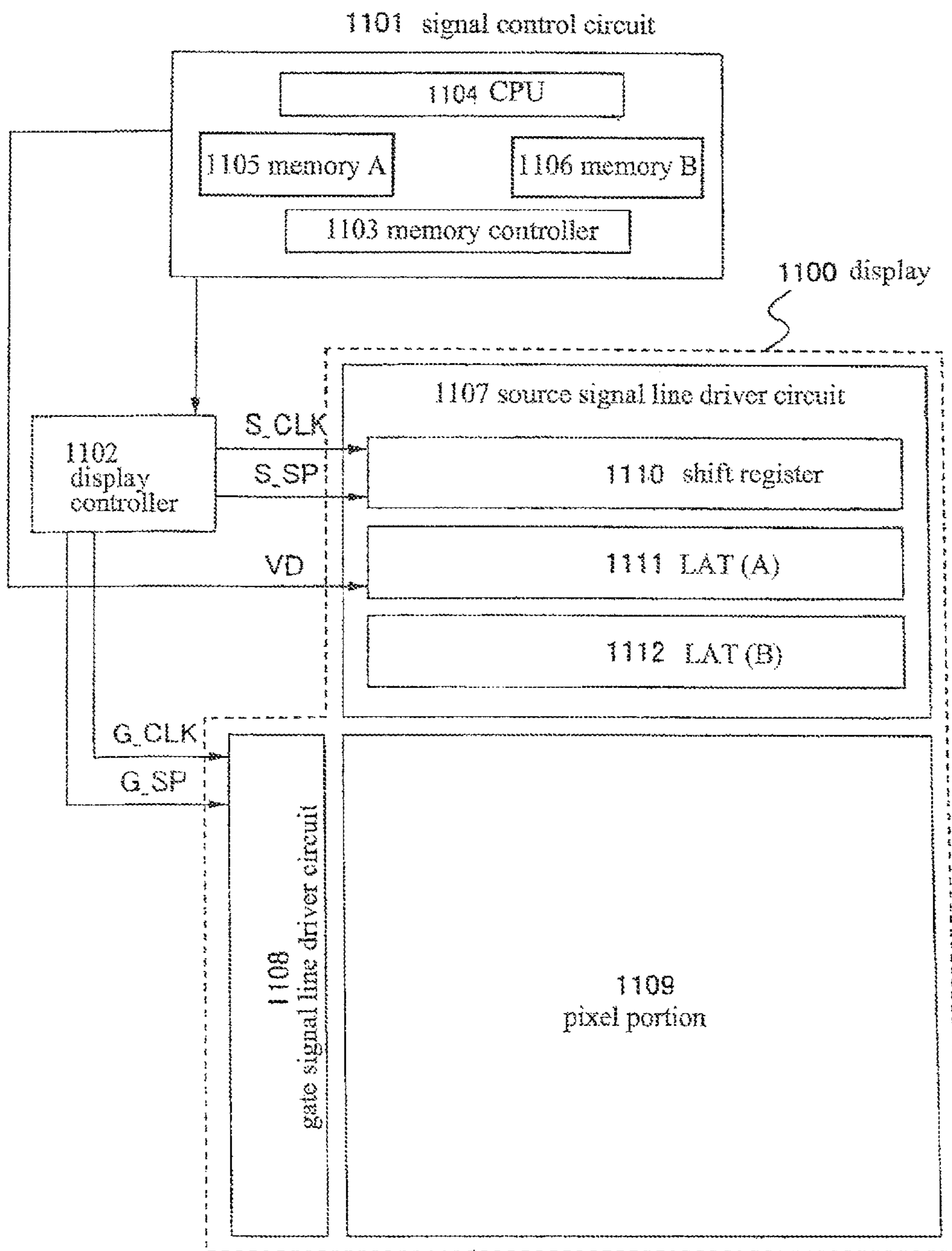
Fig.10 (PRIOR ART)
