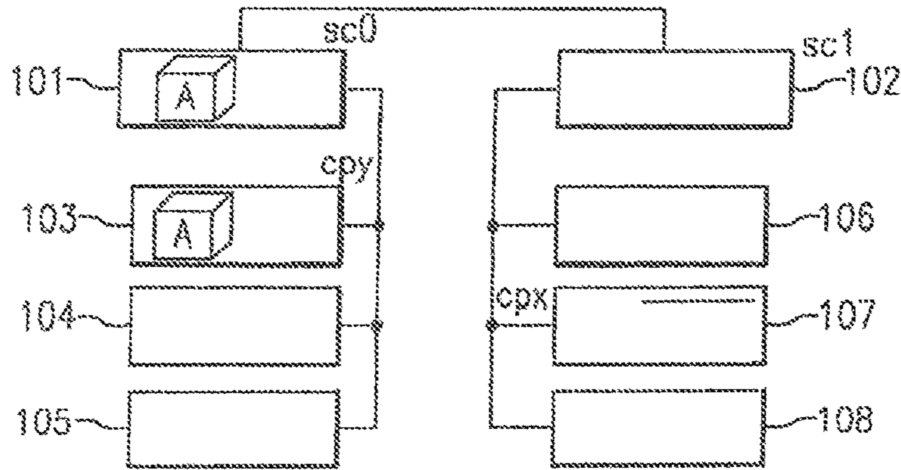
-LINE A EXISTS WRITE (EXCLUSIVE) IN A PROCESSOR CPy's CACHE
