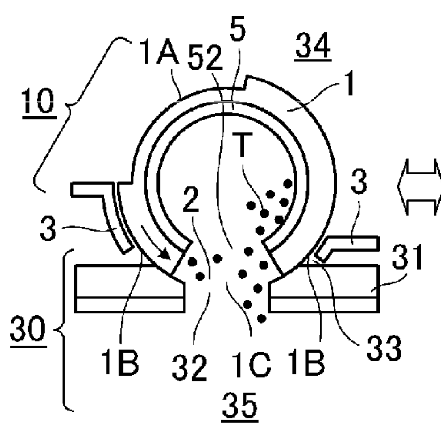
FIG. 1A SHUTTER OPEN STATE
