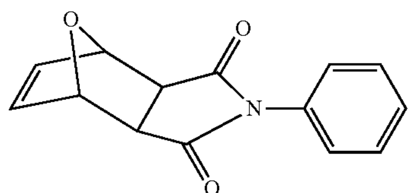
exo-7-oxanorbornene-N-phenyl- 5,6-dicarboxyanhydride
