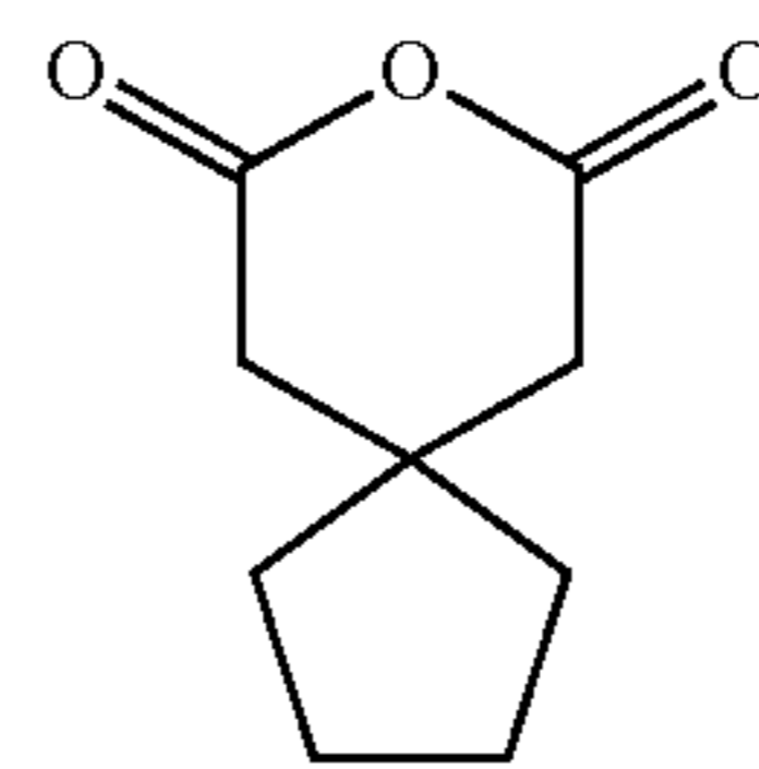
Tetramethyleneglutaric anhydride
