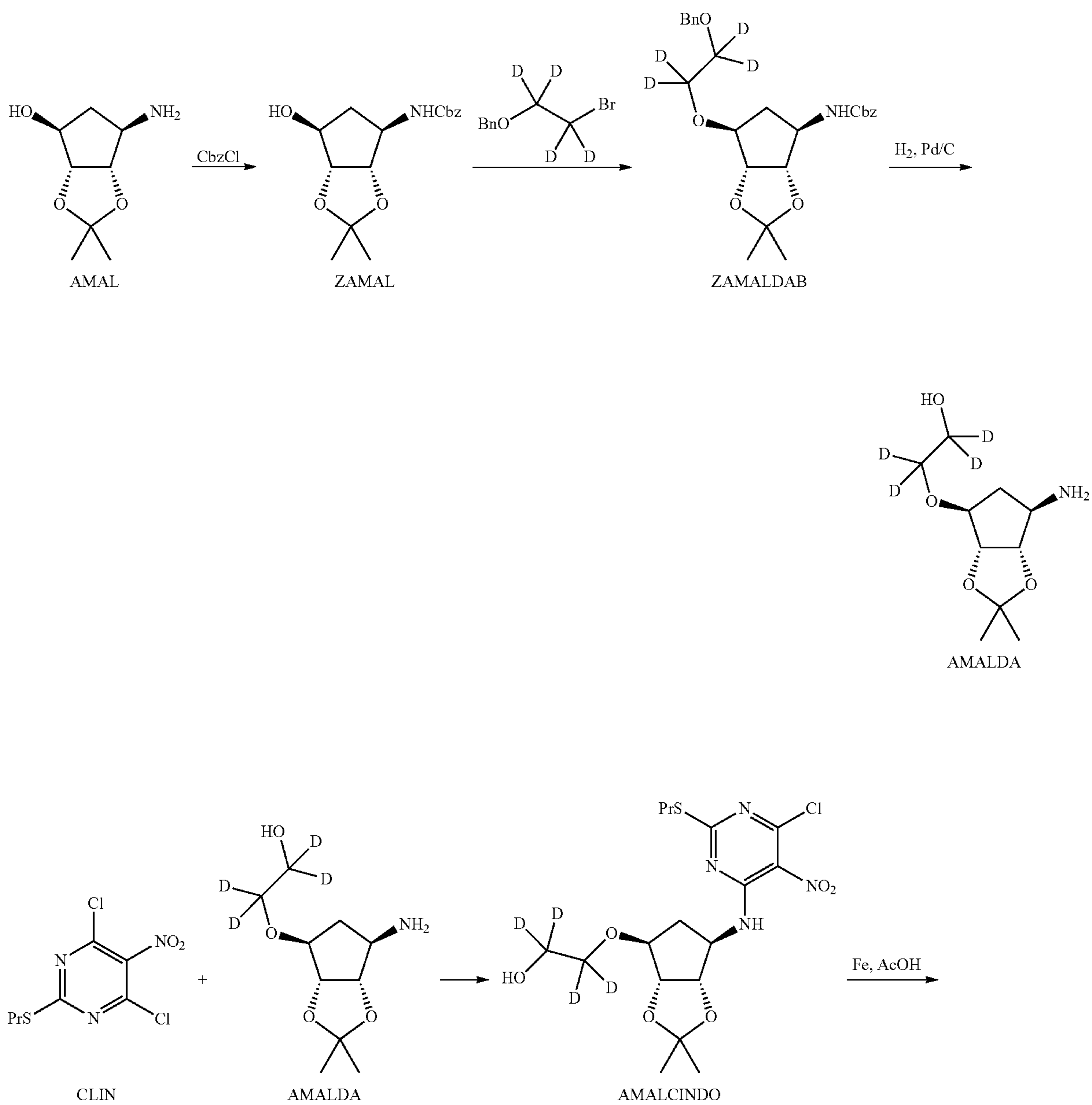
Scheme 6: Synthesis of ticagrelor with deuterated hydroxyethyl group (TCGD) as described in "deutero" patent WO 11/017108.
