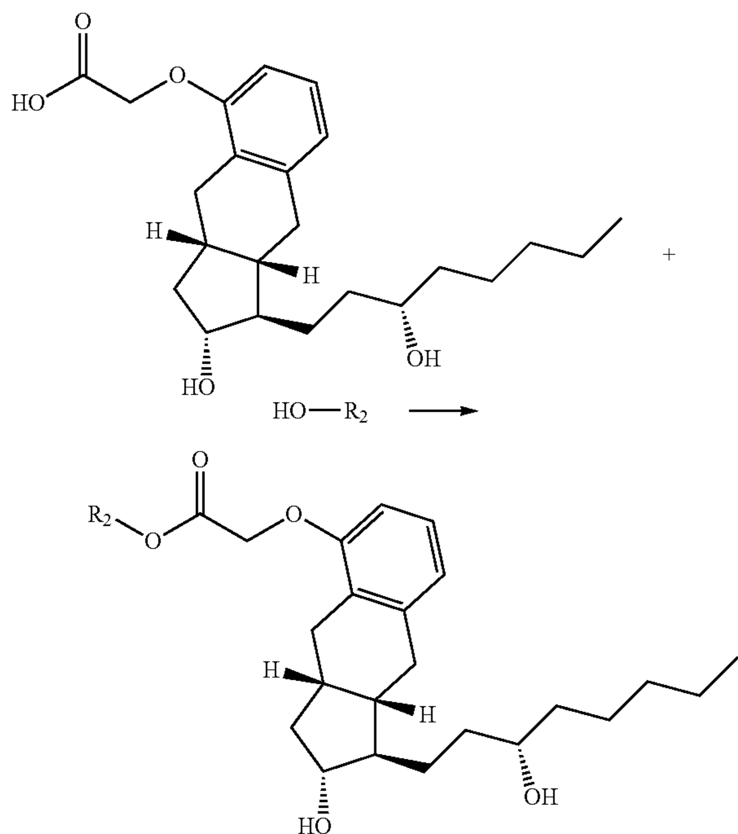
Scheme 1: Esterification Mechanism for alkyl ester-TR Compounds
