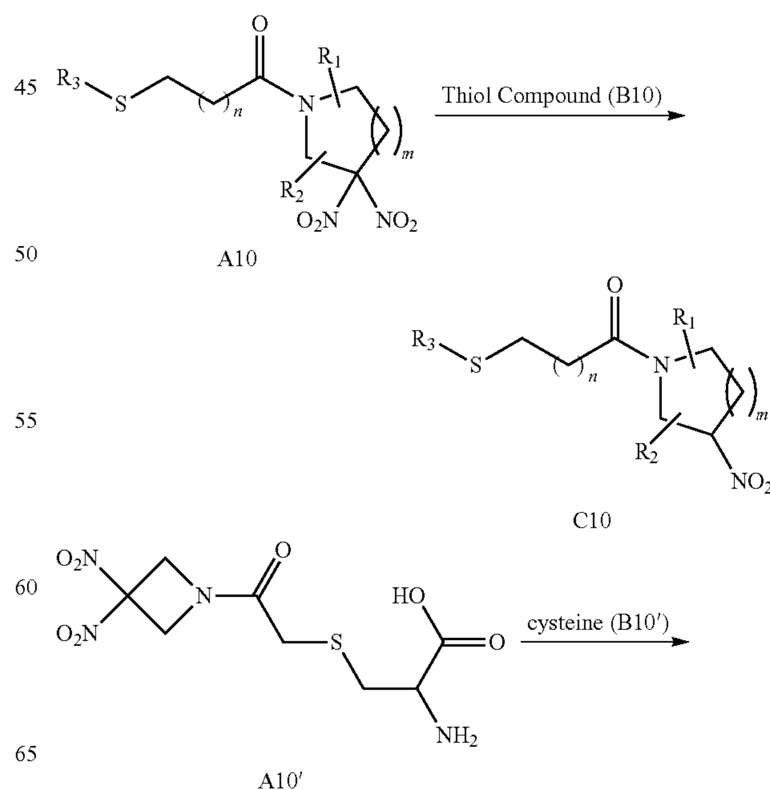
SCHEME 10
