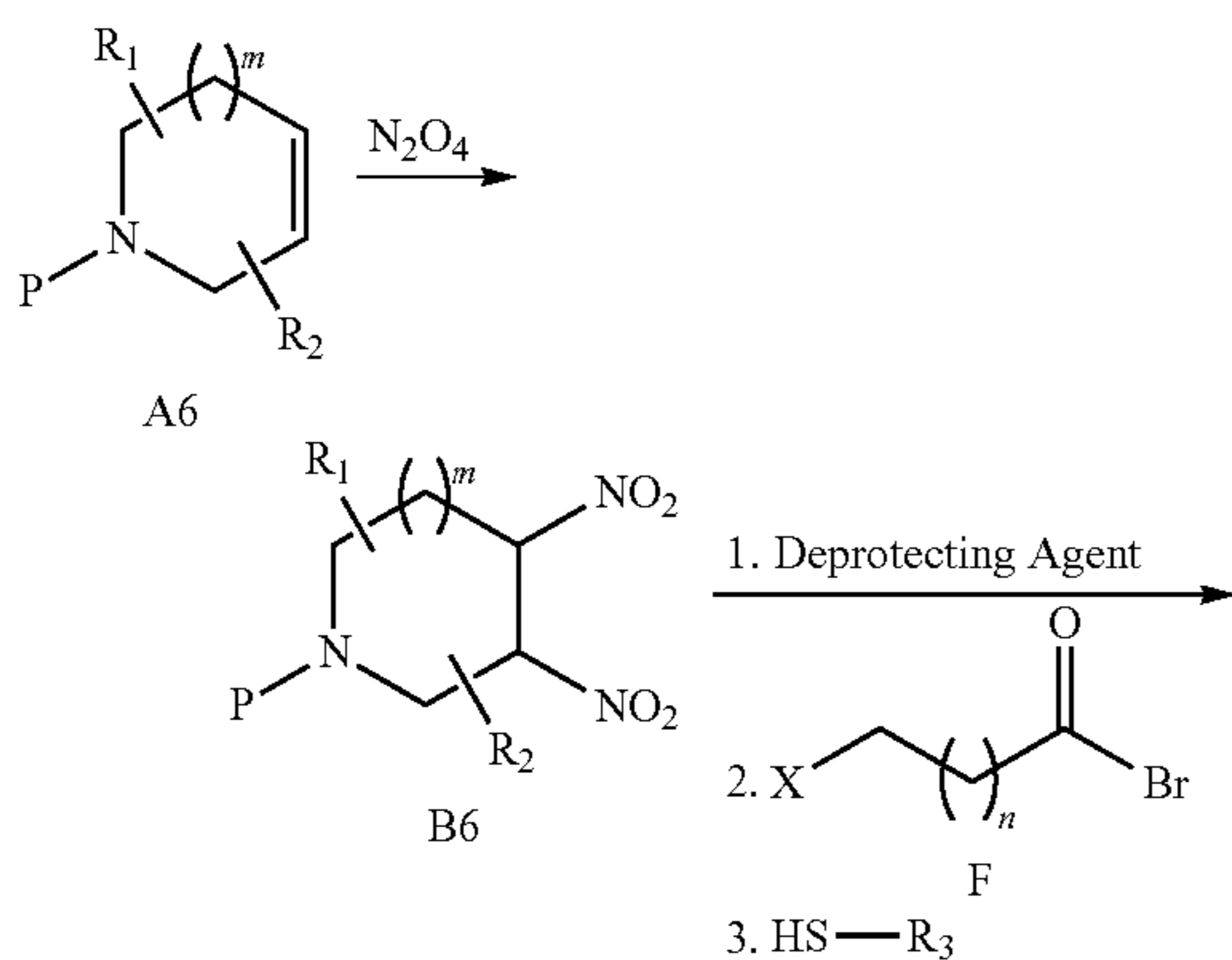
SCHEME 6
