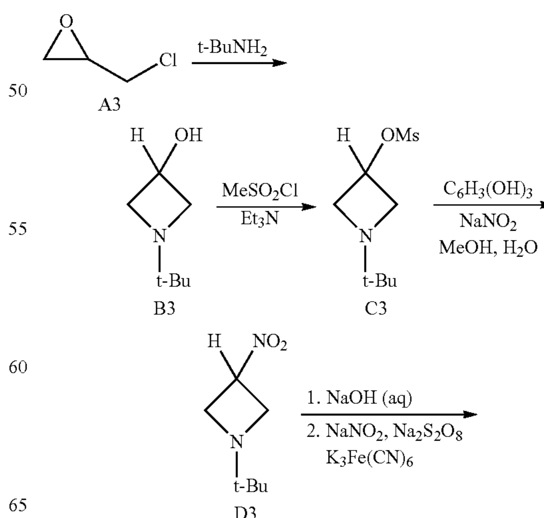
SCHEME 3
