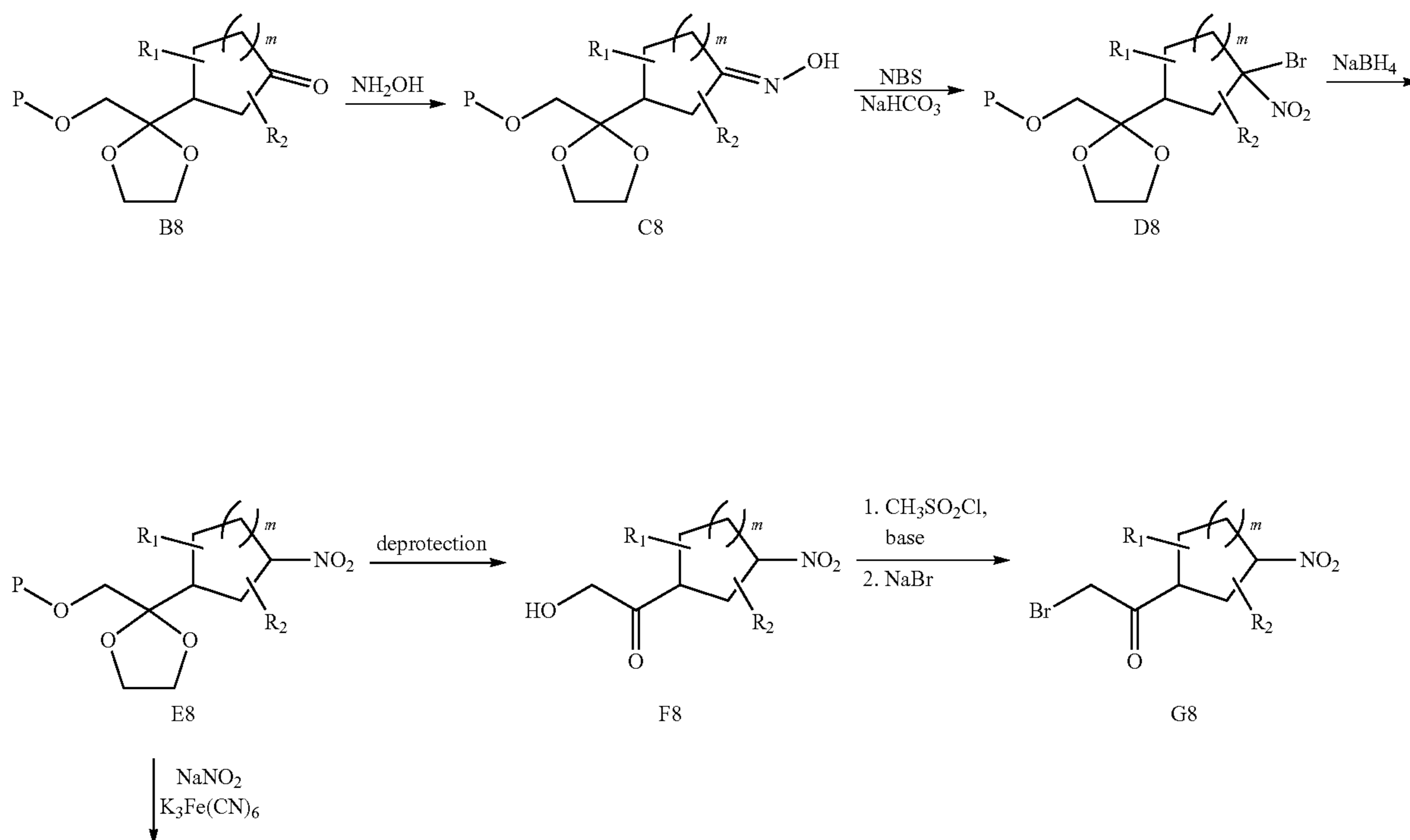
SCHEME 8
