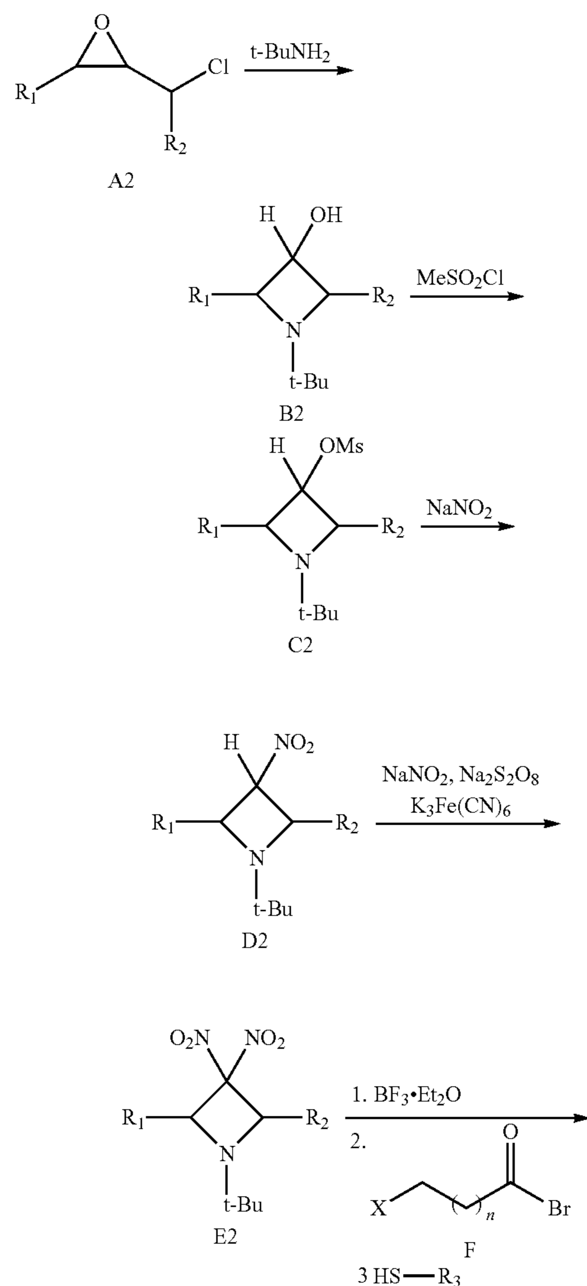
SCHEME 2
