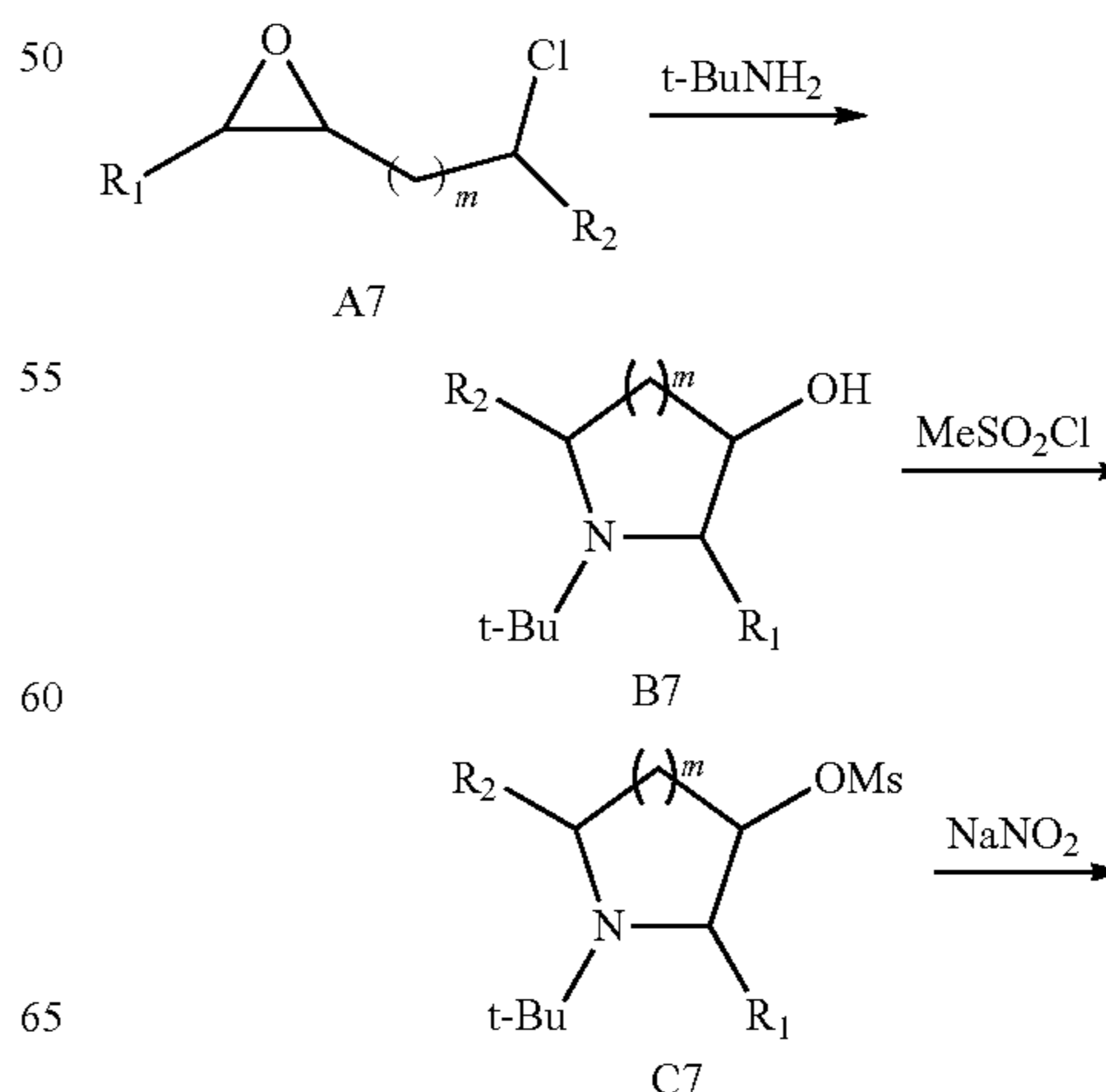
SCHEME 7
