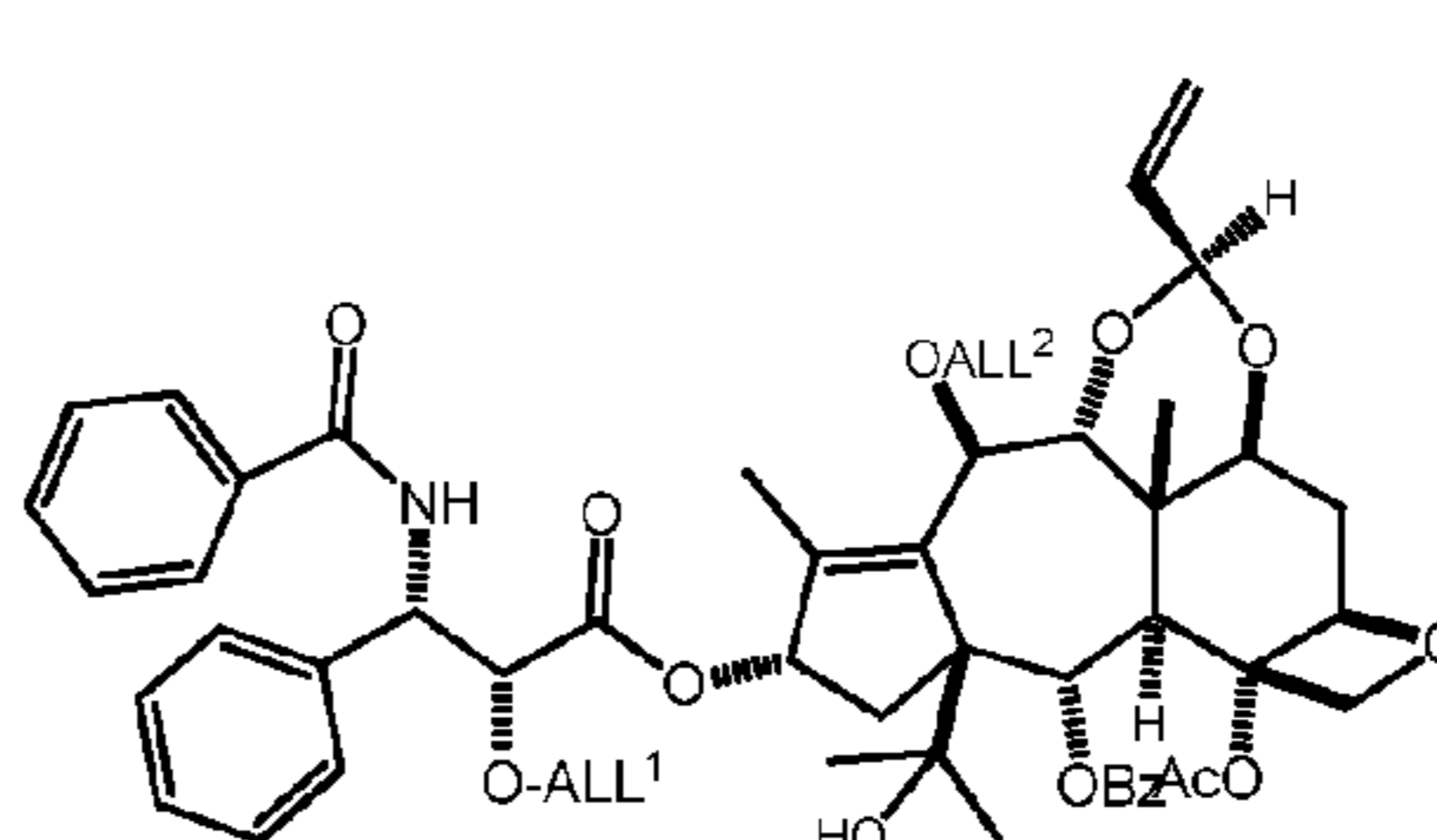
ALLMC of a 10-beta abeo-taxane analog (19h)
