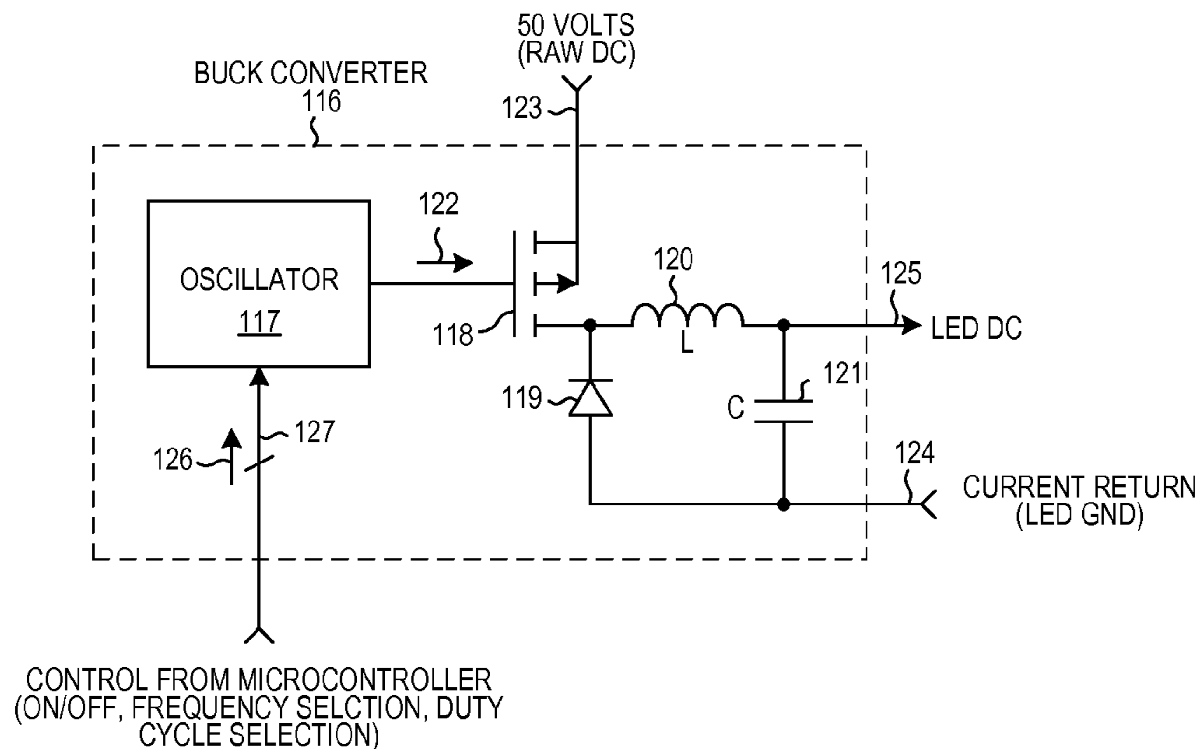
BUCK CONVERTER
