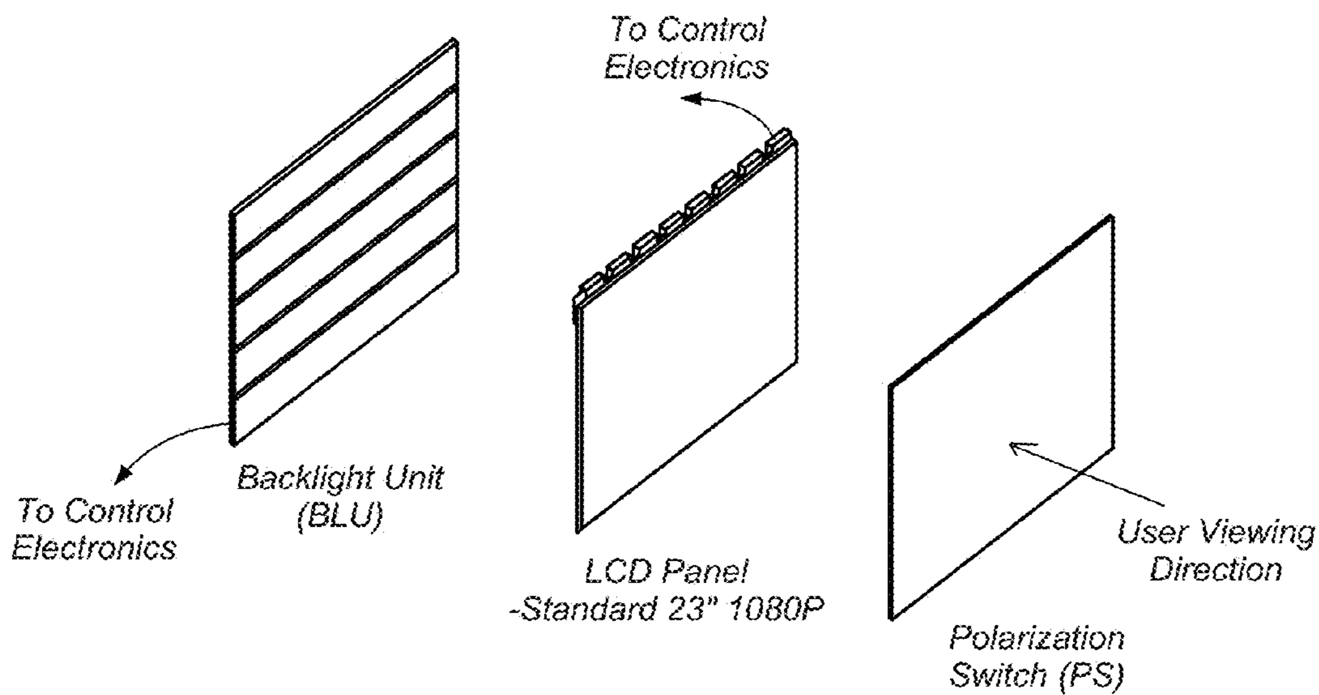
FIG. 2 (PRIOR ART)
