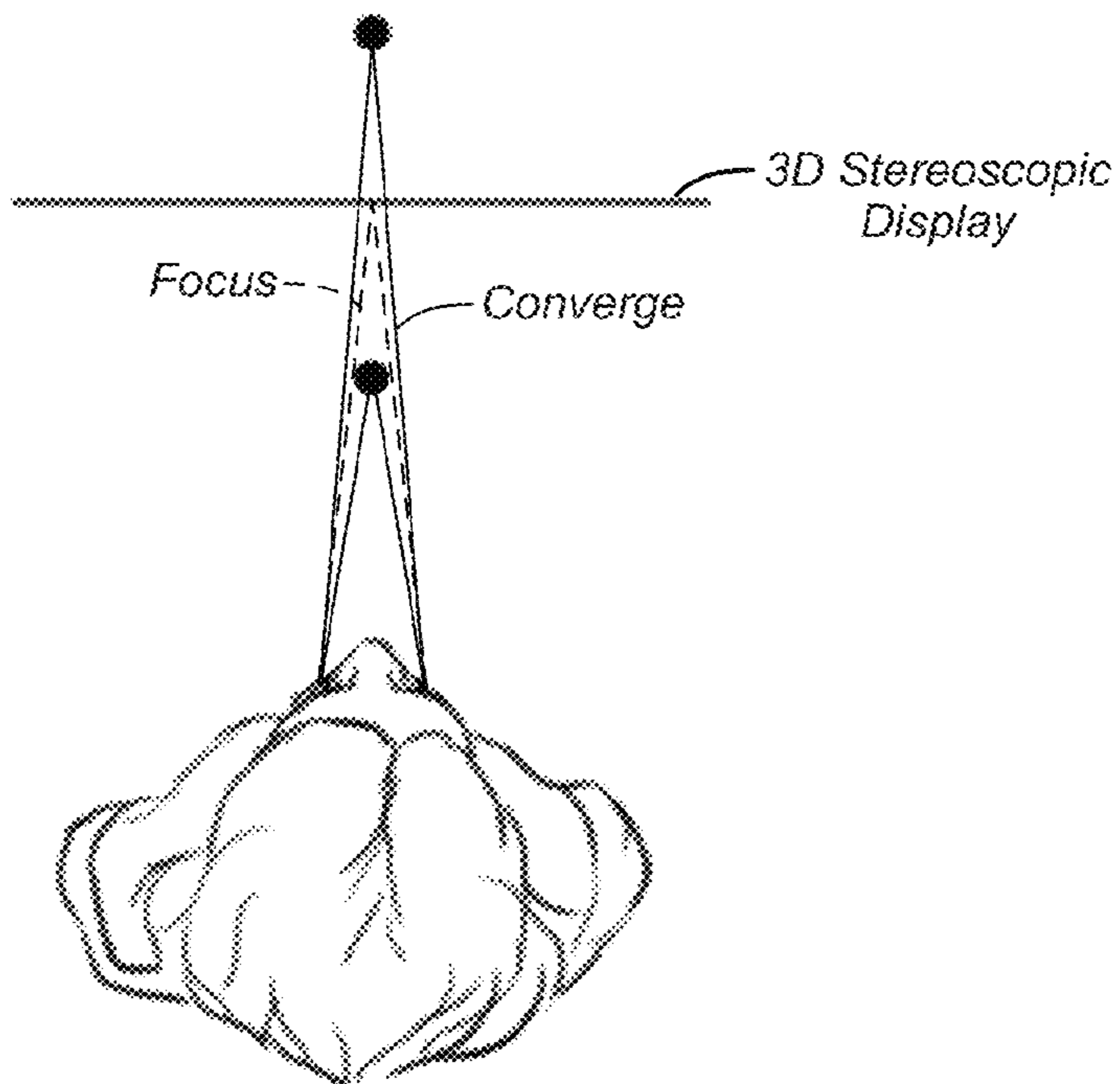
FIG. 5 (PRIOR ART)
