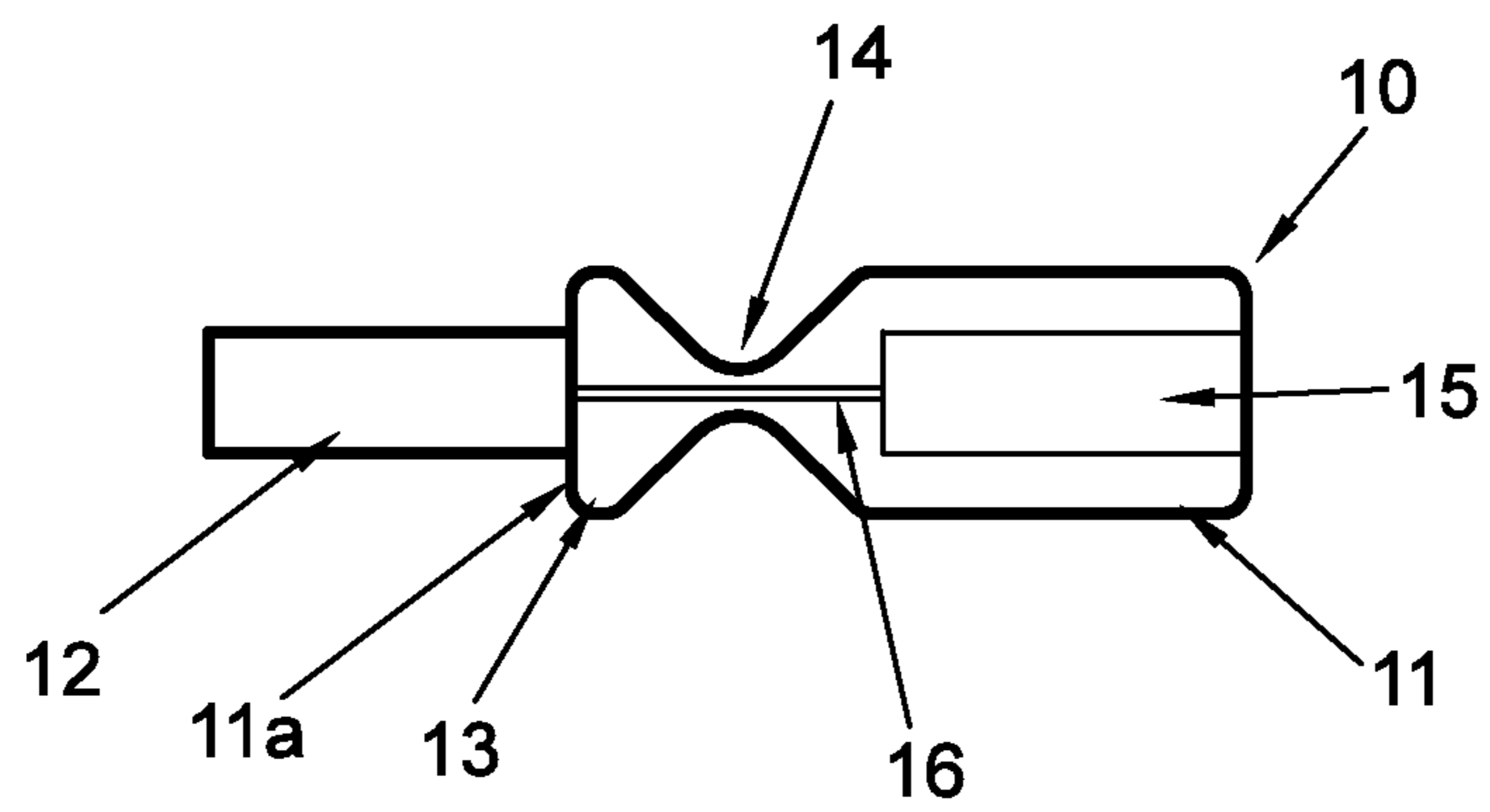
SECTION B-B (Fig 1)
