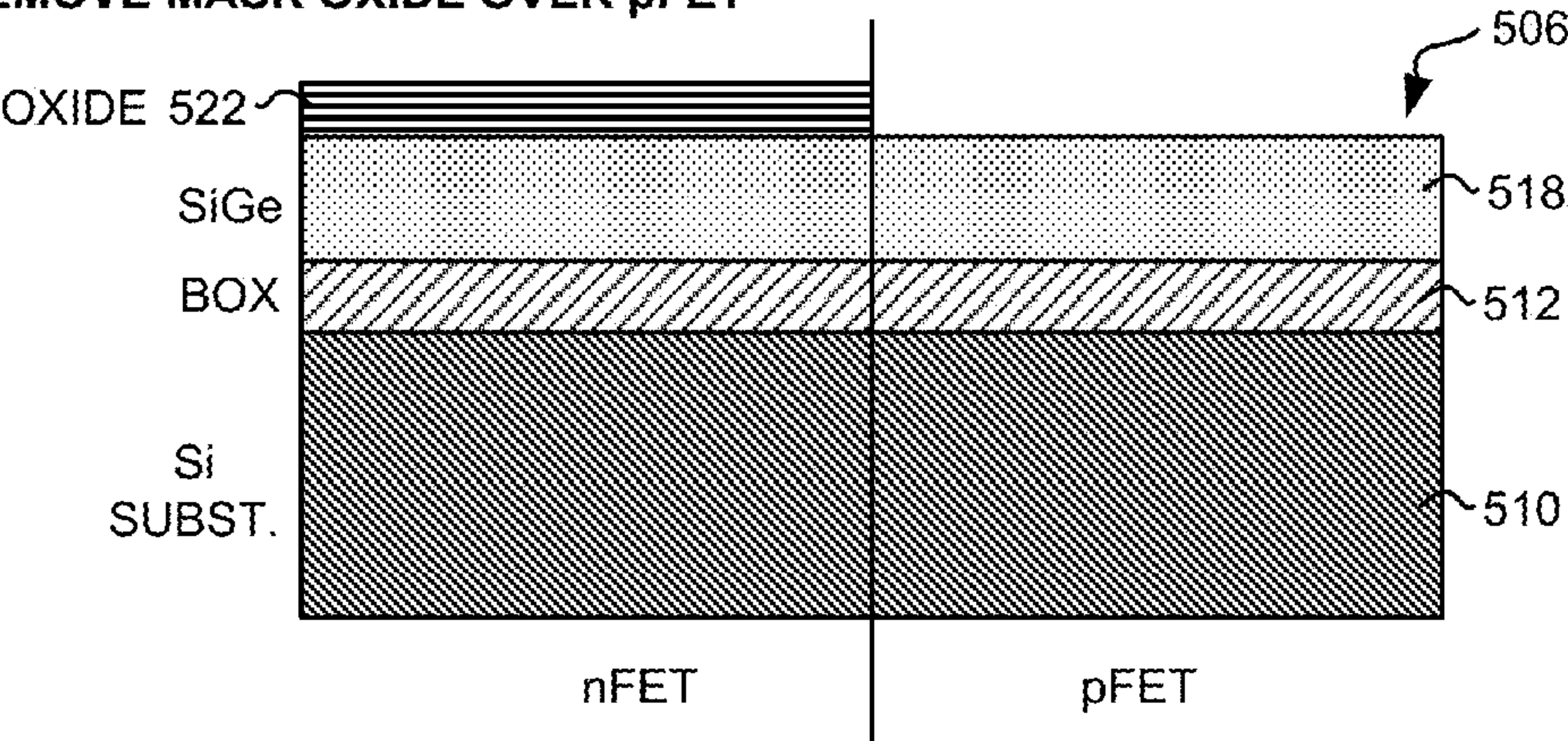
REMOVE MASK OXIDE OVER pFET
