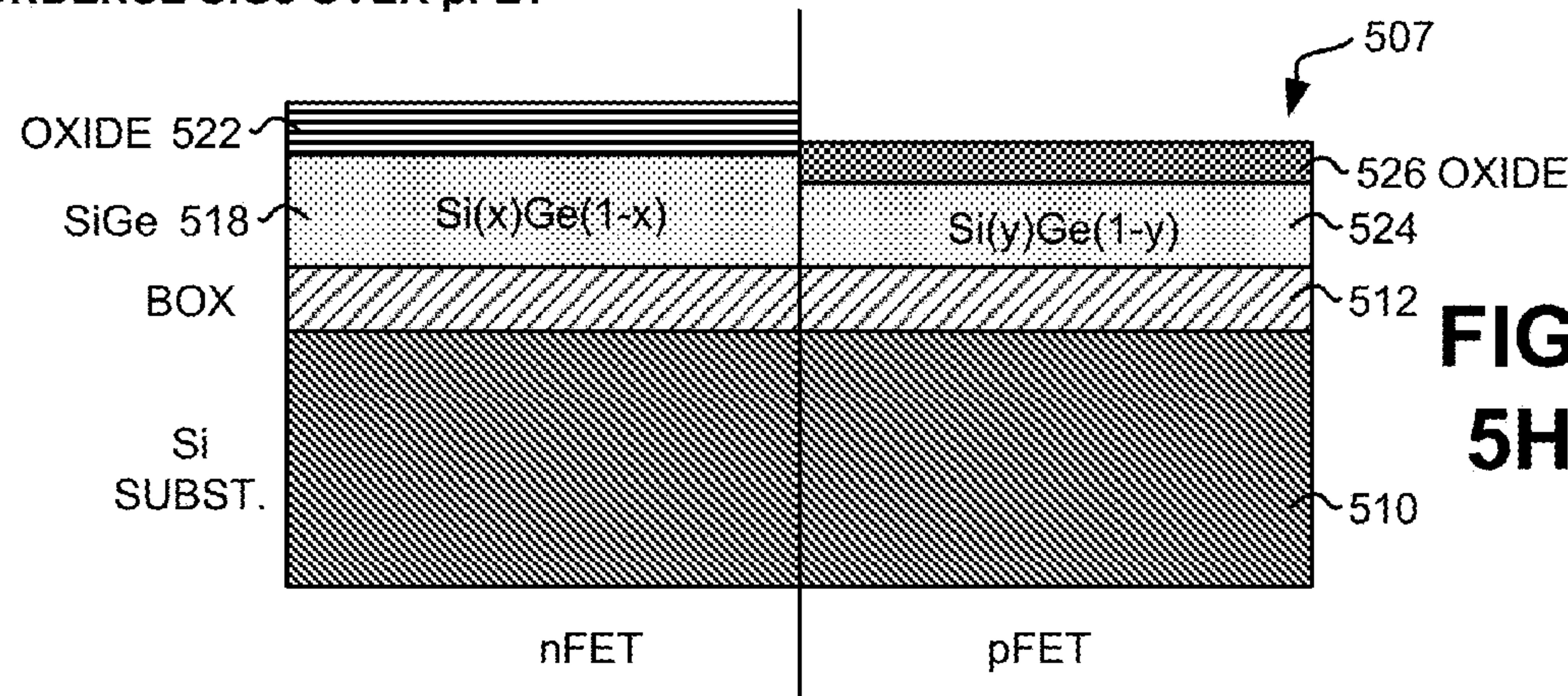
CONDENSE SiGe OVER pFET
