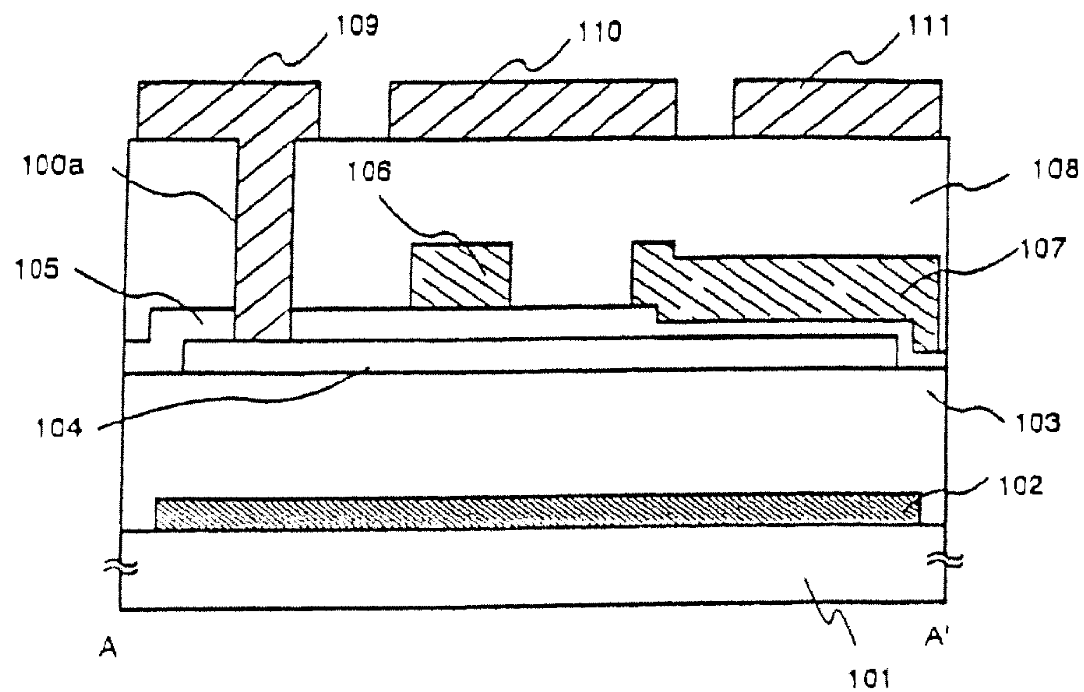
Fig. 3A A-A' cross sectional view
