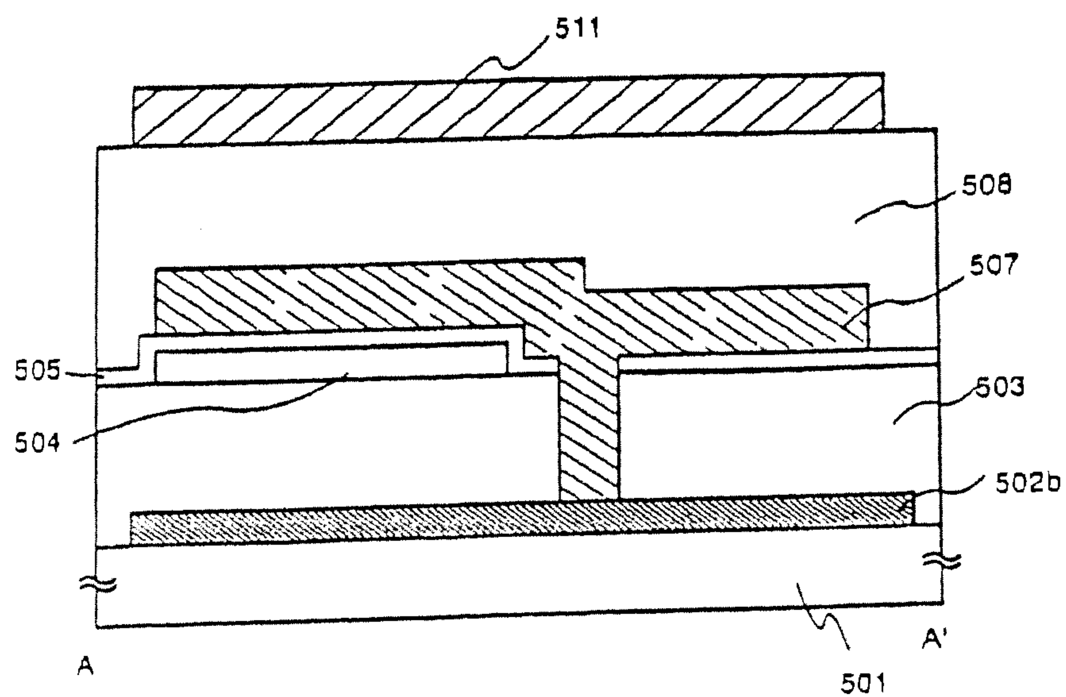
Fig. 15A A-A' Cross sectional view
