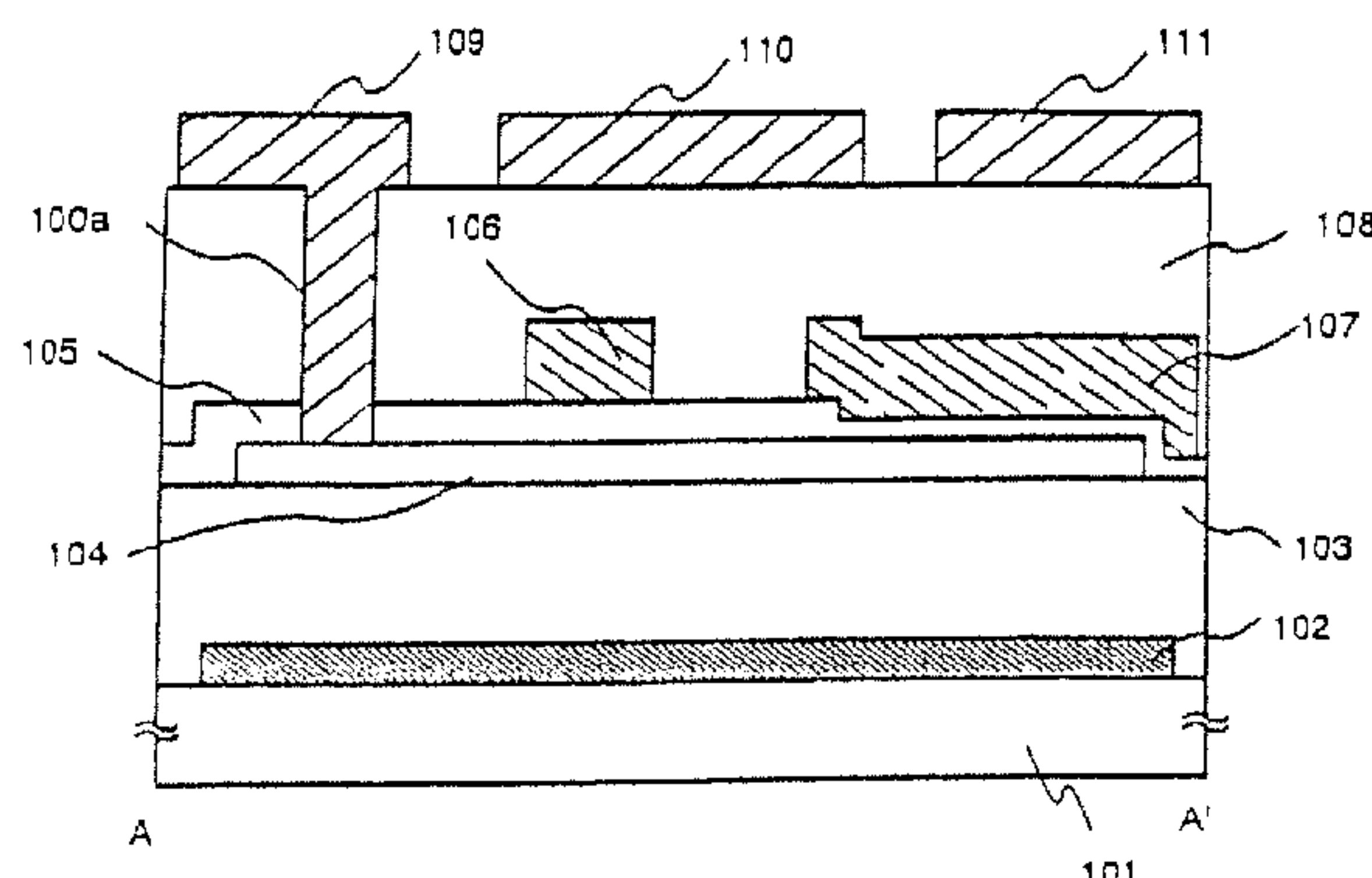
A-A' cross sectional view
