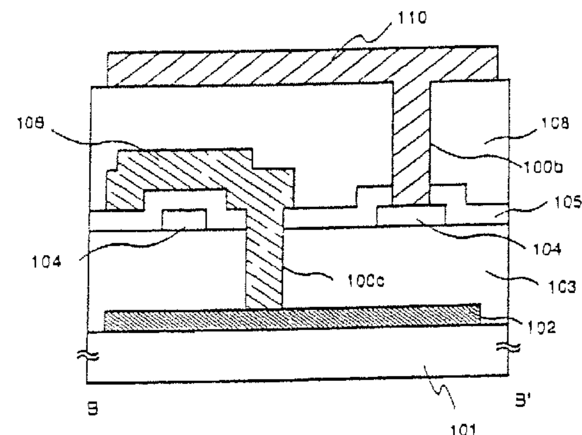
B-B' cross sectional view
