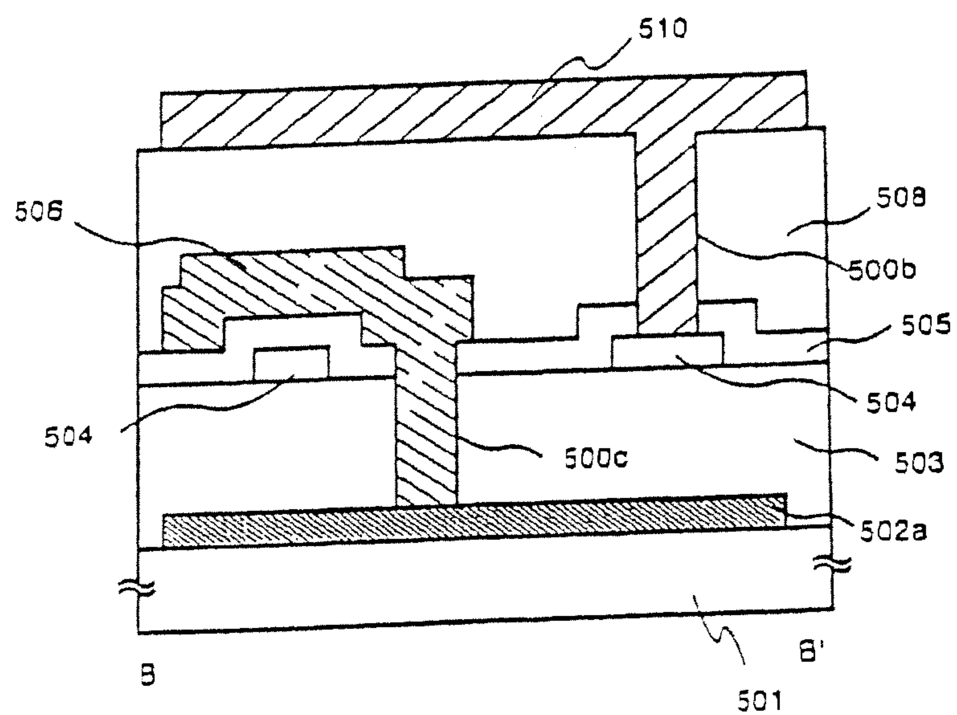
Fig. 15B B-B' Cross sectional view
