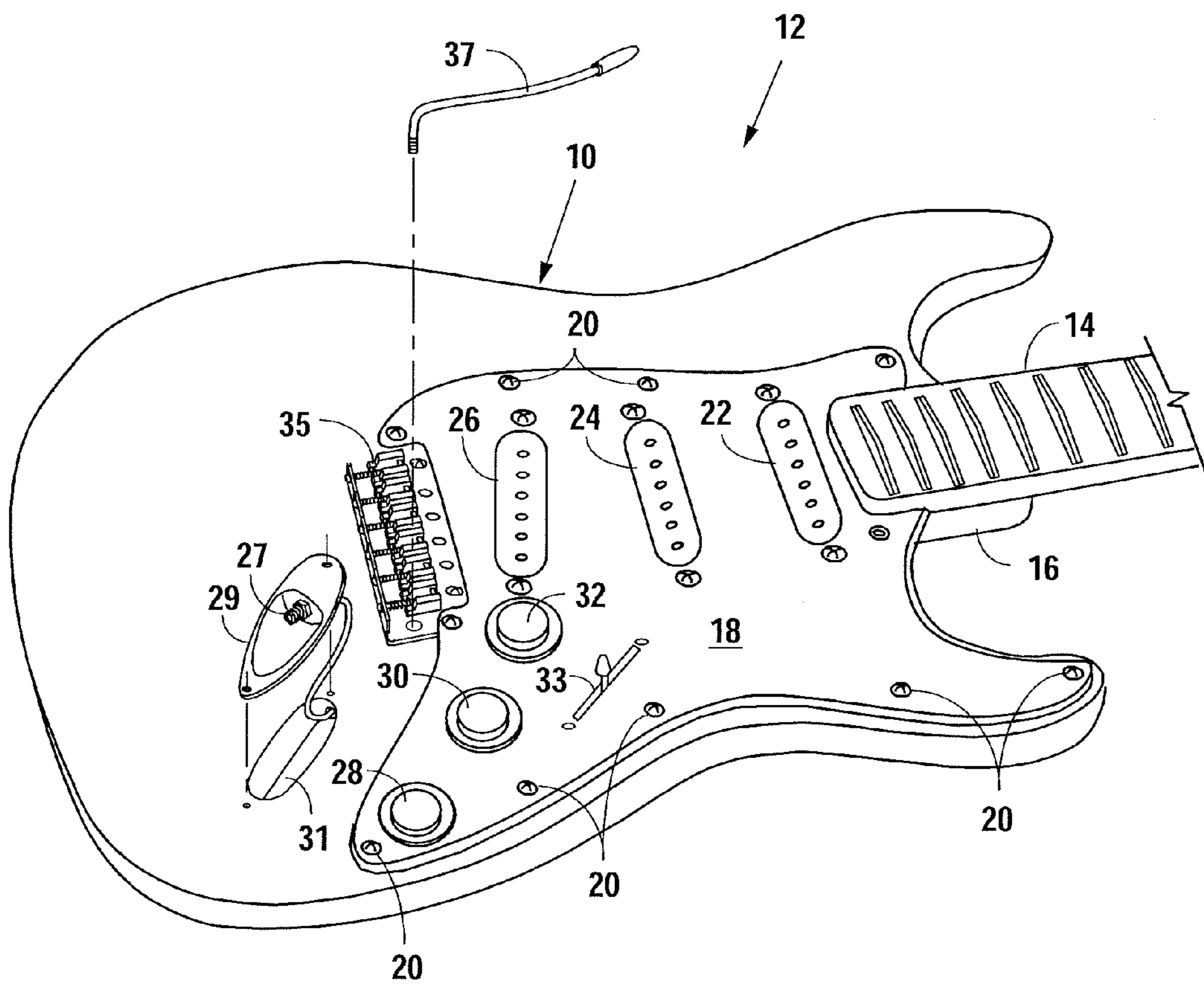
Fig. 1 PRIOR ART
