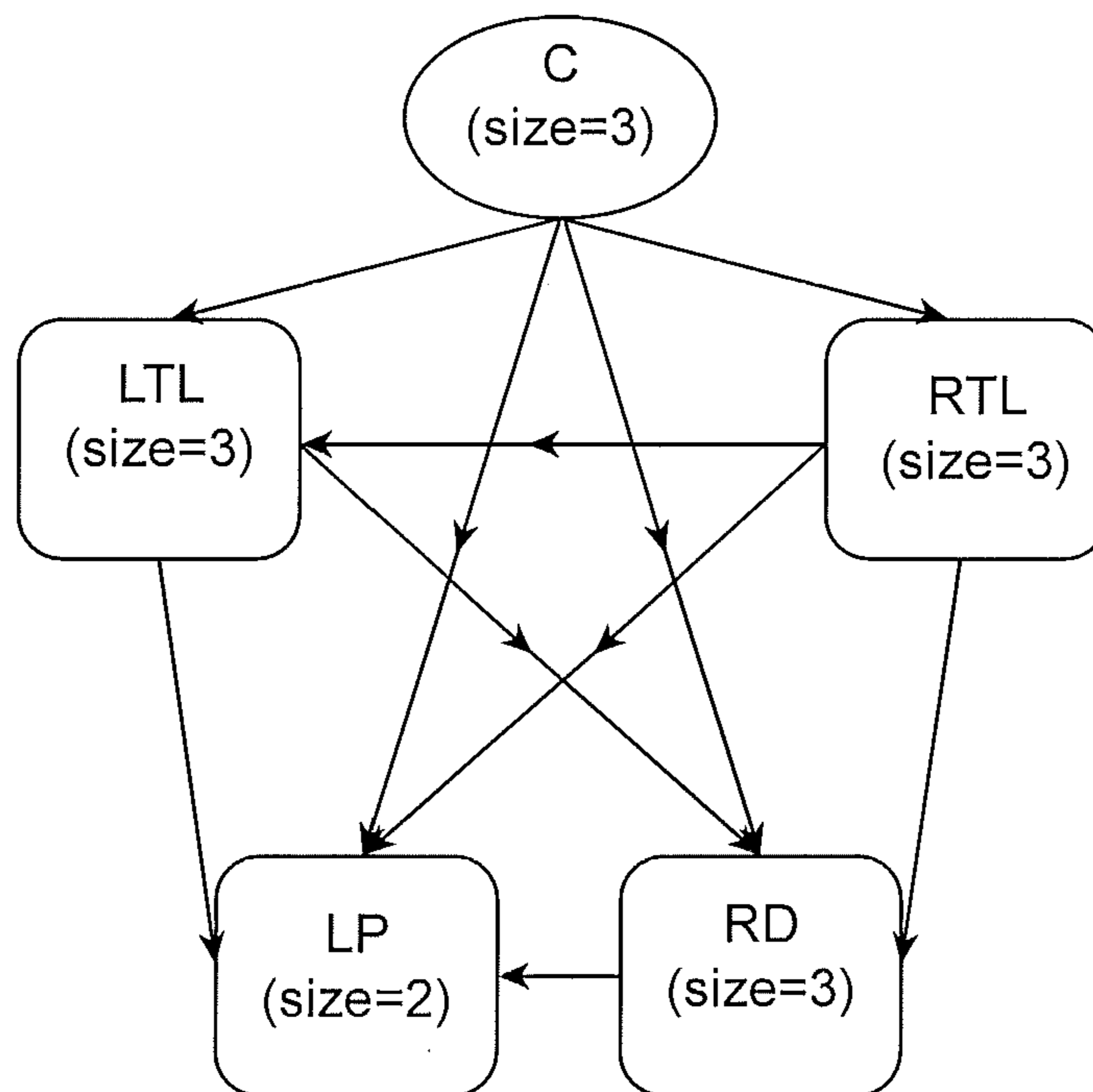
K2 generated structure
