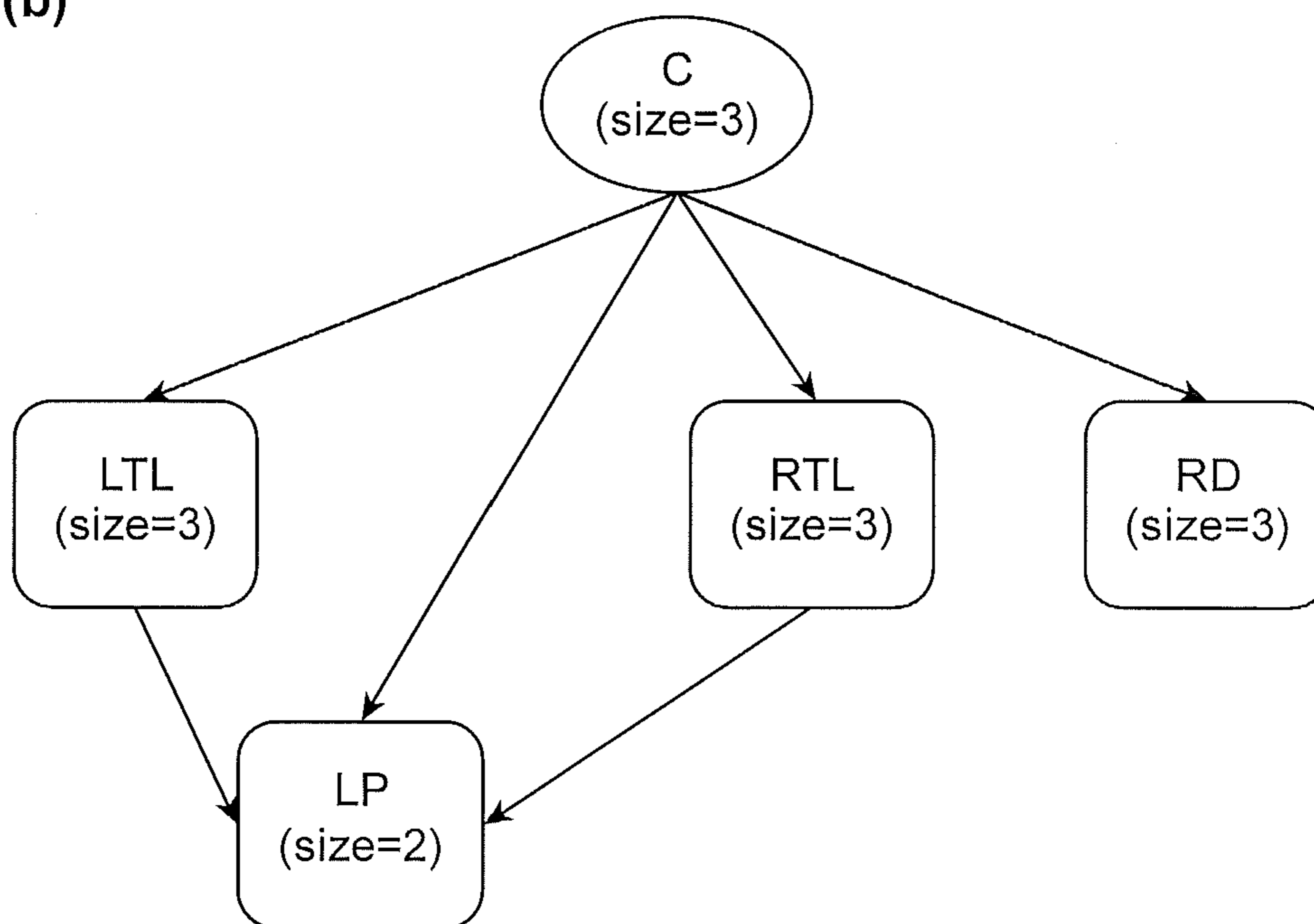
Manually structured Bayesian network
