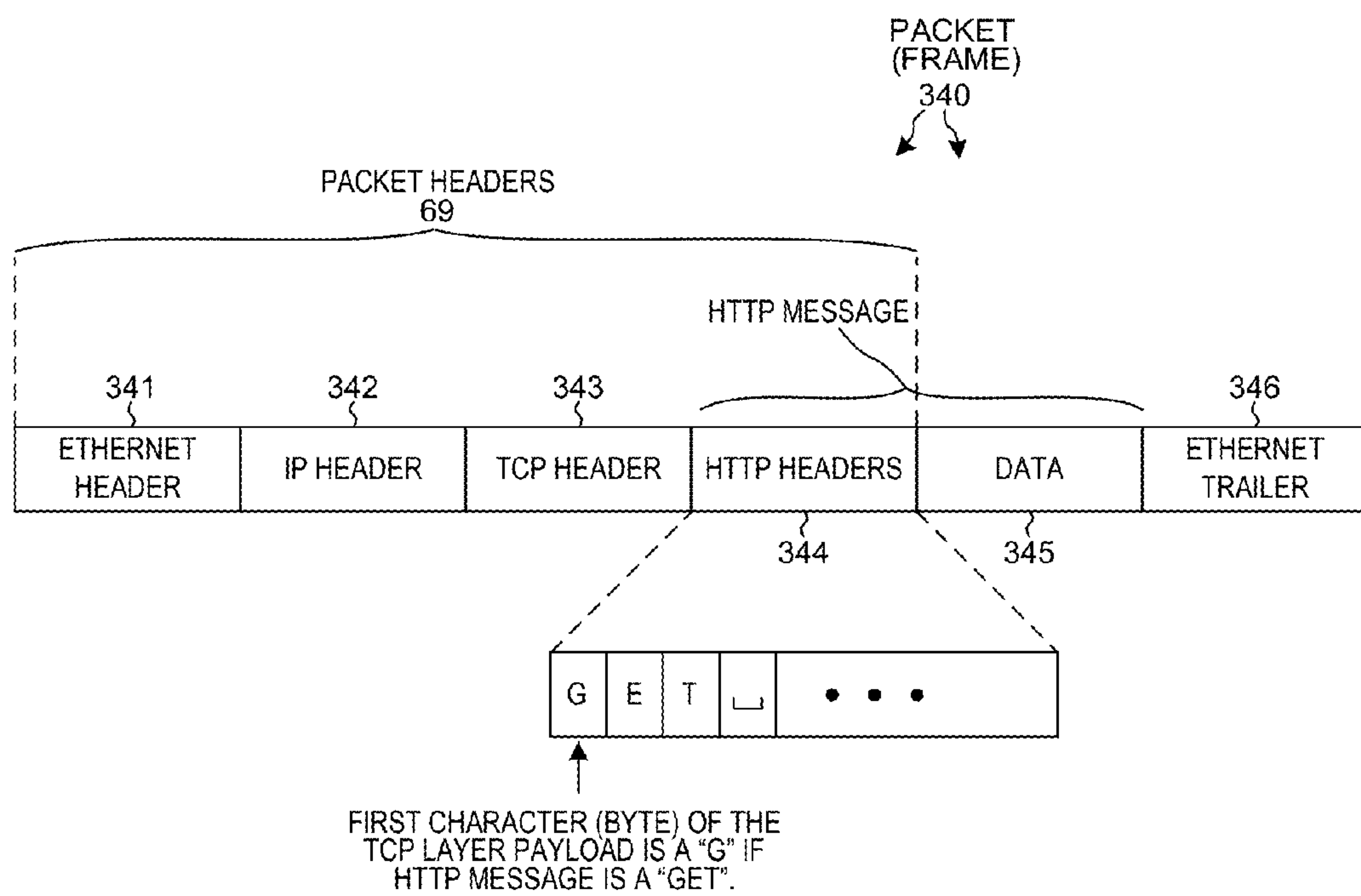
ETHERNET FRAME (PACKET) THAT CONTAINS A HTTP GET MESSAGE FIG. 27
