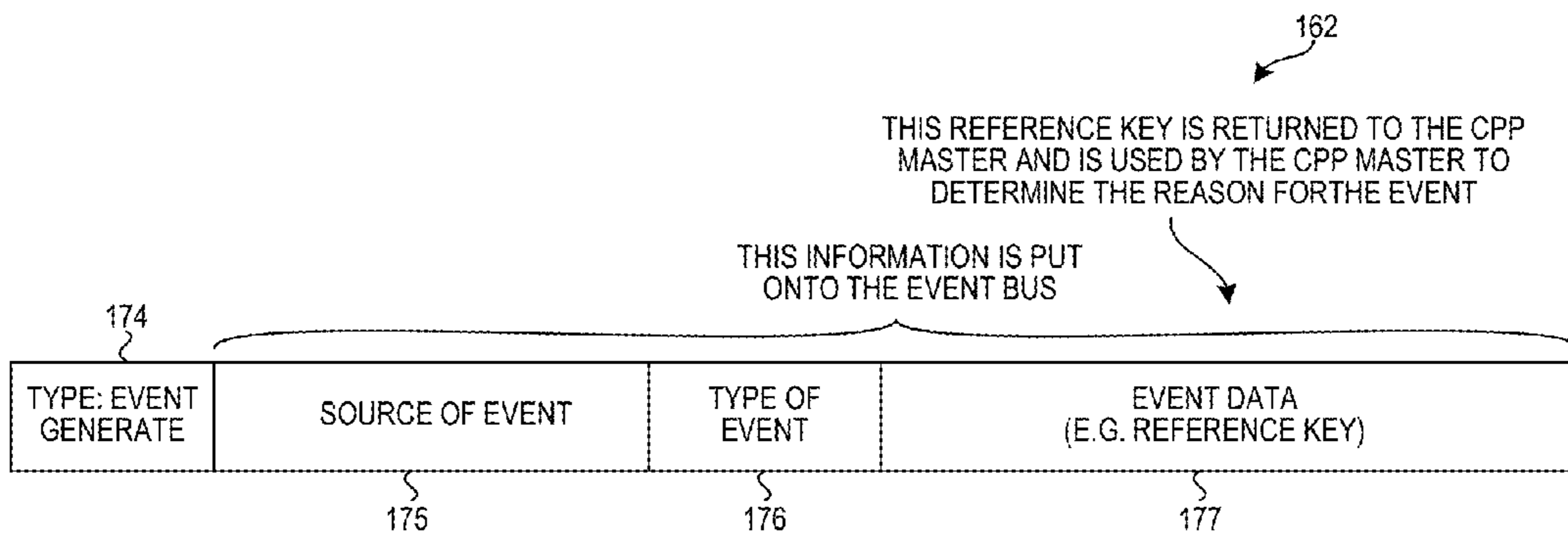
NFA ENGINE EVENT GENERATE COMMAND FIG. 11
