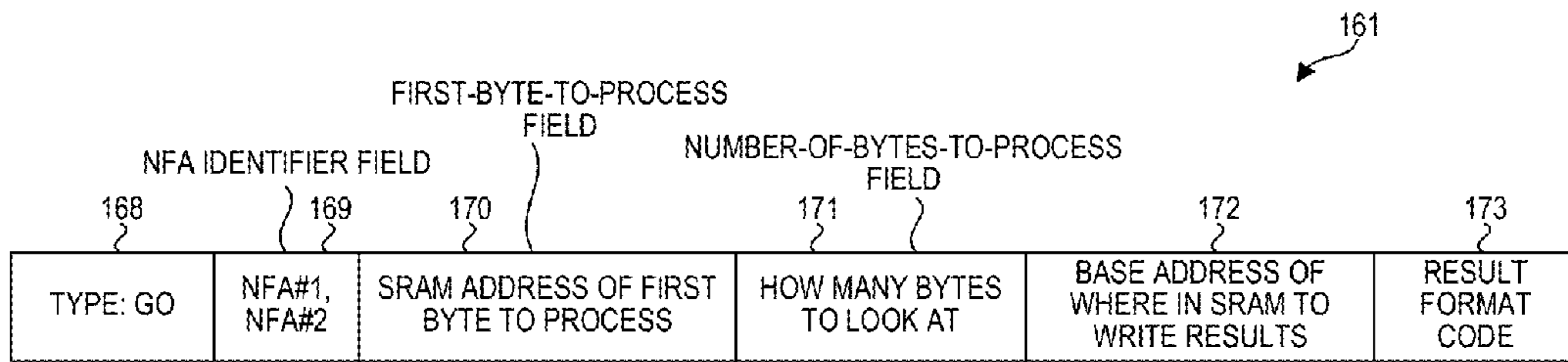
NFA ENGINE GO COMMAND FIG. 10
