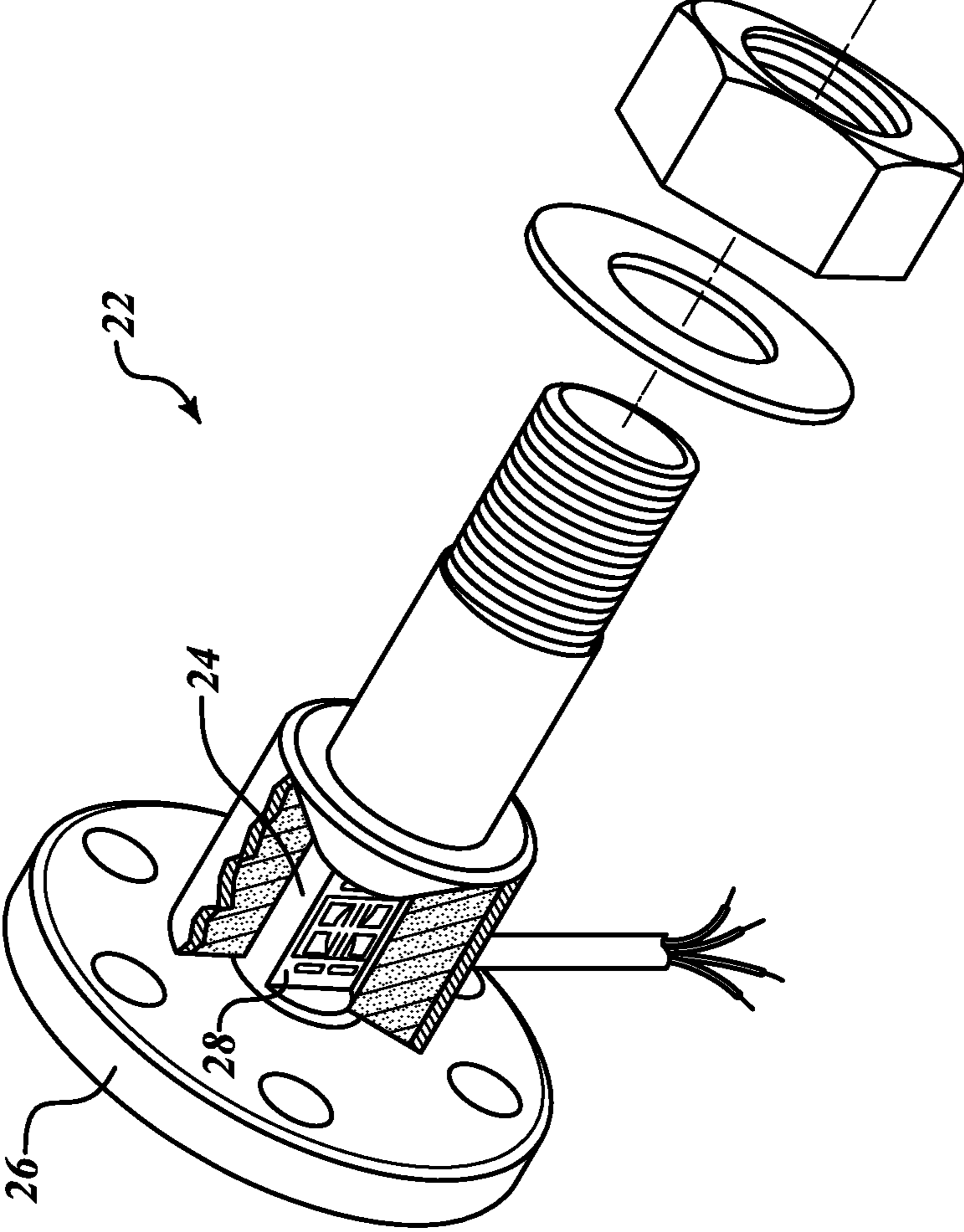
FIG. 3 (Prior Art)
