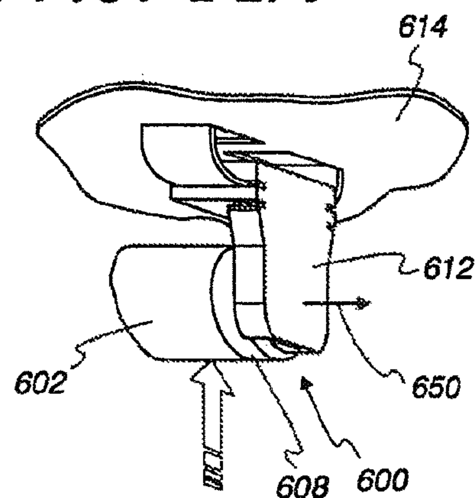
Fig. 59 Prior Art
