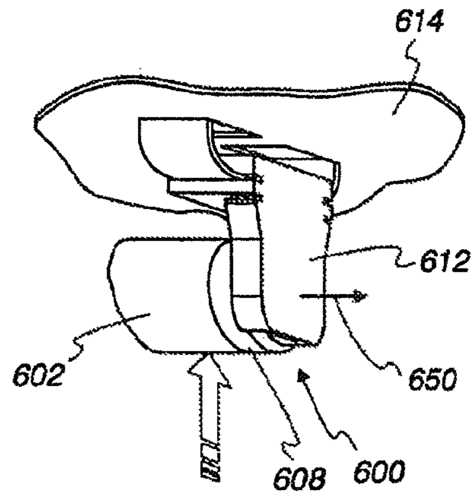
Fig. 59 Prior Art
