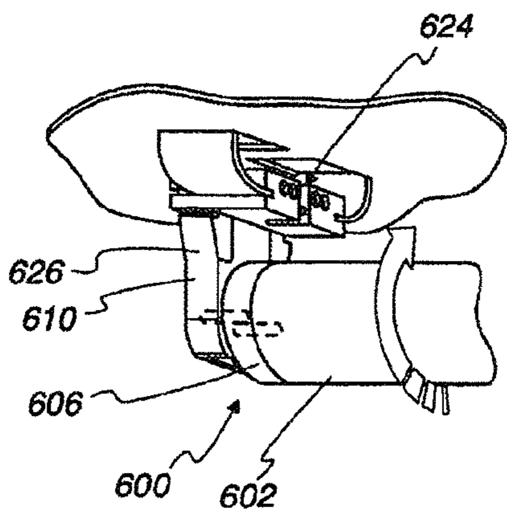
Fig. 60 Prior Art
