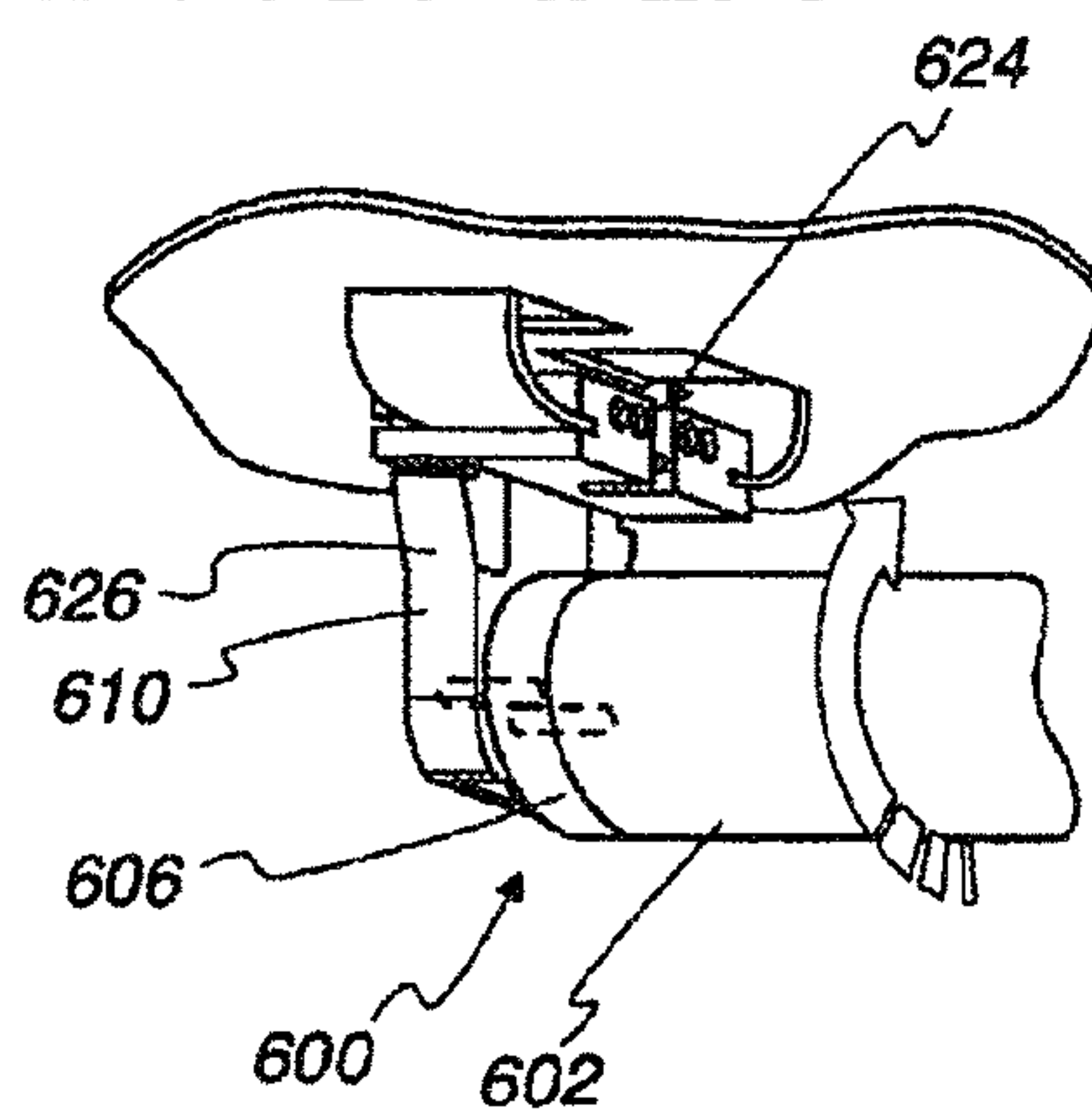
Fig. 60 Prior Art
