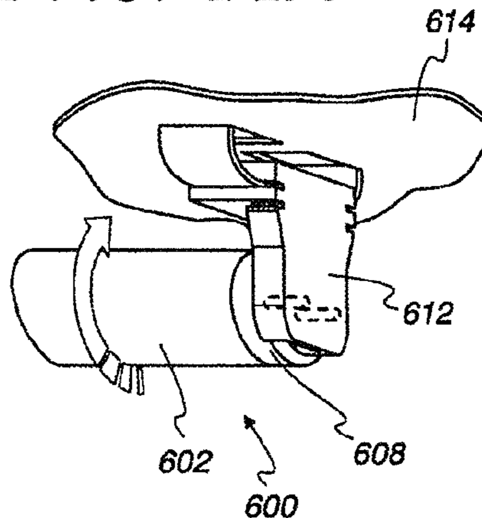
Fig. 61 Prior Art
