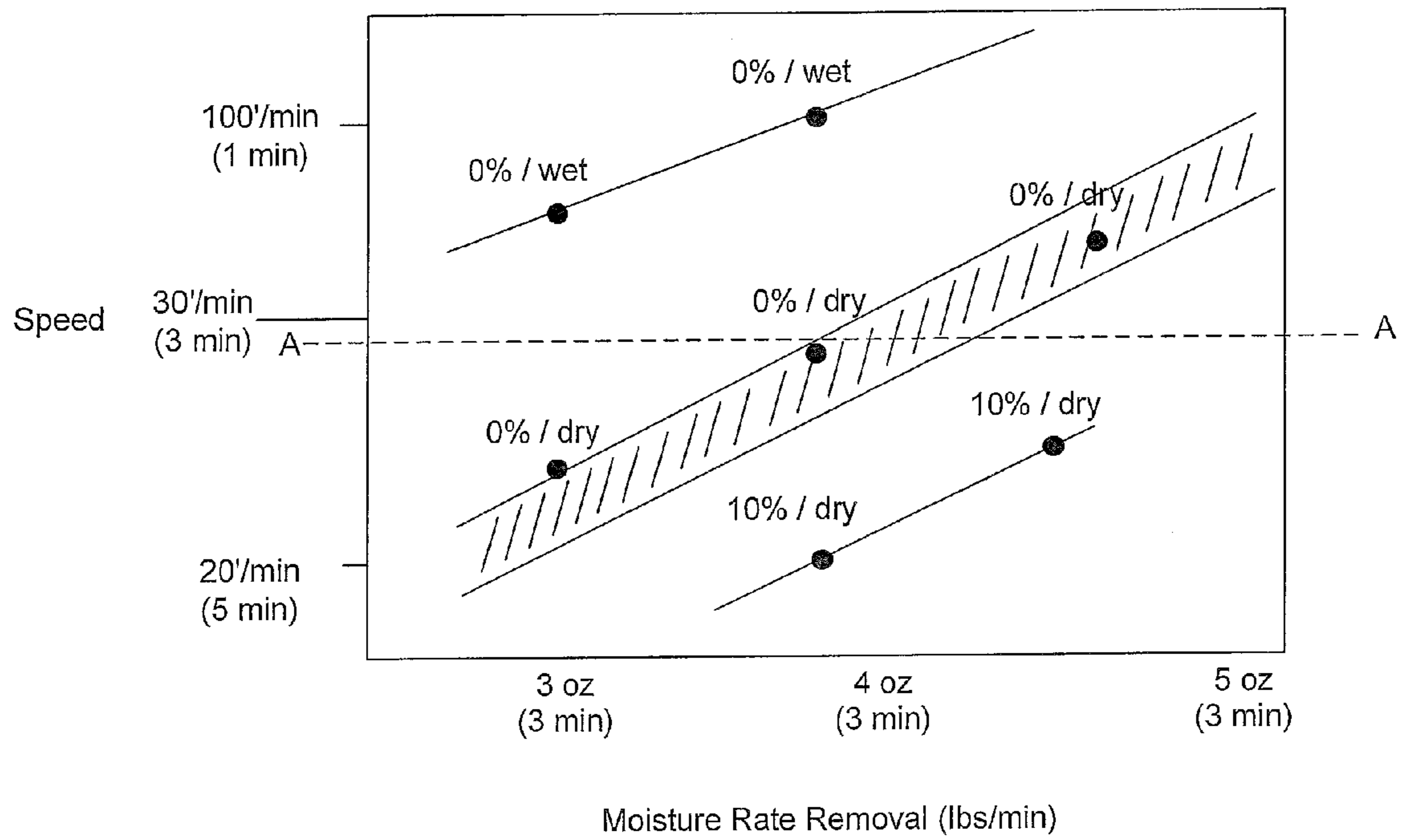
FIG. 5 (Drying / % Rebound)
