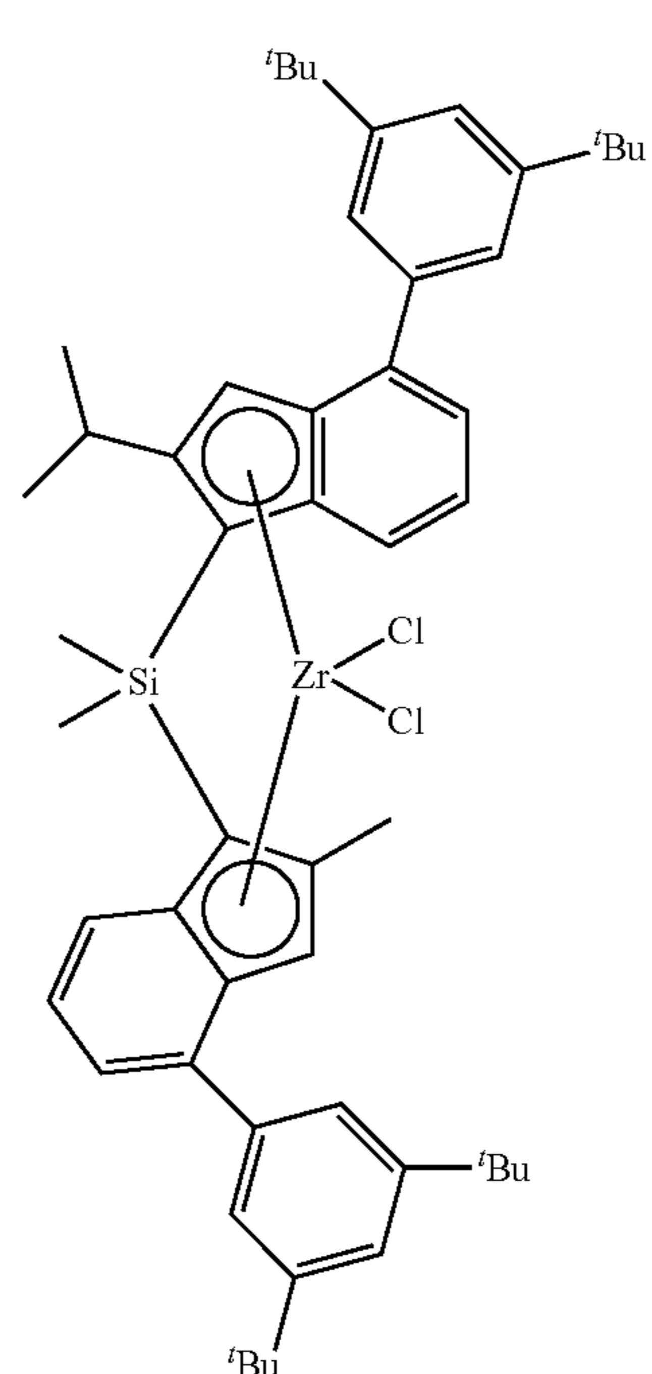
MTC-5 rac/meso = 10/1
