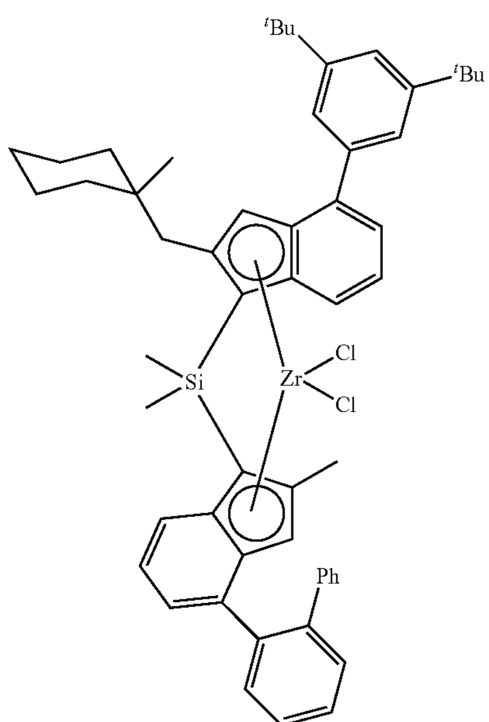
MTC-3 rac/meso = 1.3/1
