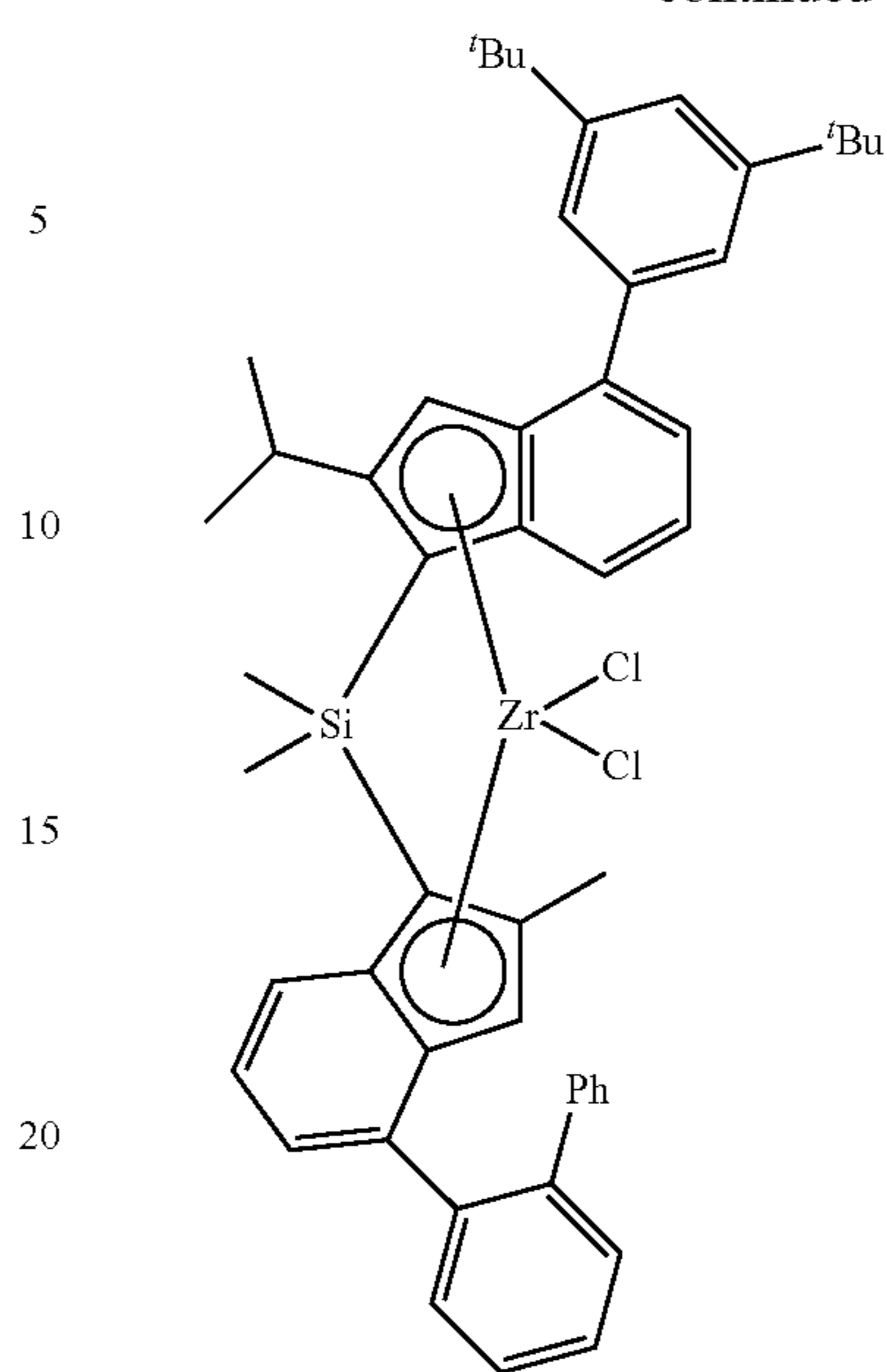
MTC-4 rac/meso > 50:1
