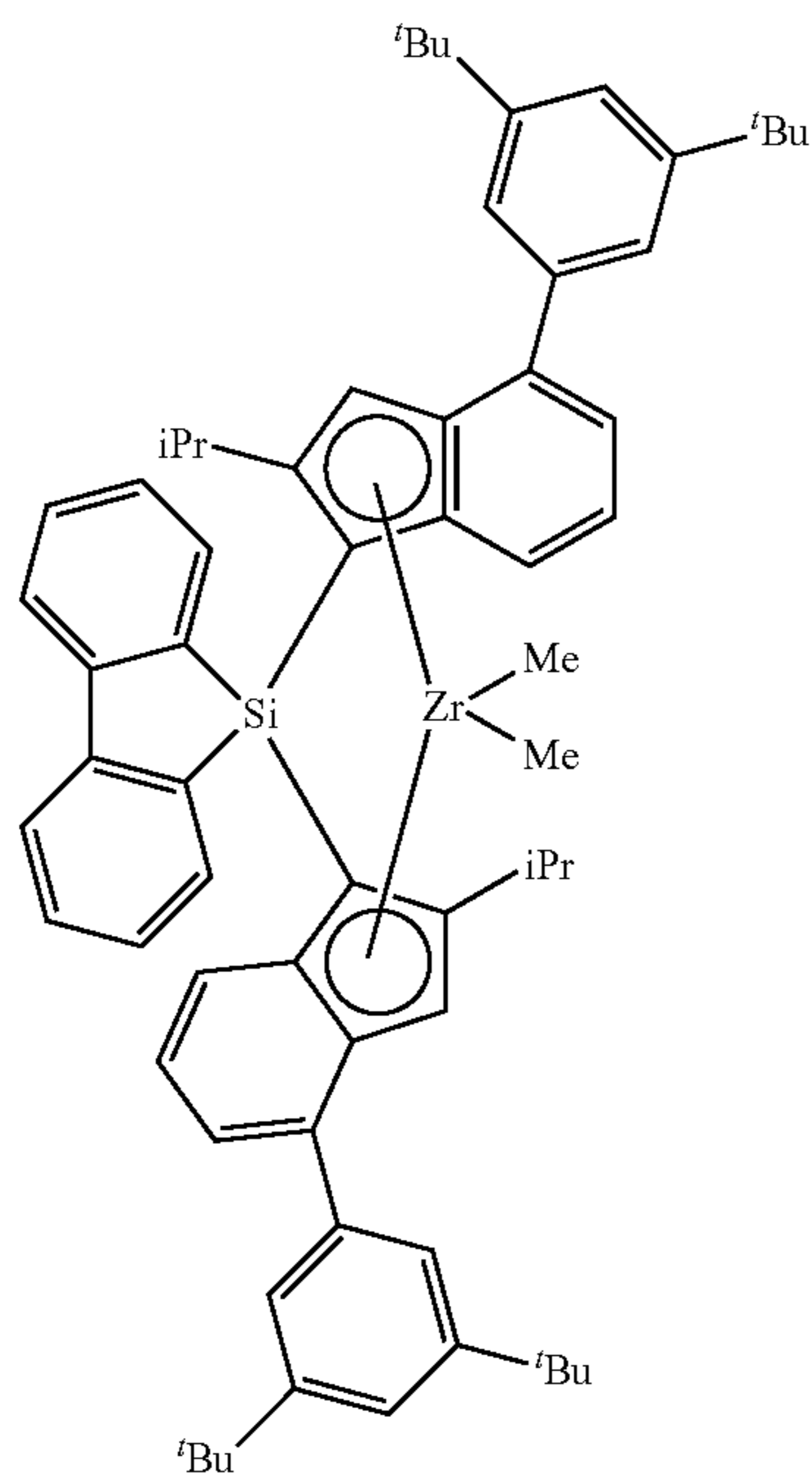
MTC-B rac/meso > 20:1
