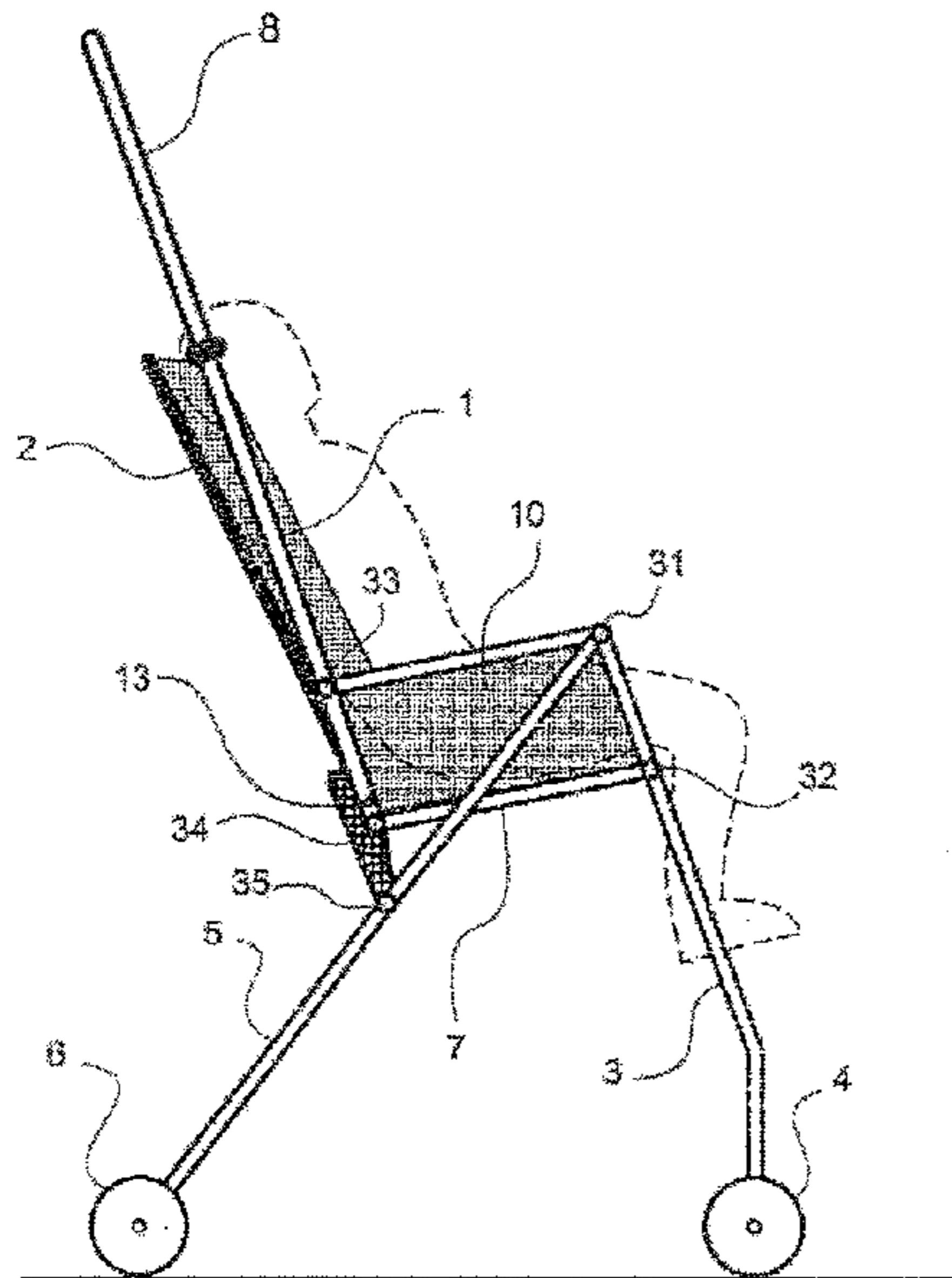
Figure 1 (Prior art)
