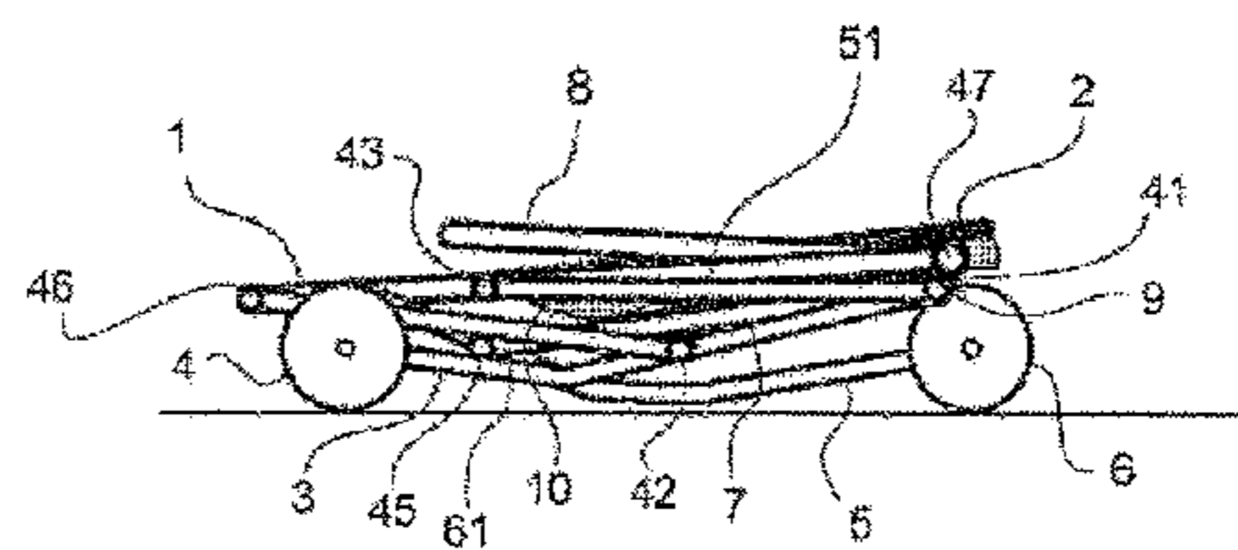
Figure 2C (Prior art)
