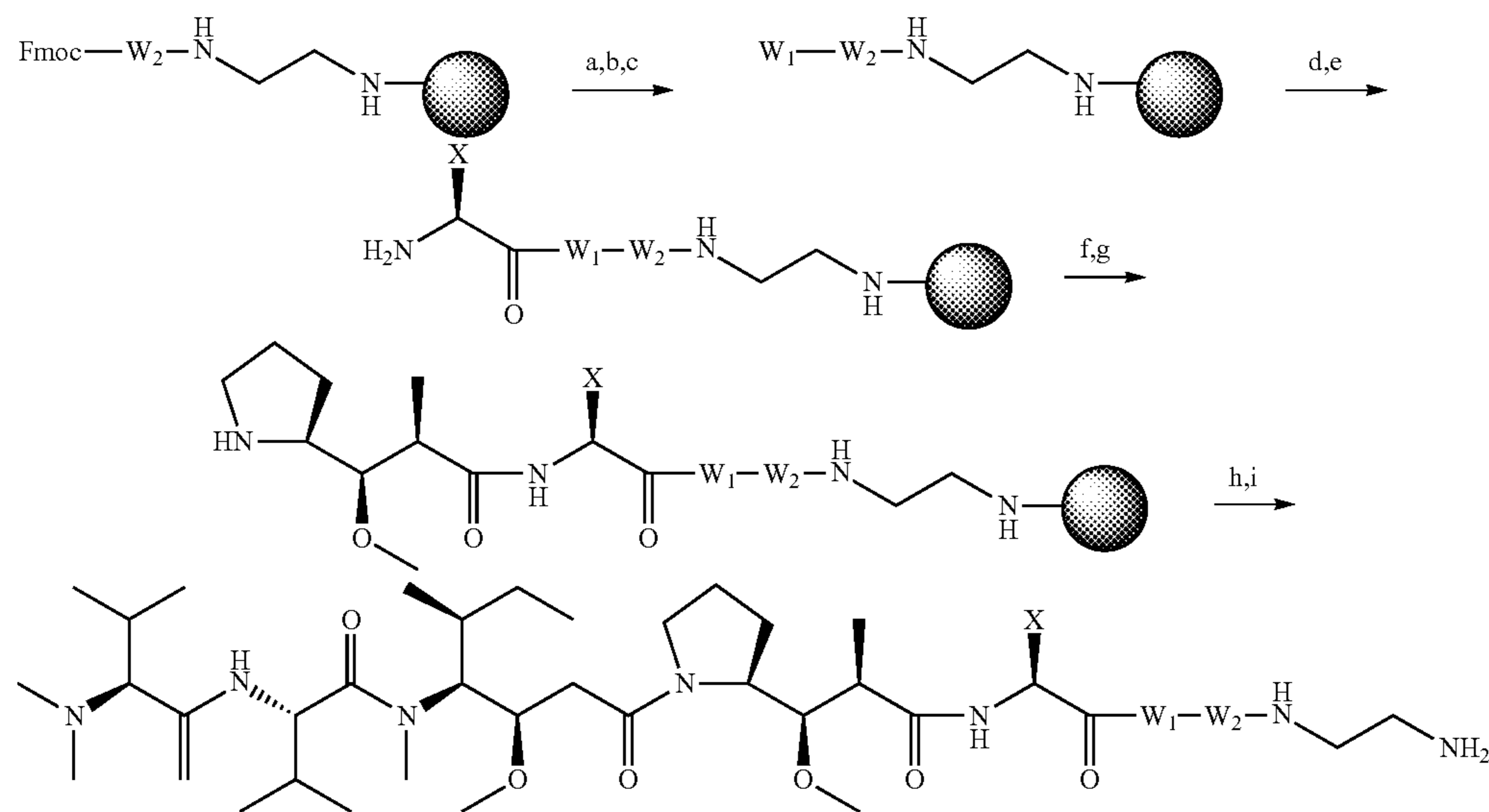
Scheme 1. Solid Phase Synthesis Route
