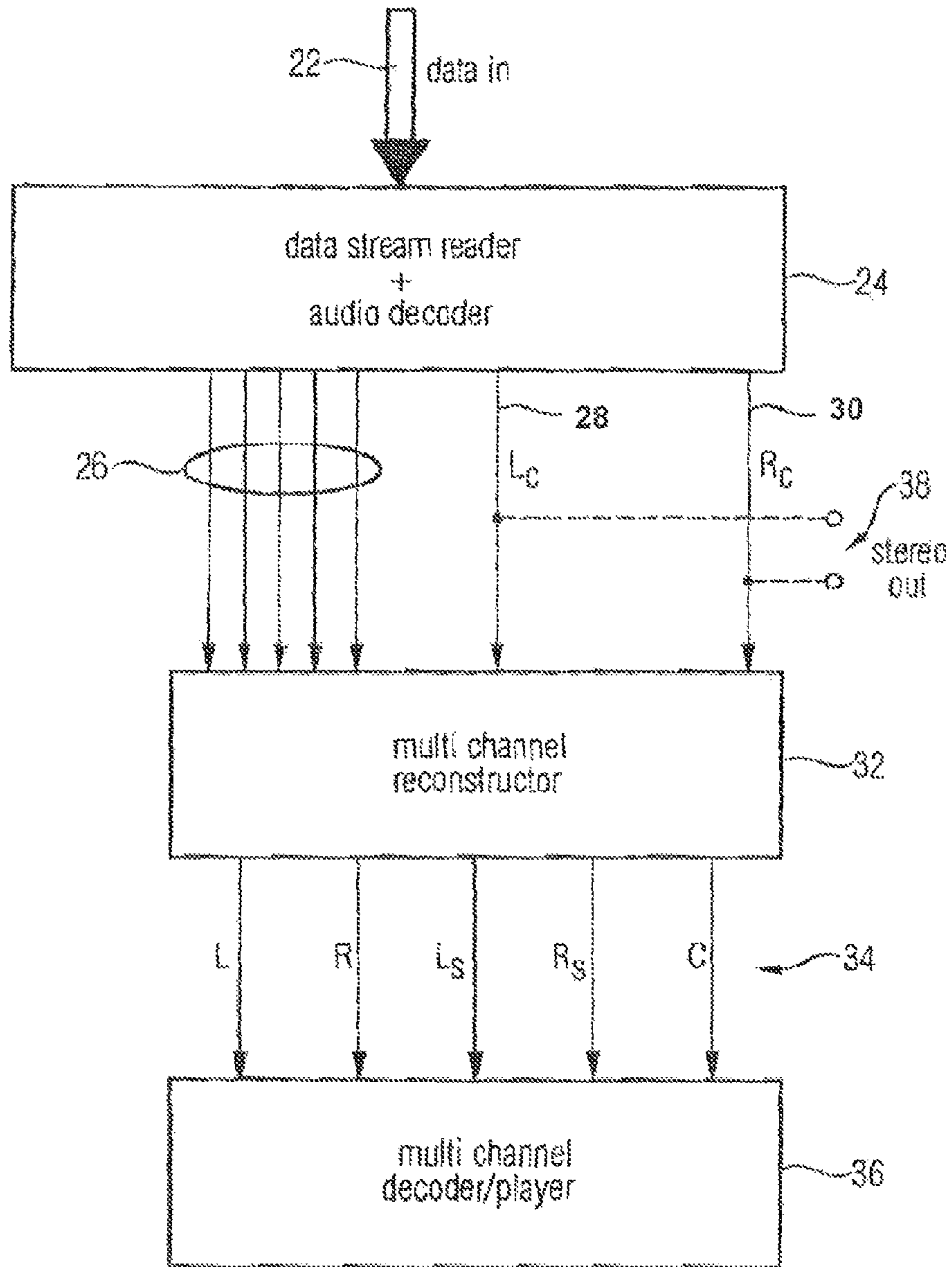
FIG 2 (Decoder)
