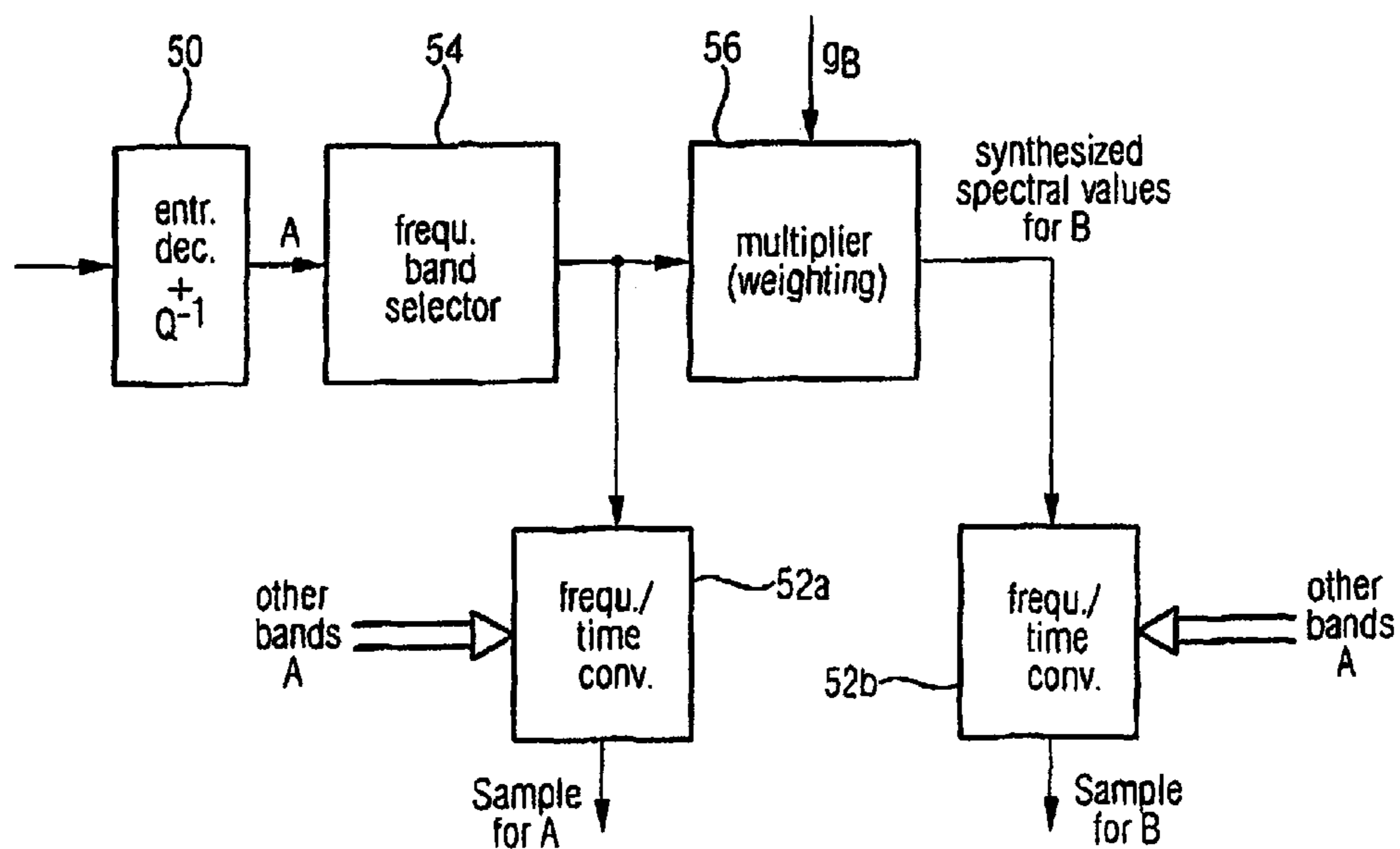
FIG 5 (decoder side)
