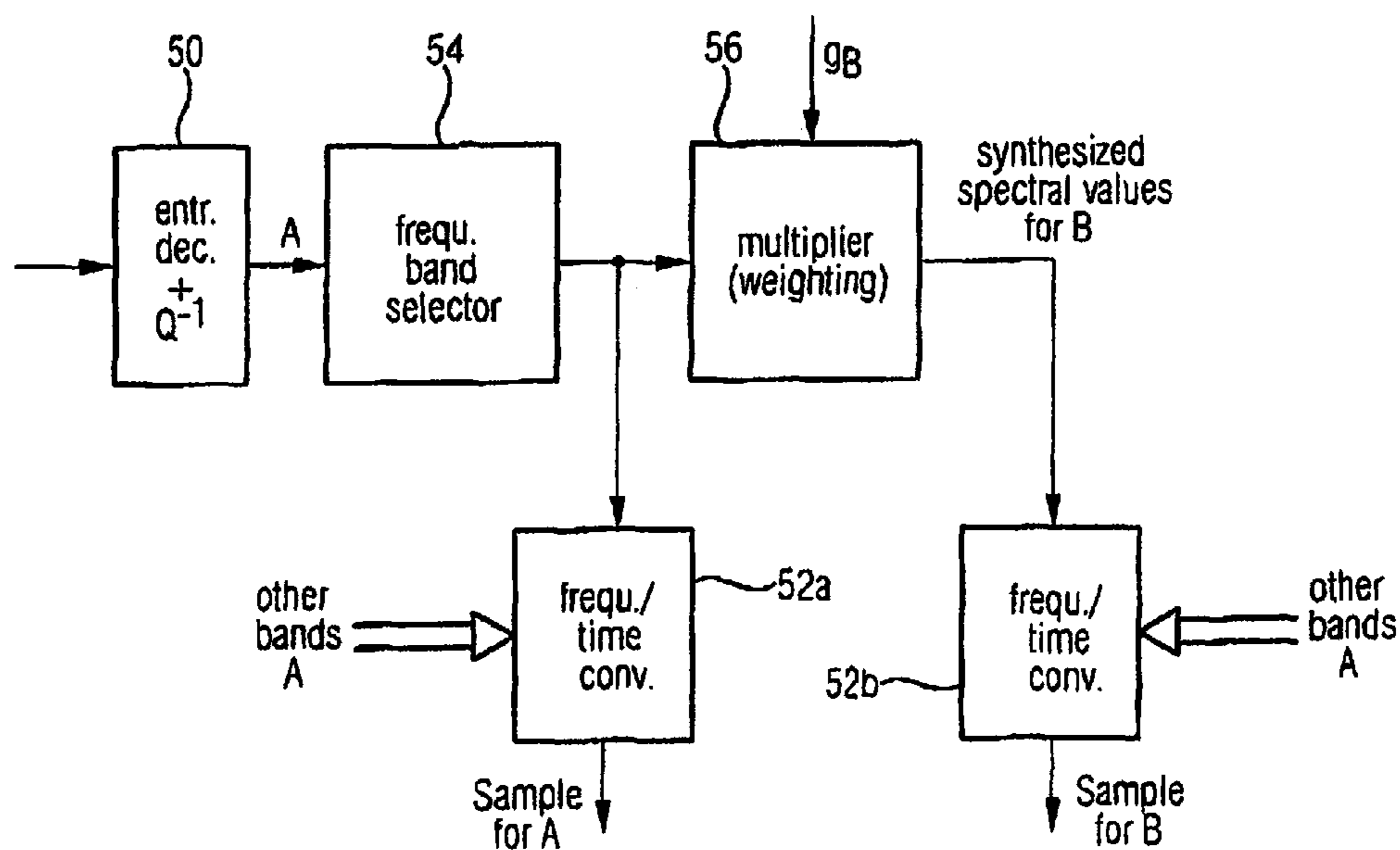
FIG 5 (decoder side)
