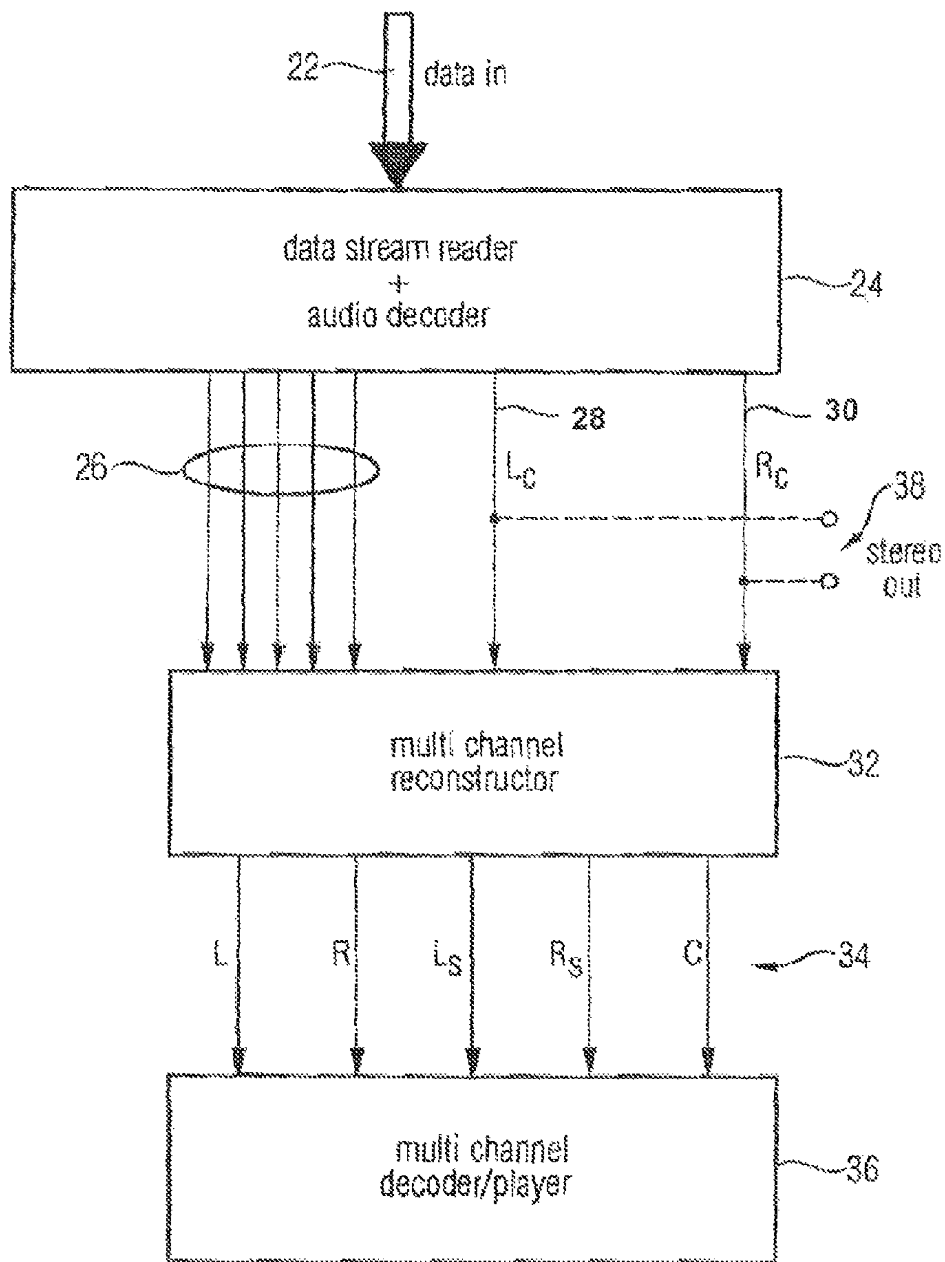
FIG 2 (Decoder)
