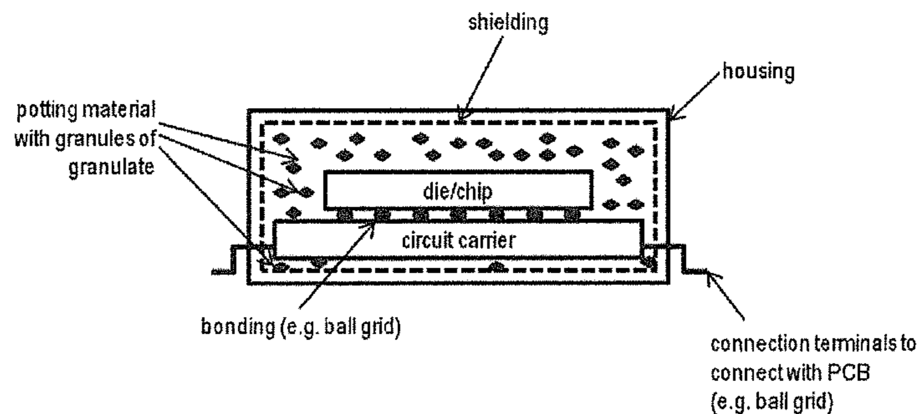
Tamper-protected semiconductor module provided with a cocoon PUF.
