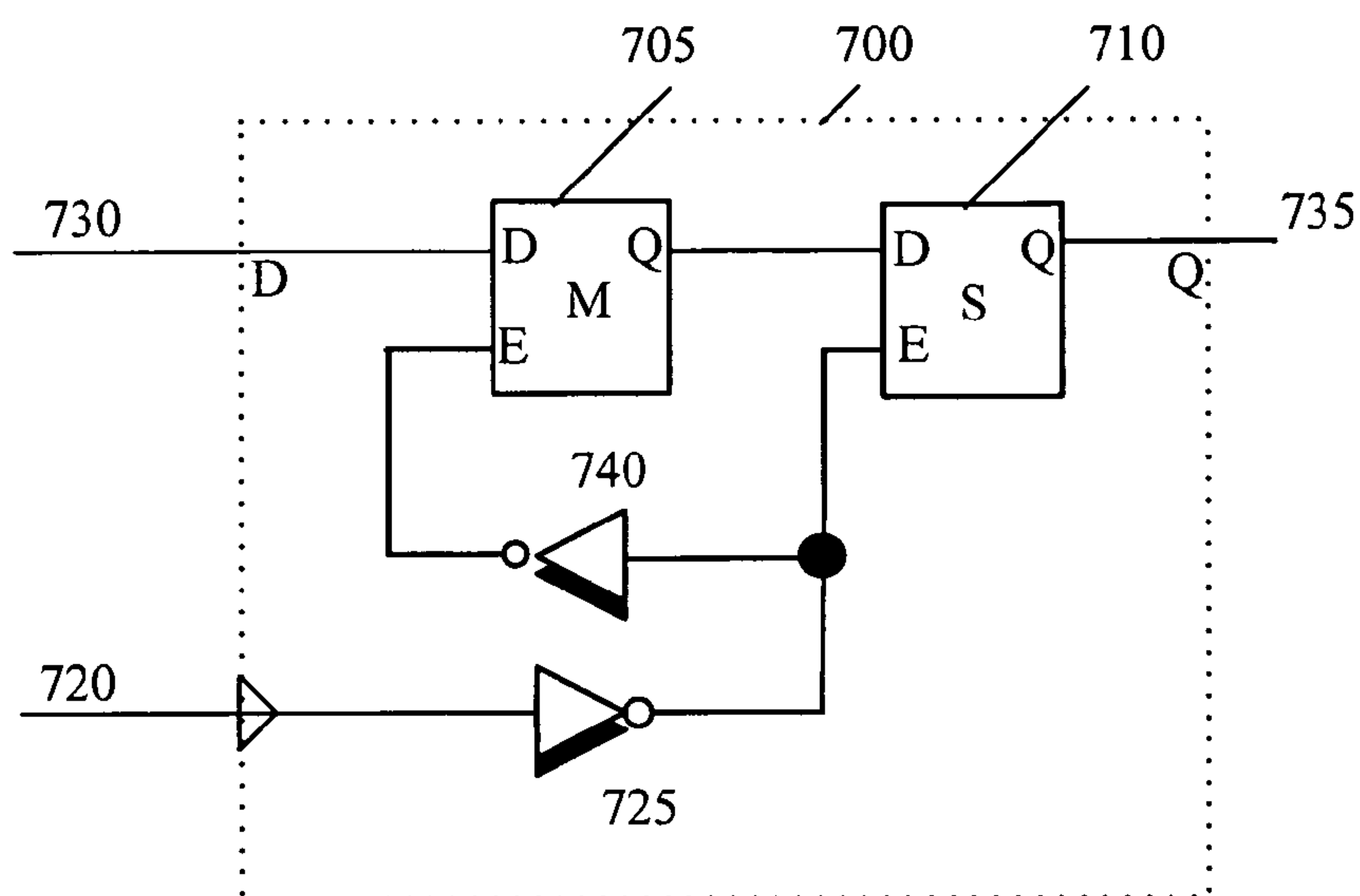
Figure 7 Prior Art
