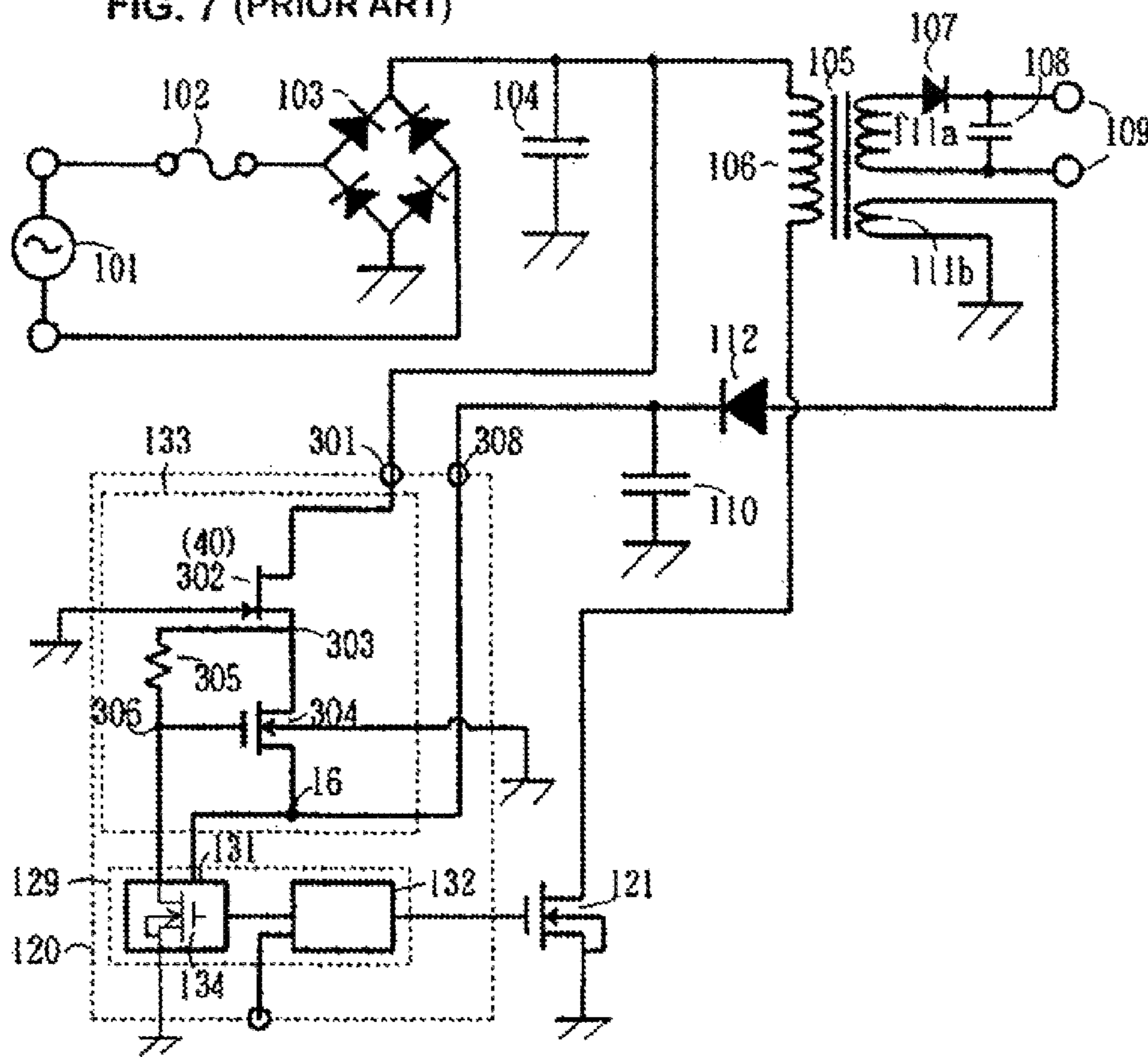
FIG. 7 (PRIOR ART)
