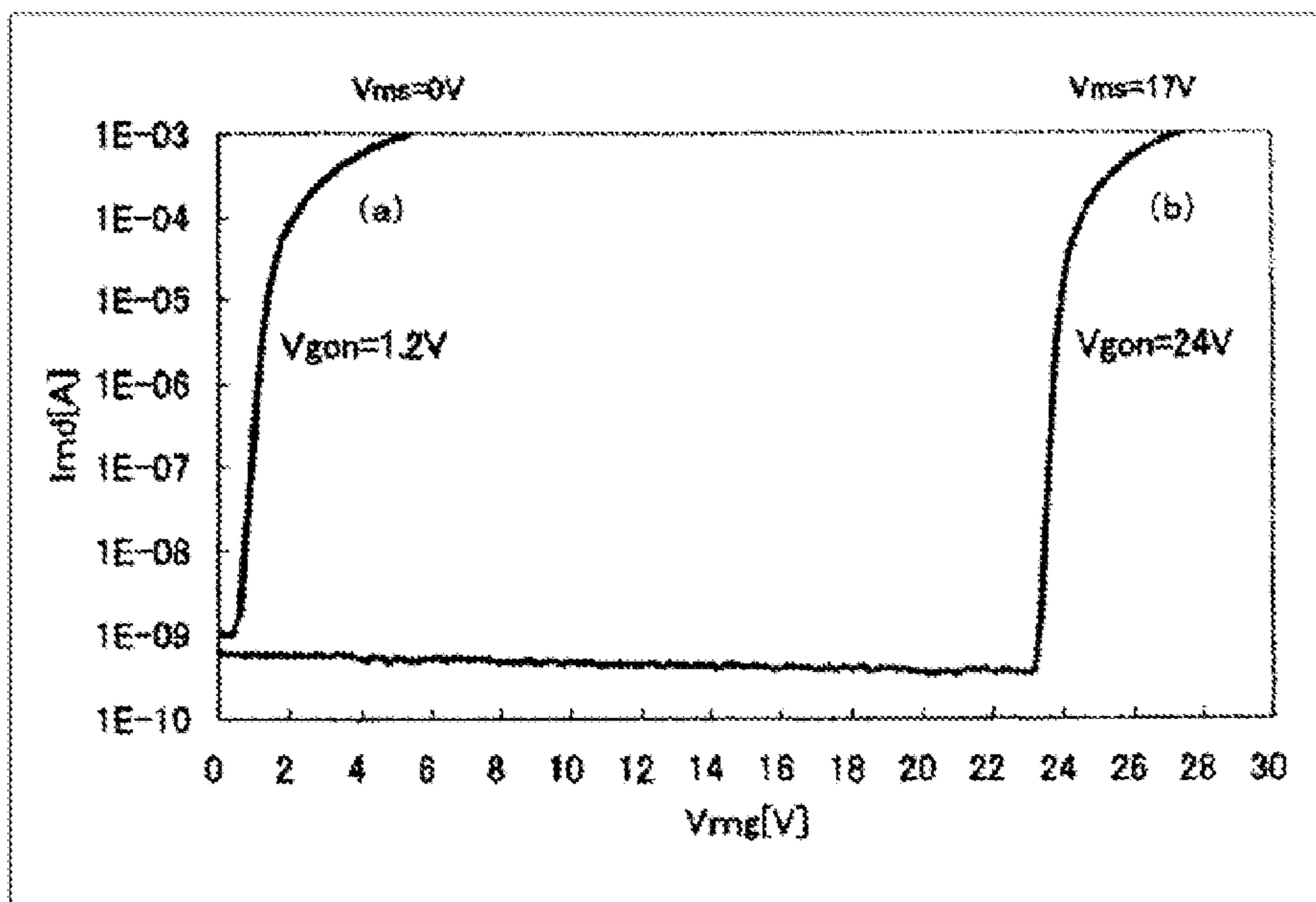
SWITCHING CHARACTERISTIC OF NMOSFET FOR START-UP CIRCUIT
