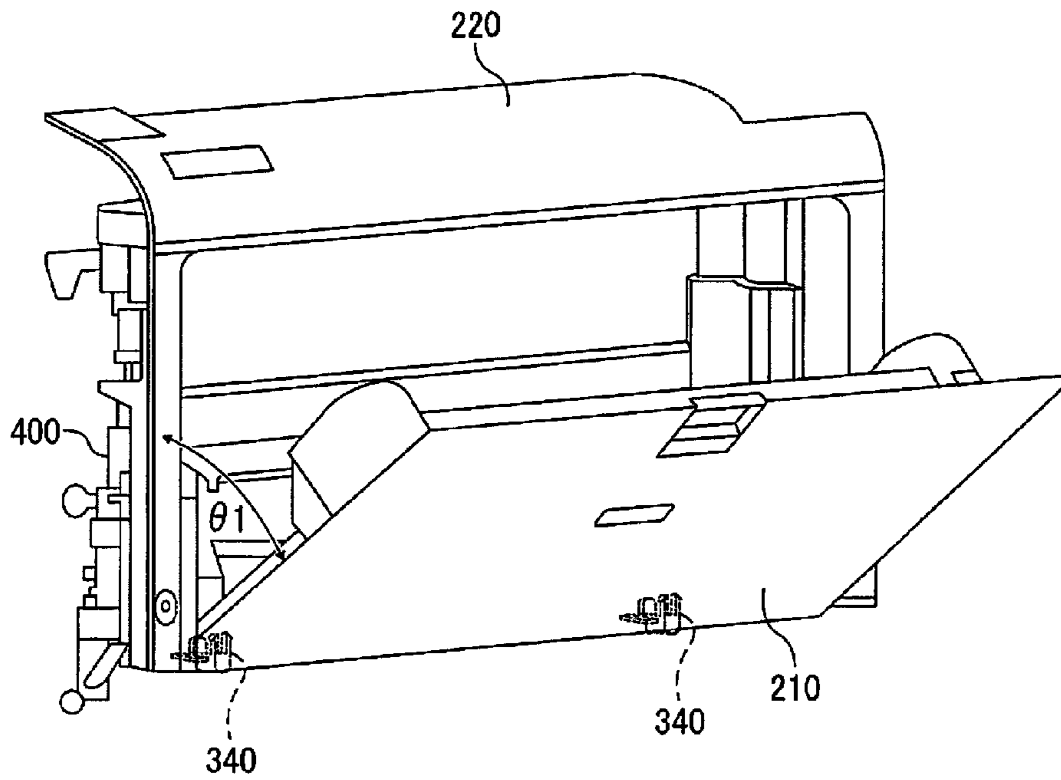
FIG. 2 Prior Art
