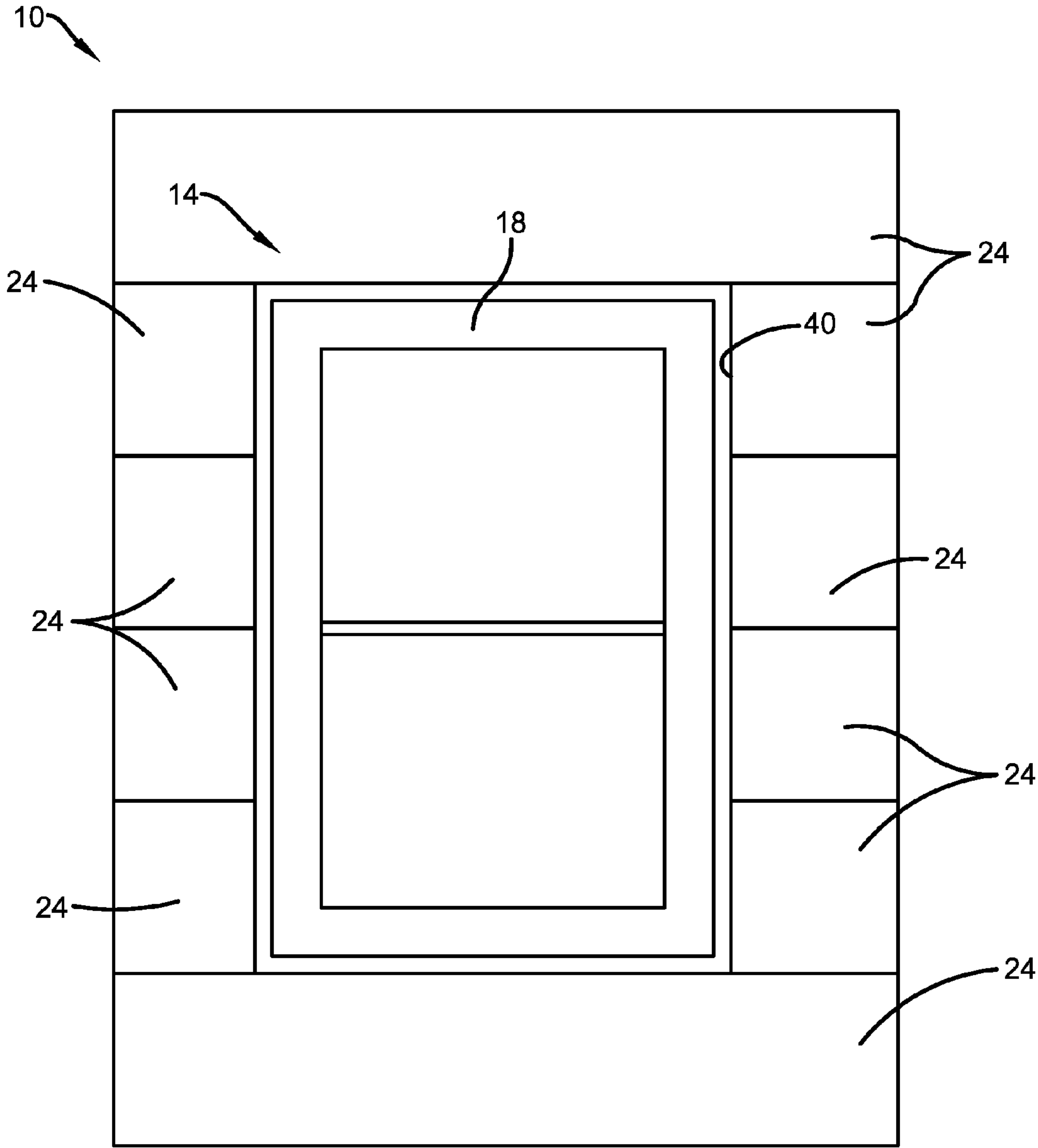
FIG. 4 PRIOR ART
