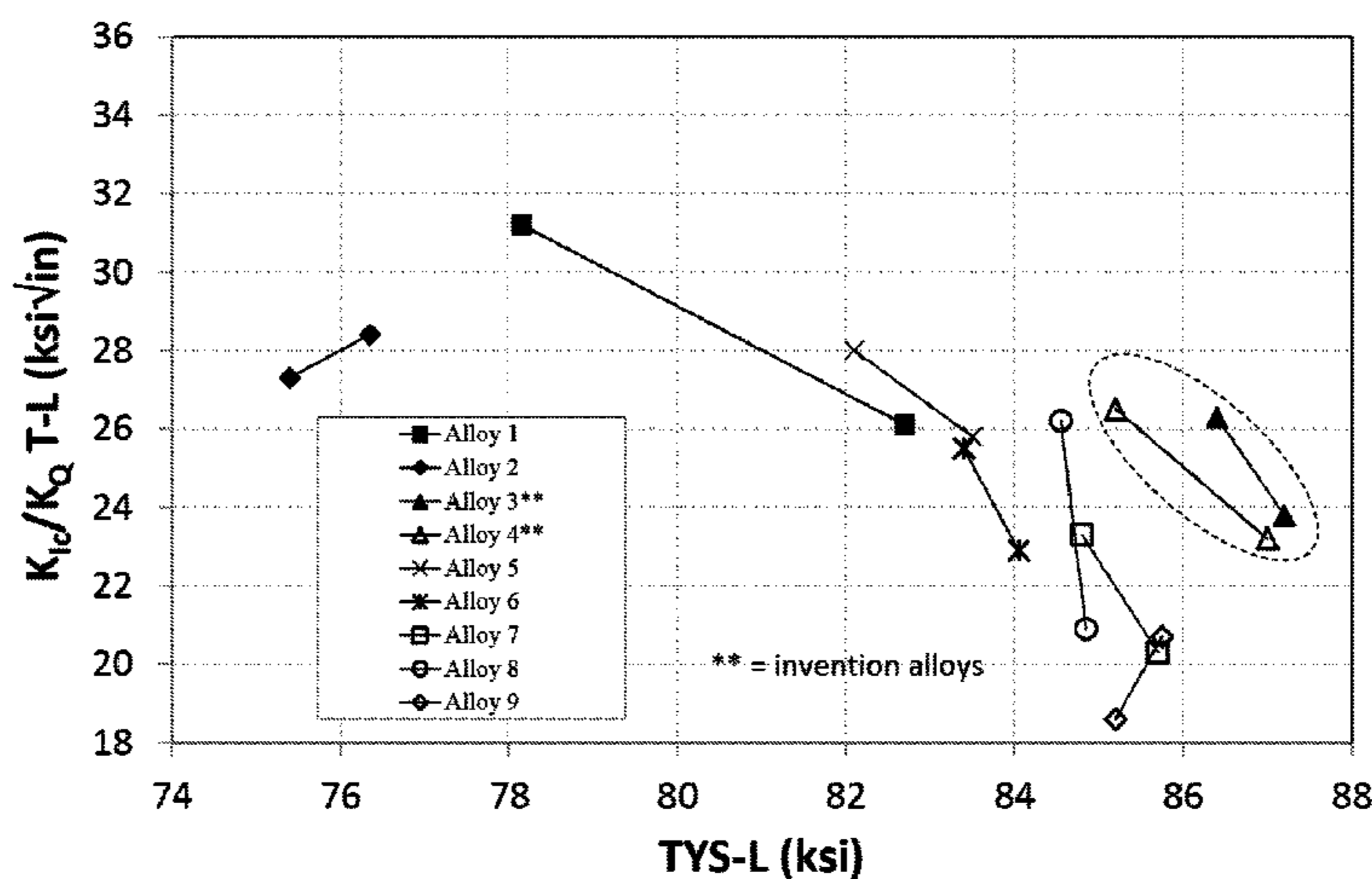
Strength (L) v. Toughness (T-L) for Example 1 Alloys
