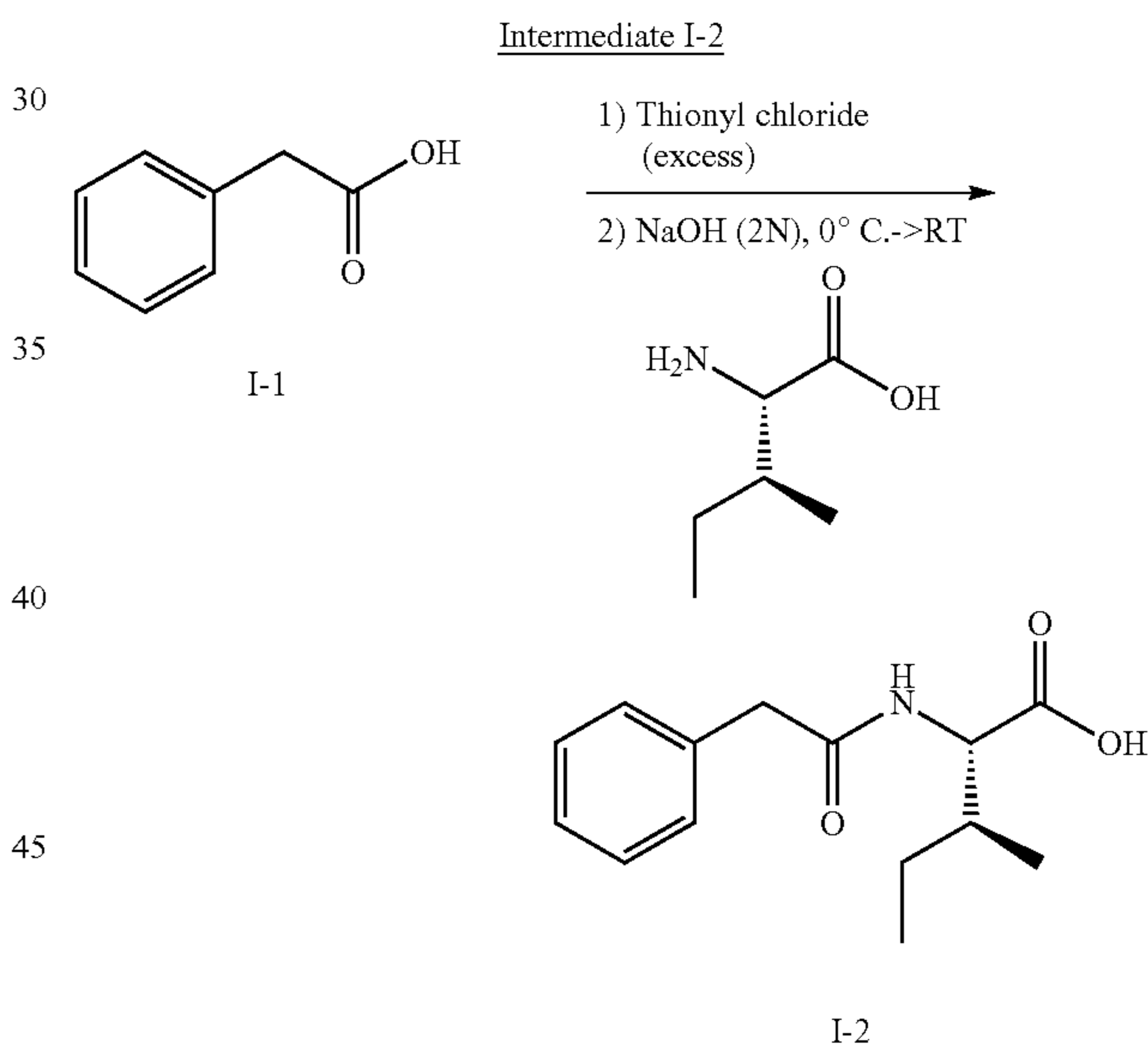
(2S,3S)-3-Methyl-2-(2-phenylacetamido)pentanoic acid (I-2)
