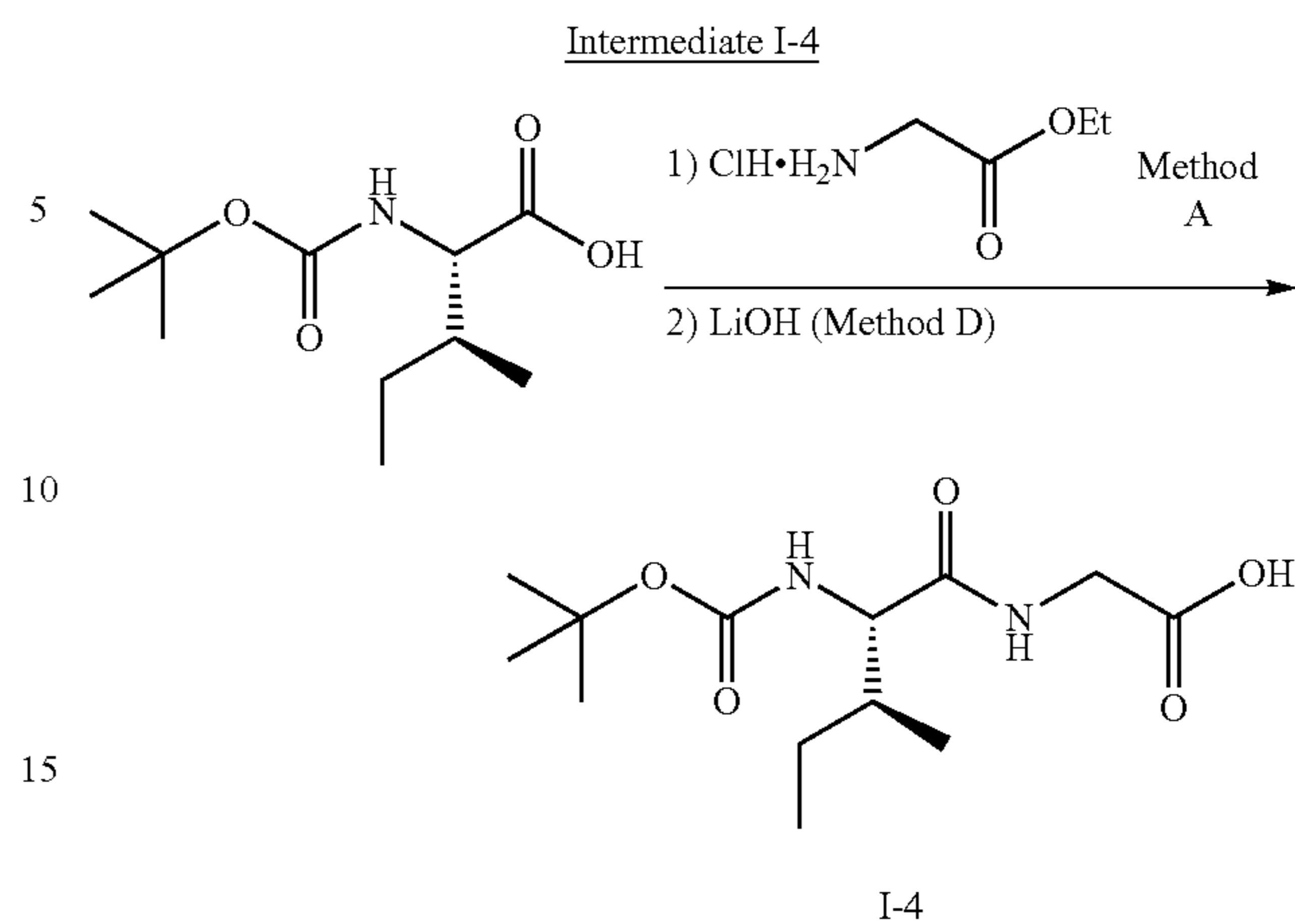
2-((2S,3S)-2-((tert-butoxycarbonyl)amino)-3-methylpentanamido)acetic acid (I-4)
