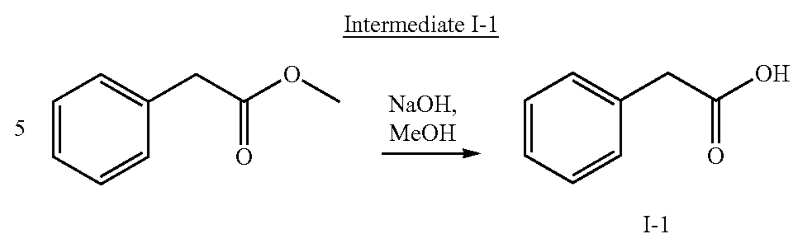
2-Phenylacetic acid (I-1)
