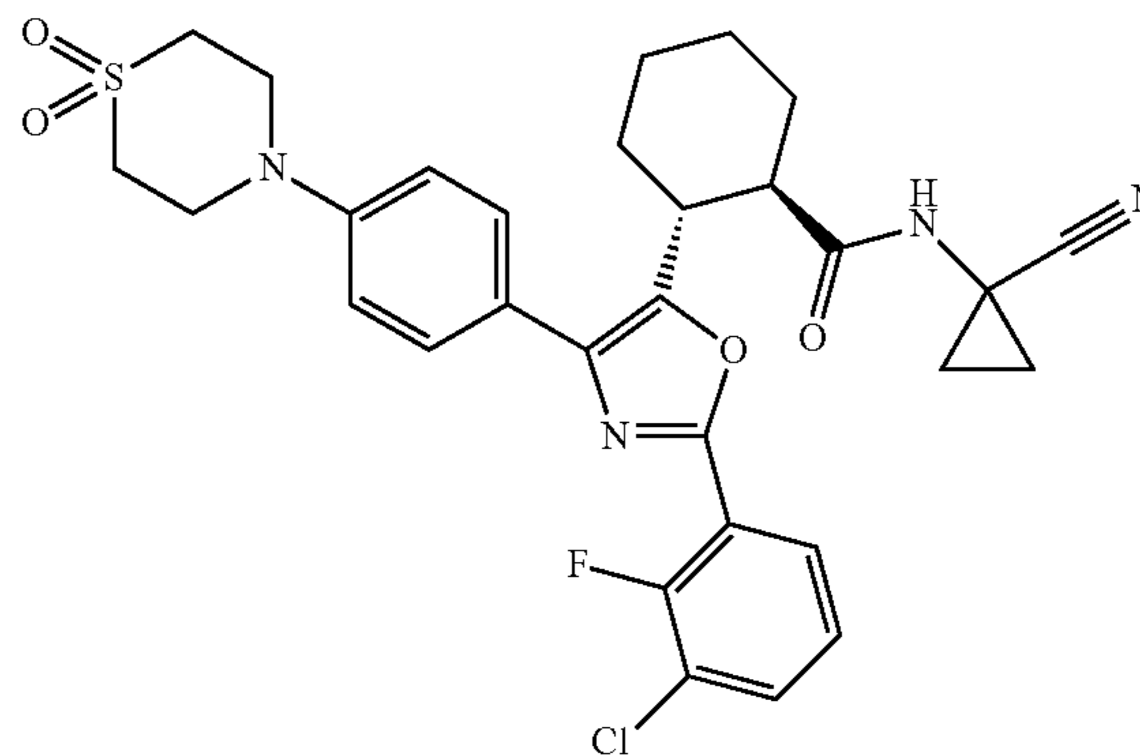
(1R,2R)-2-(2-(3-chloro-2-fluorophenyl)-4-(4-(1,1-dioxidothiomorpholino)phenyl)oxazol-5-yl)-N-(1-cyanocyclopropyl)cyclohexanecarboxamide (Compound 6)
