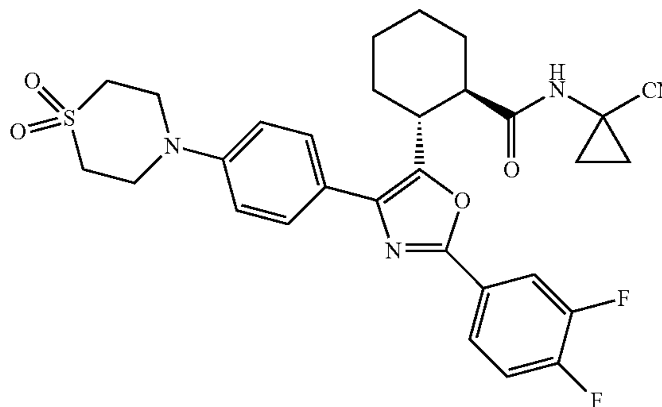
(1R,2R)—N-(1-Cyanocyclopropyl)-2-(2-(3,4-difluorophenyl)-4-(4-(1,1-dioxidothiomorpholino)phenyl)oxazol-5-yl)cyclohexanecarboxamide (Compound 1)
