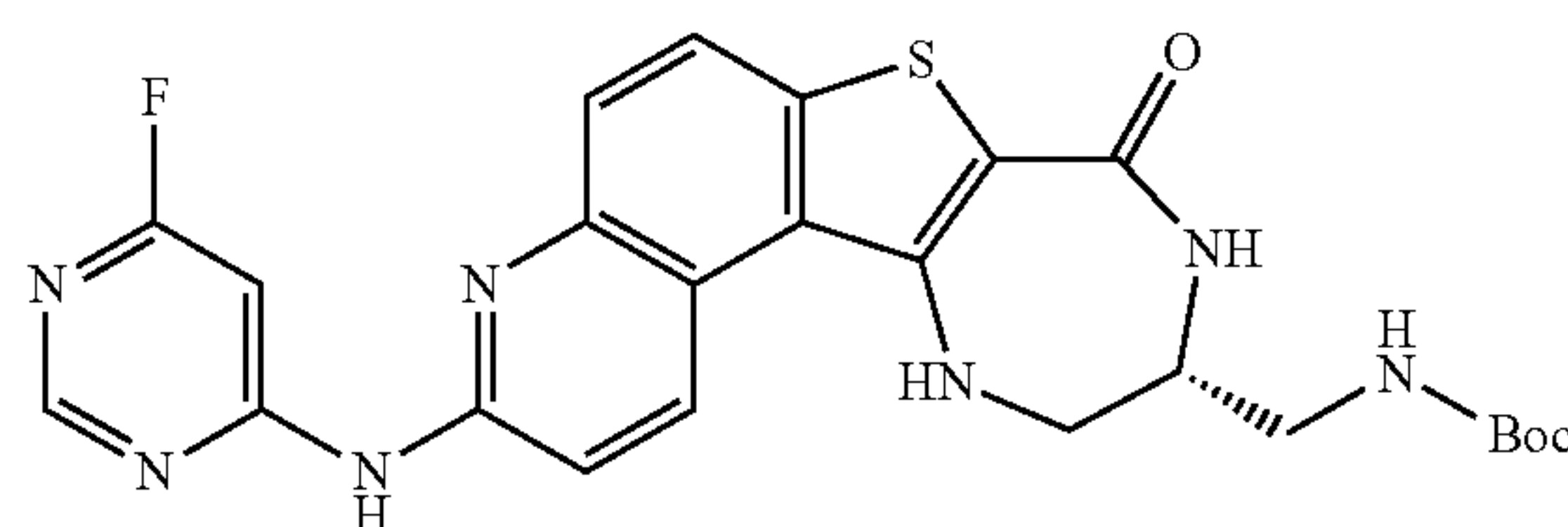
S8-Step 4: Synthesis of (S)-tert-butyl ((3-((6-fluoropyrimidin-4-yl)amino)-8-oxo-9,10,11,12-tetrahydro-8H-[1,4]diazepino[5',6':4,5]thieno[3,2-f]quinolin-10-yl)methyl)carbamate (S8-5)
