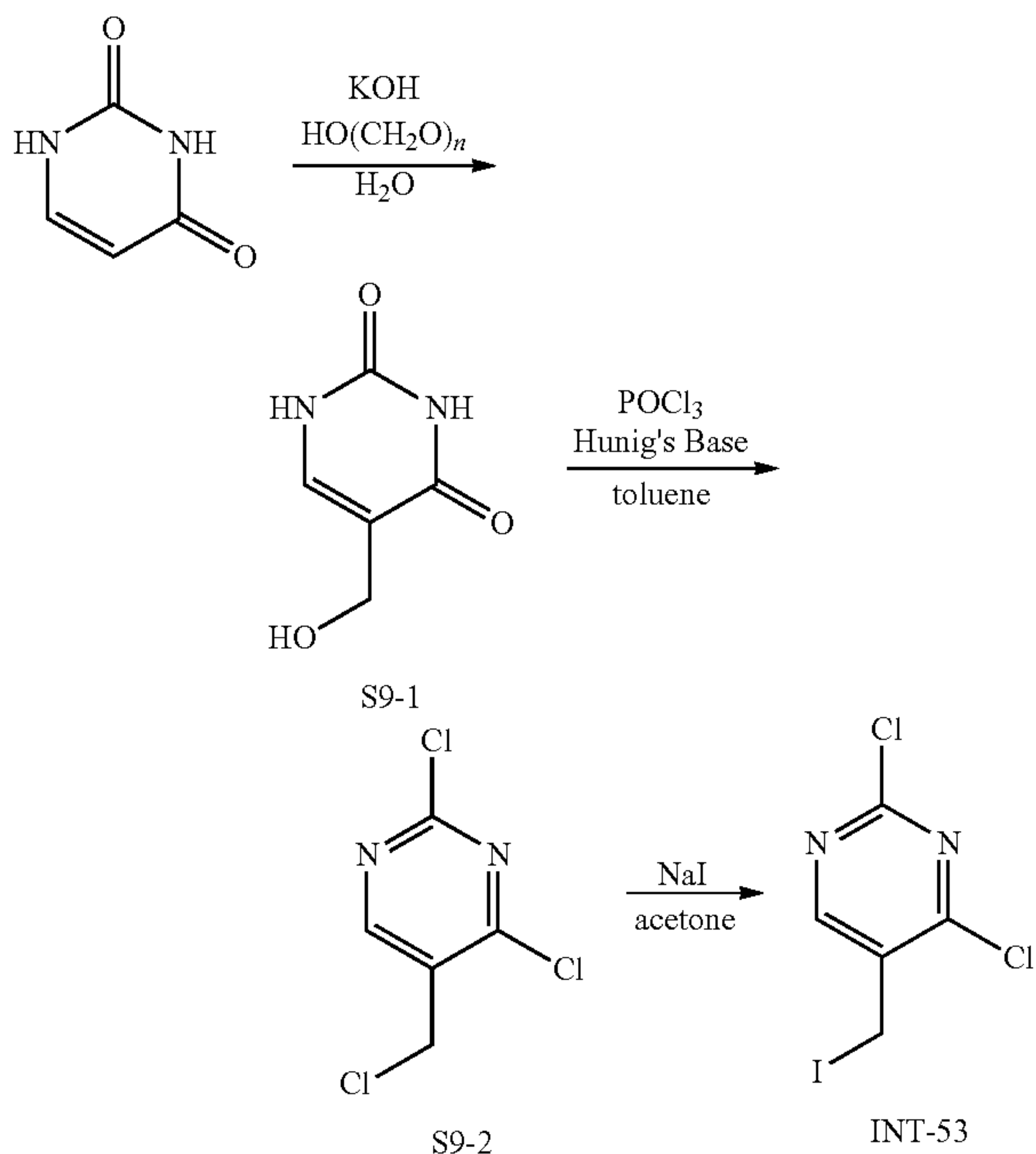
Scheme 9
