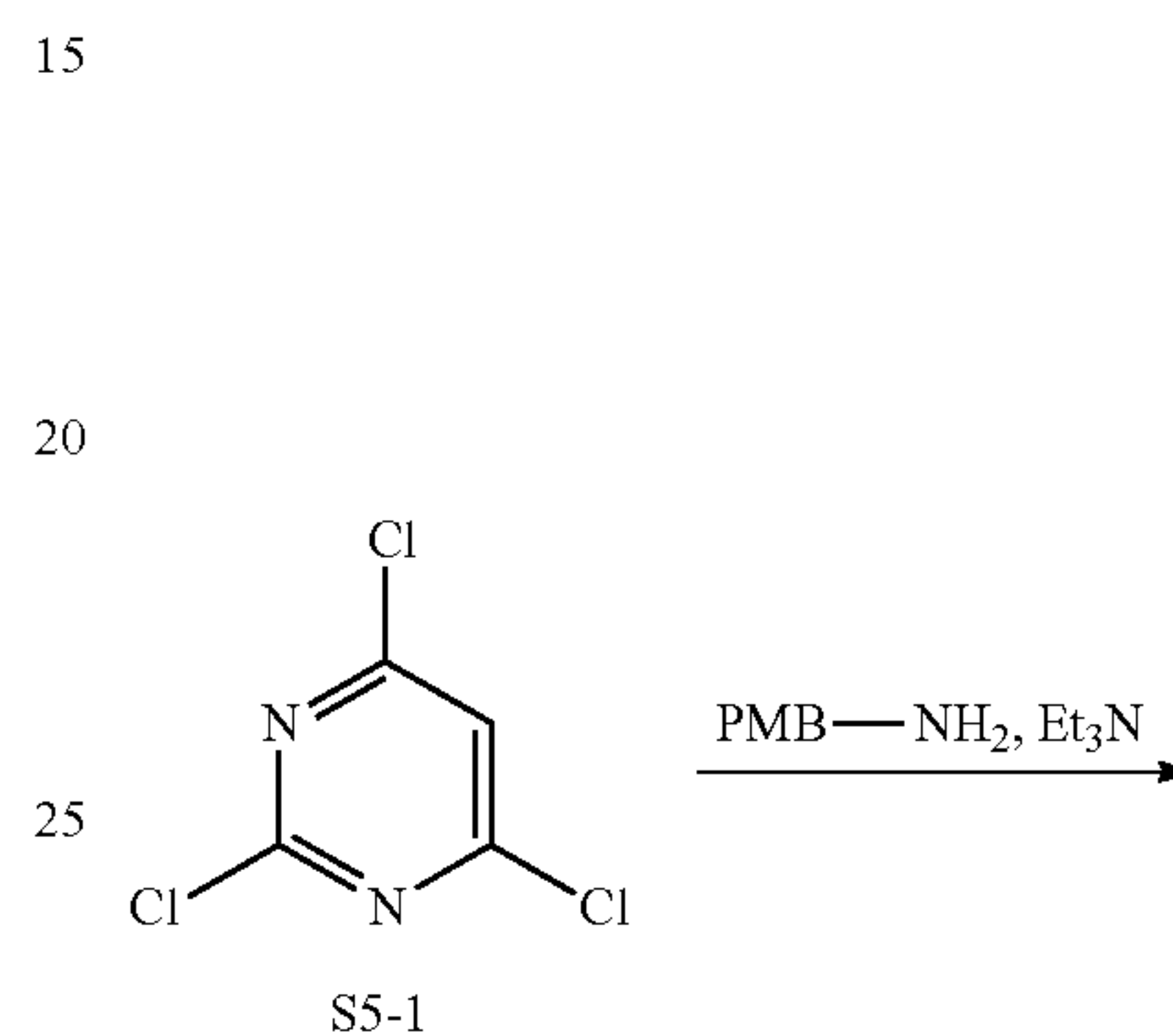
Synthesis of (R)-6-chloro-2-((1-methylpyrrolidin-3-yl)oxy)pyrimidin-4-amine (INT-28)
