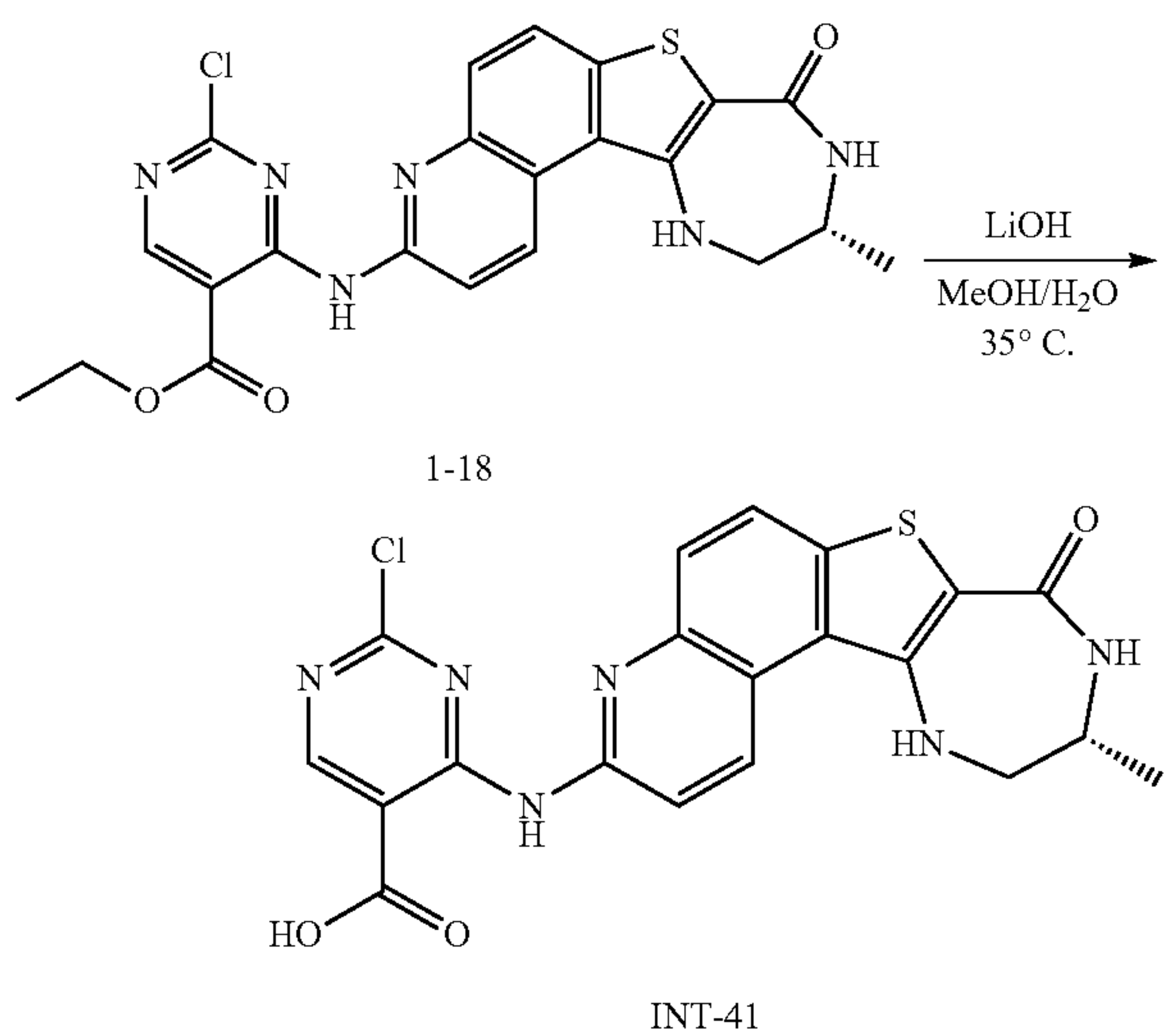
Synthesis of (R)-2-chloro-4-((10-methyl-8-oxo-9,10,11,12-tetrahydro-8H-[1,4]diazepino[5',6':4,5]thieno[3,2-f]quinolin-3-yl)amino)pyrimidine-5-carboxylic acid (INT-41)
