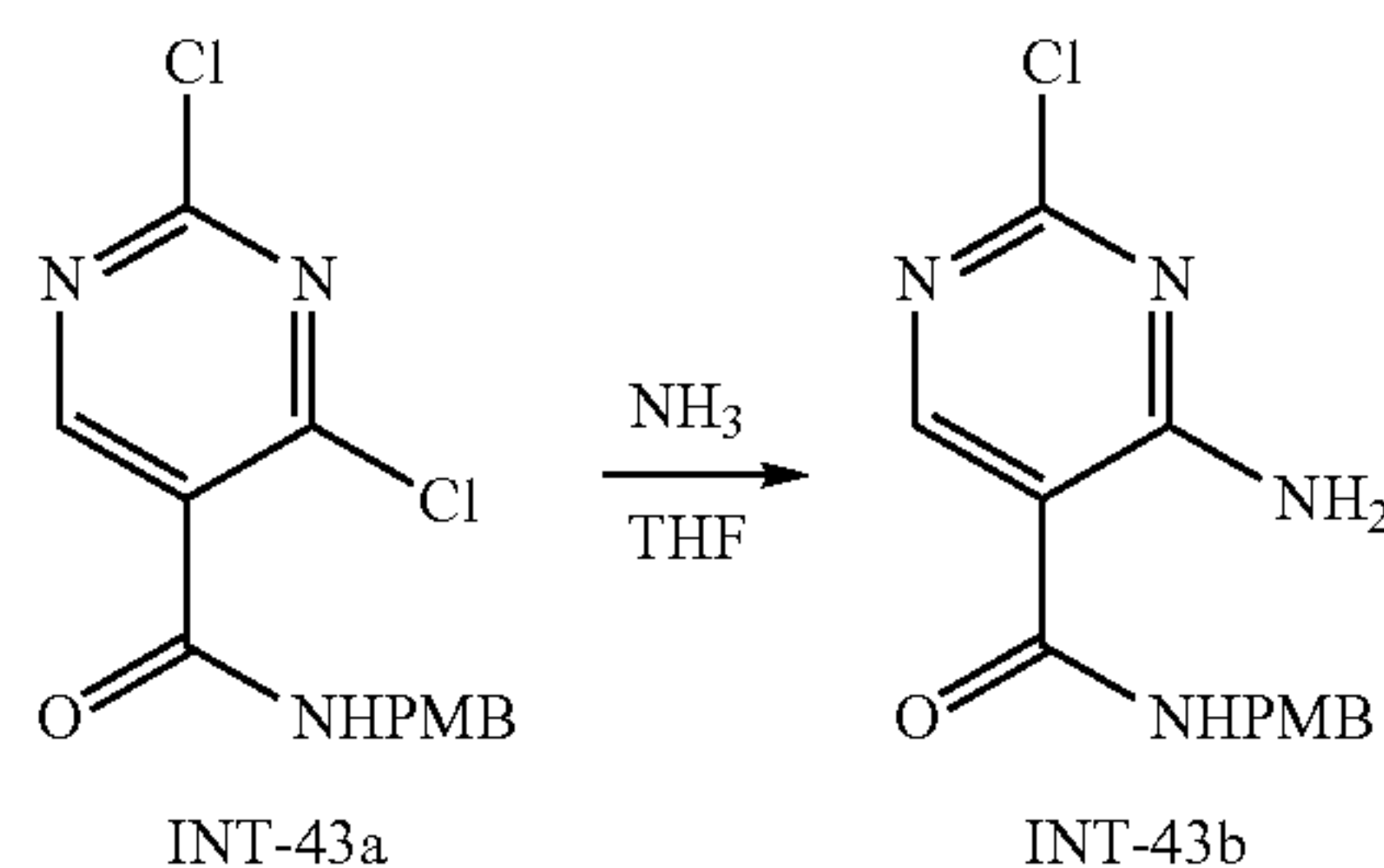
Synthesis of 4-amino-2-chloro-N-(4-methoxybenzyl)pyrimidine-5-carboxamide (INT-43b)
