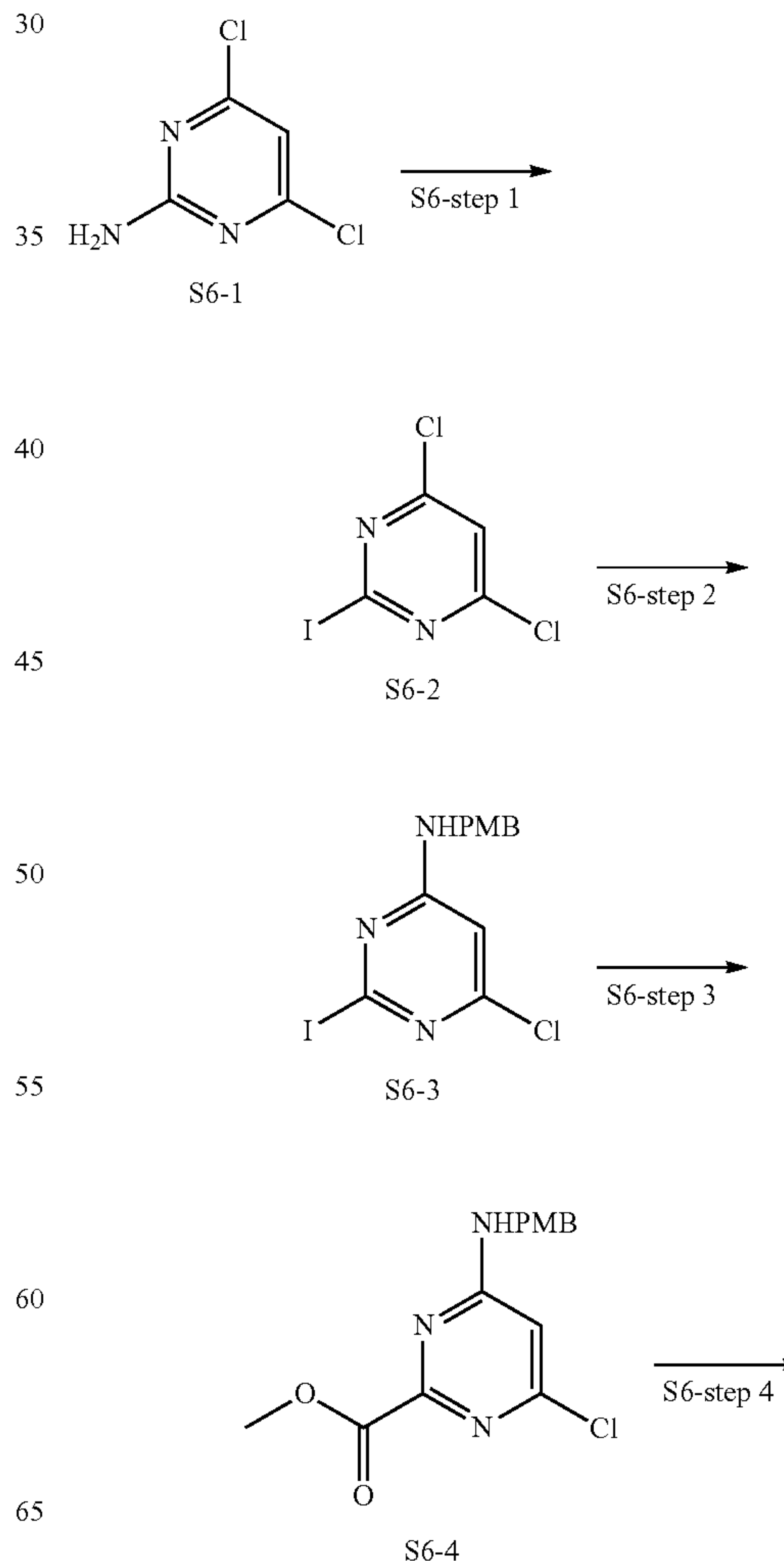
Scheme 6
