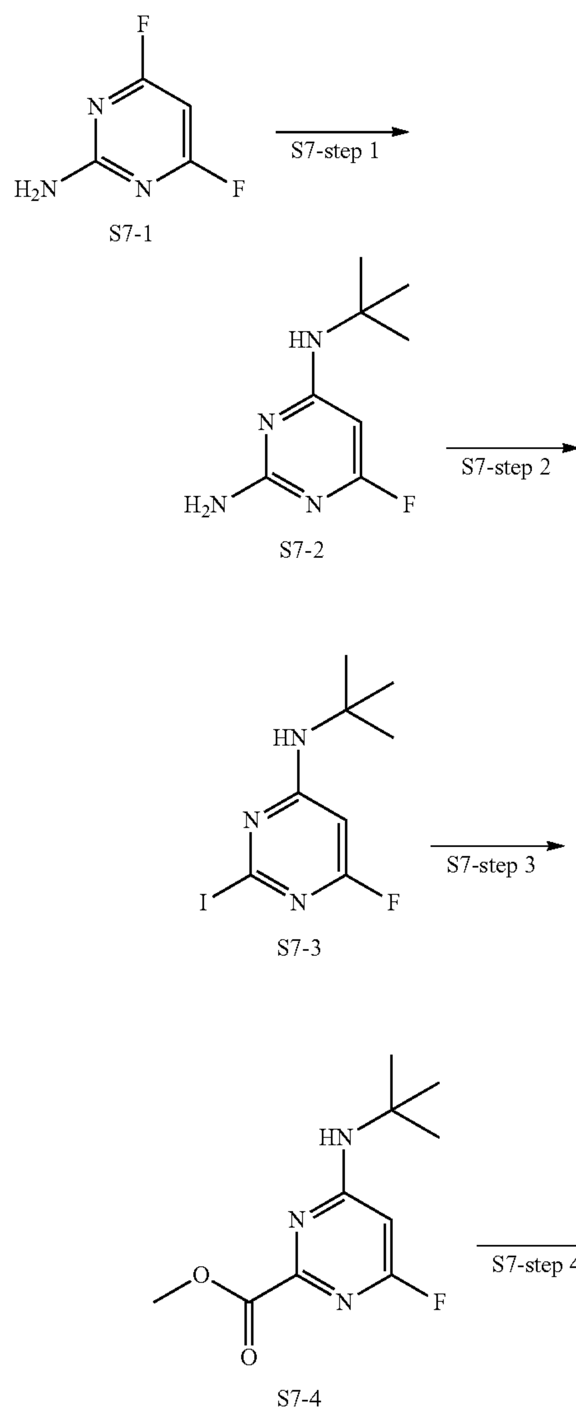
Scheme 7
