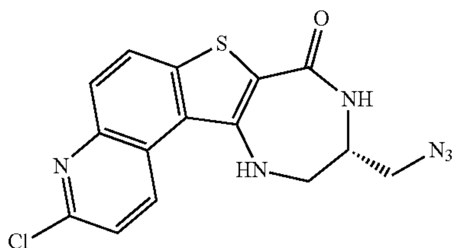
S8-Step 2: Synthesis of (S)-10-(azidomethyl)-3-chloro-9,10,11,12-tetrahydro-8H-[1,4]diazepino[5',6':4,5]thieno[3,2-f]quinolin-8-one (S8-3)
