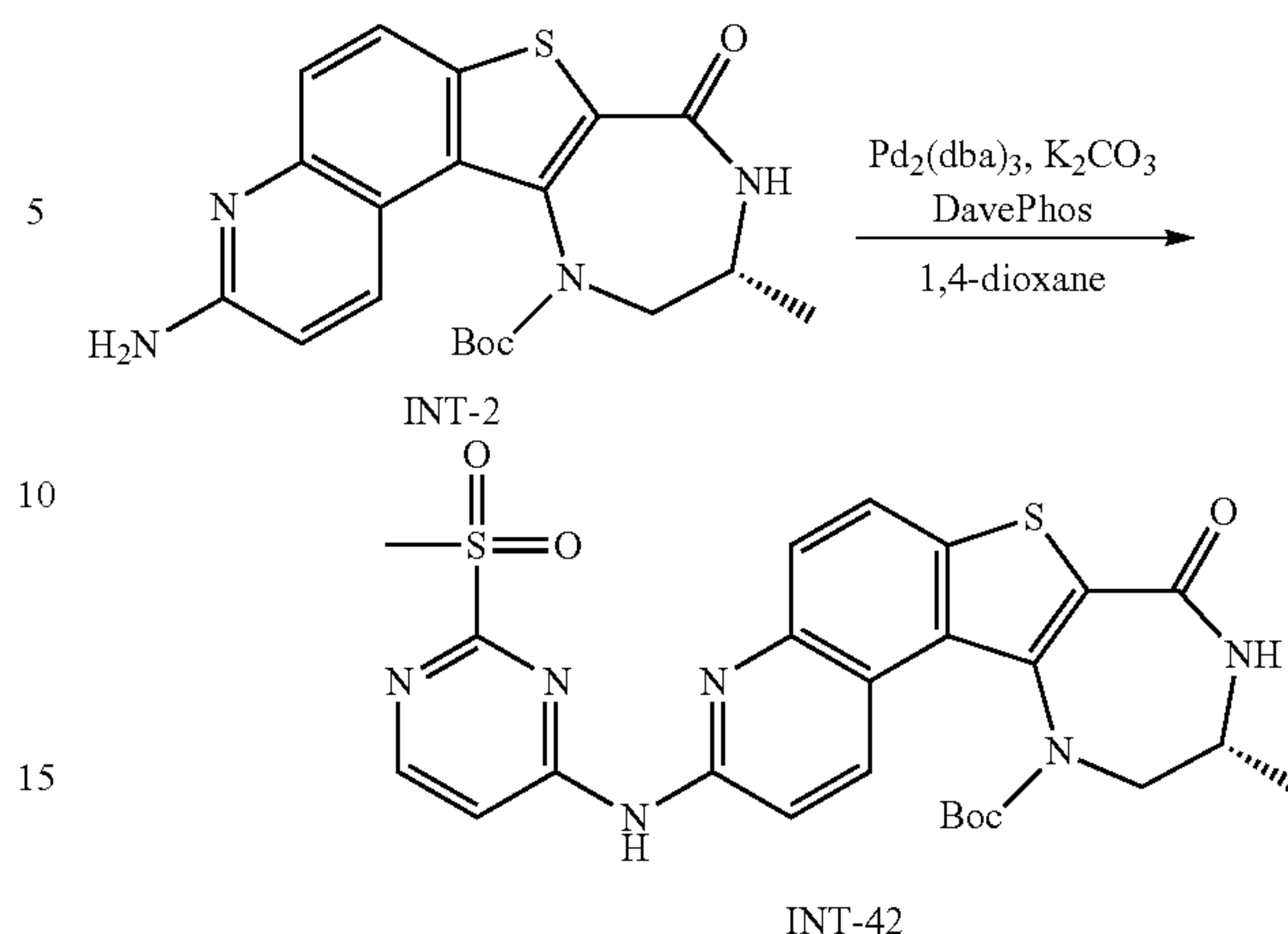
Synthesis of (R)-tert-butyl 10-methyl-3-((2-(methylsulfonyl)pyrimidin-4-yl)amino)-8-oxo-10,11-dihydro-8H-[1,4]diazepino[5',6':4,5]thieno[3,2-f]quinoline-12(9H)-carboxylate (INT-42)
