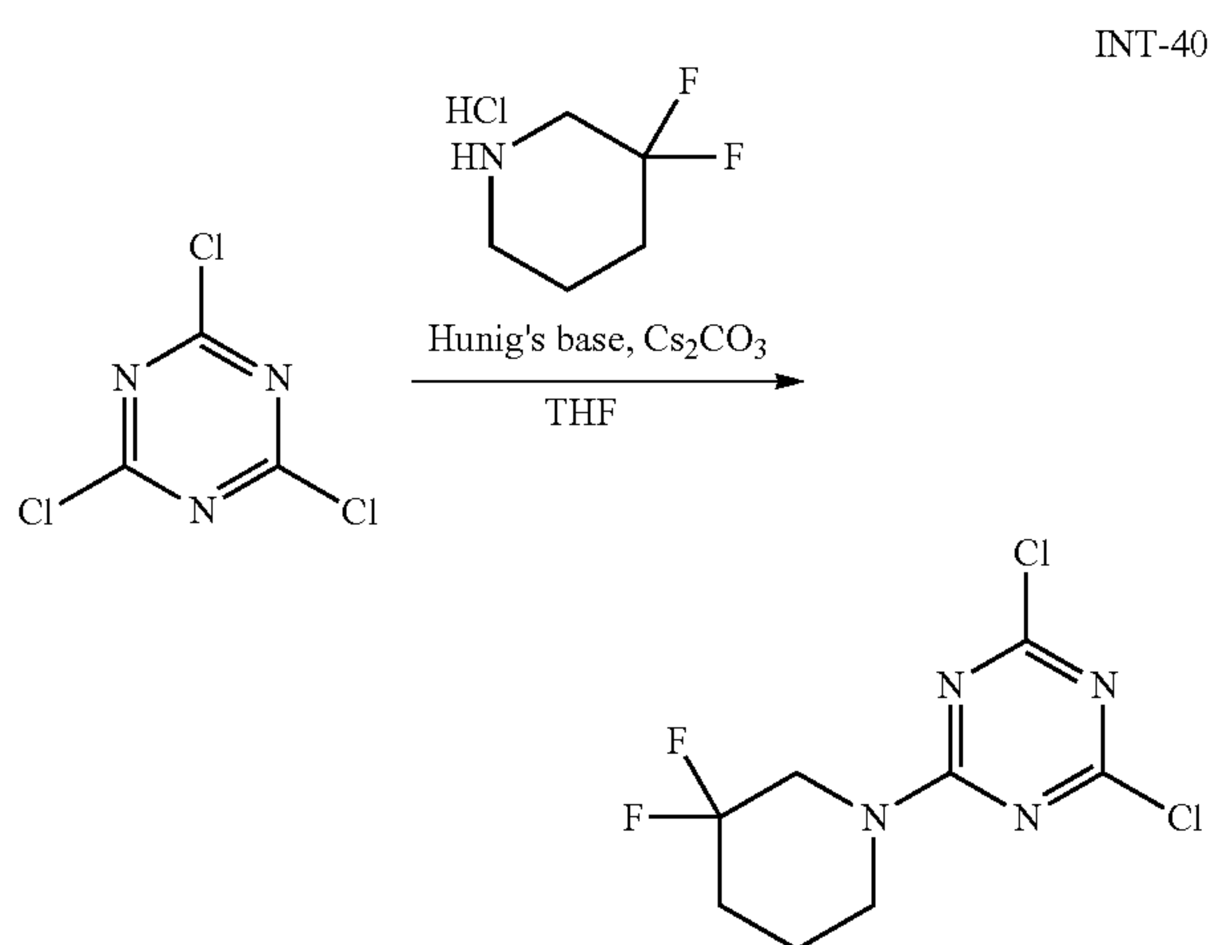
Synthesis of 2,4-dichloro-6-(3,3-difluoropiperidin-1-yl)-1,3,5-triazine (INT-40)
