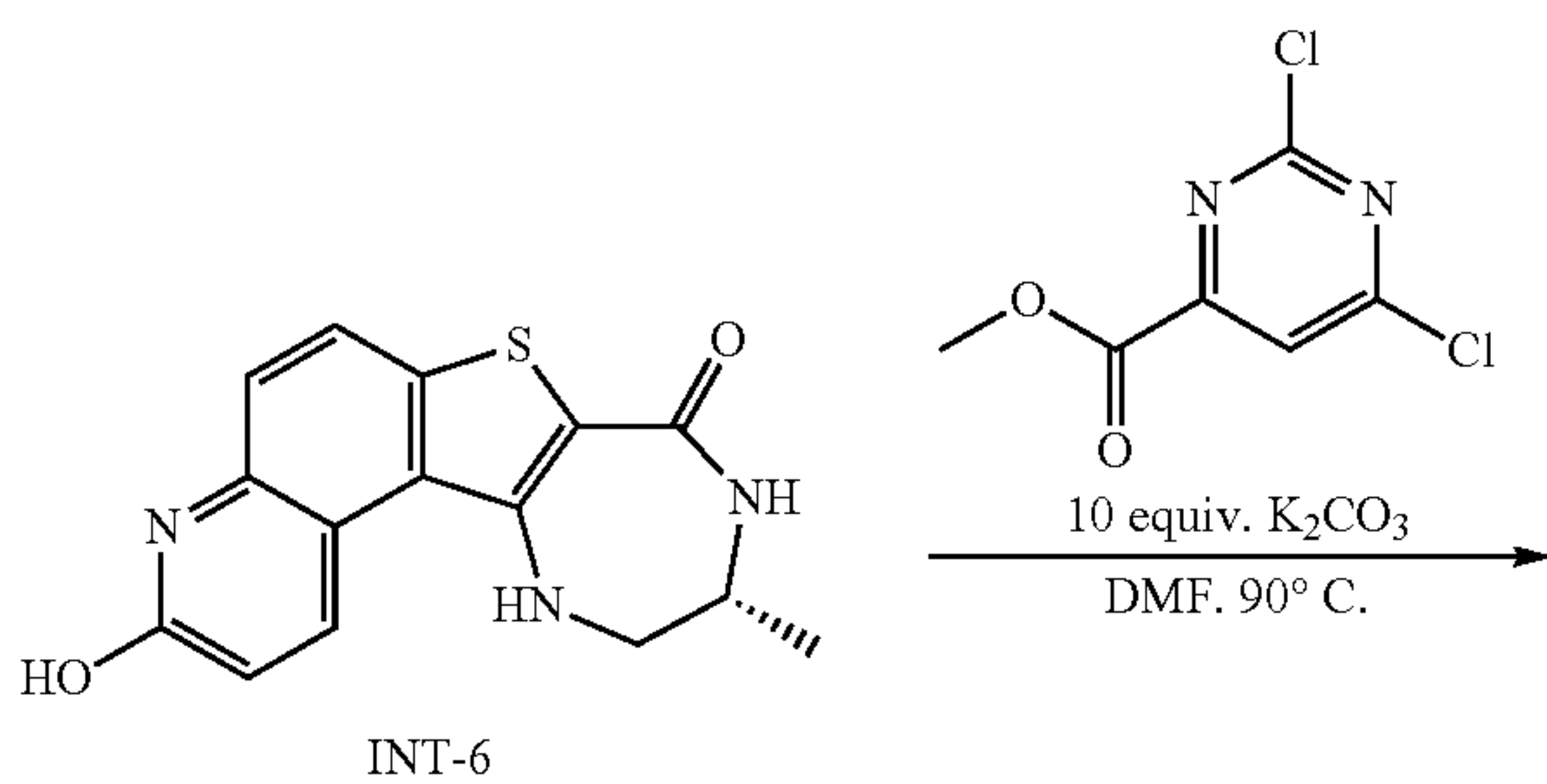
Scheme 10
