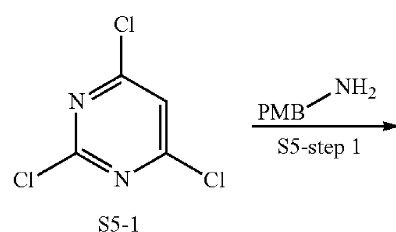
Scheme 5
