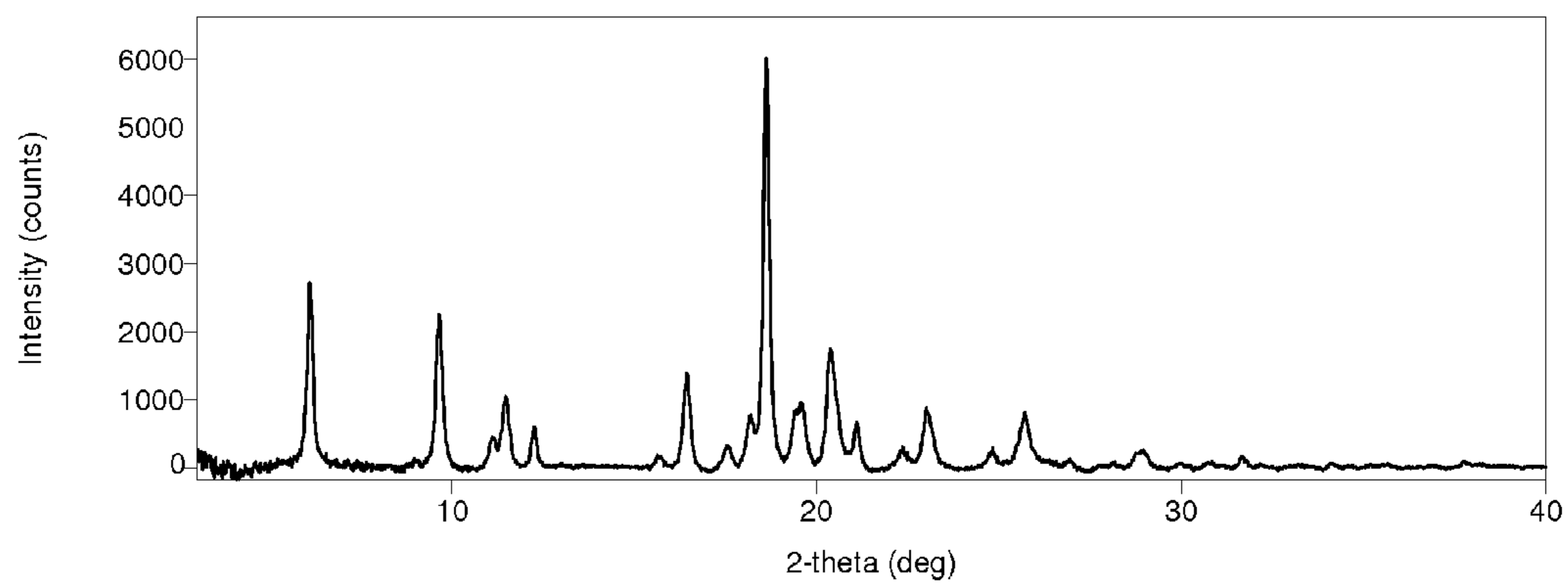
Representative XRPD pattern of crystalline Form A of Compound 3
