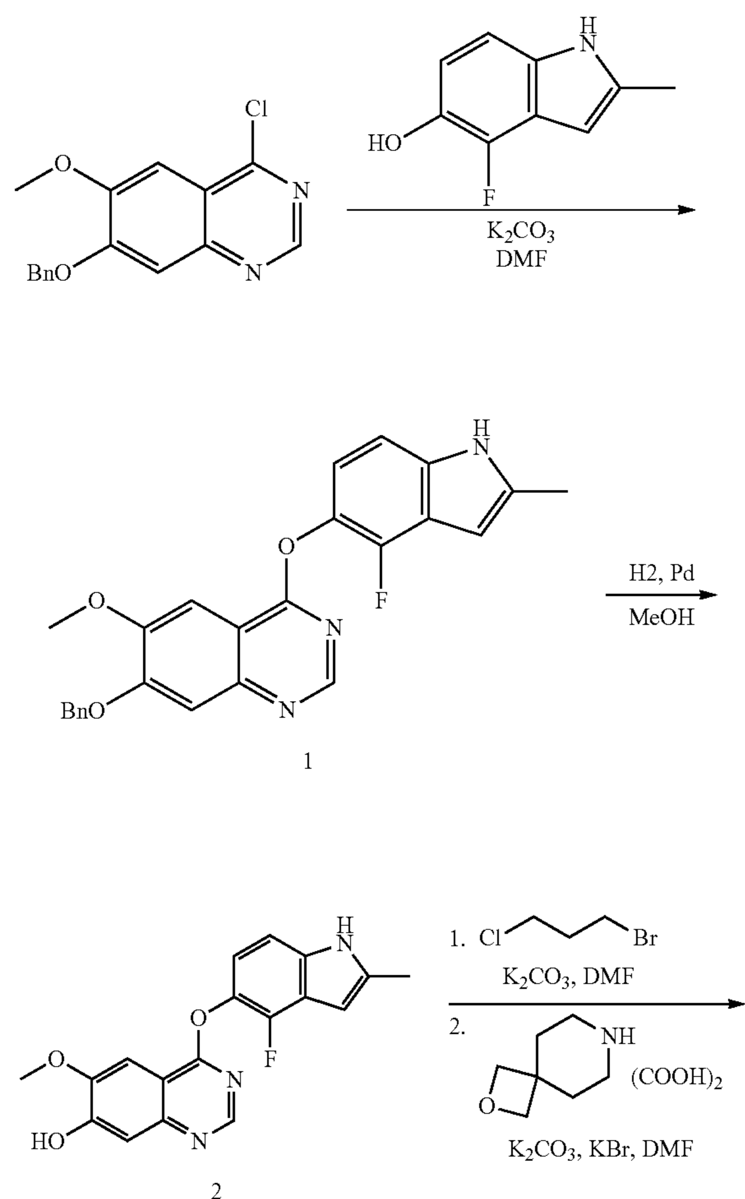
Scheme 1: Method A of synthesizing Compound 3.
