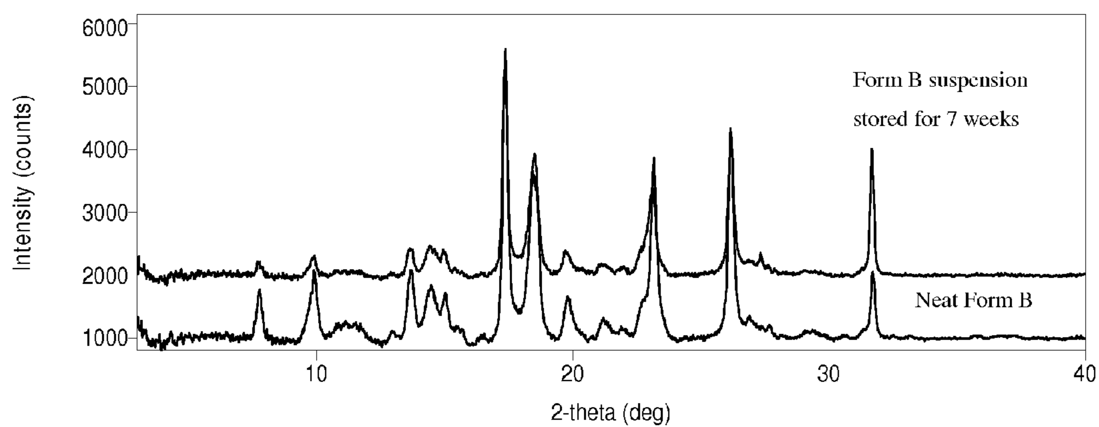
XRPD pattern of neat crystalline Form B of Compound 3 (bottom) and crystalline Form B in suspension stored for 7 weeks (top)
