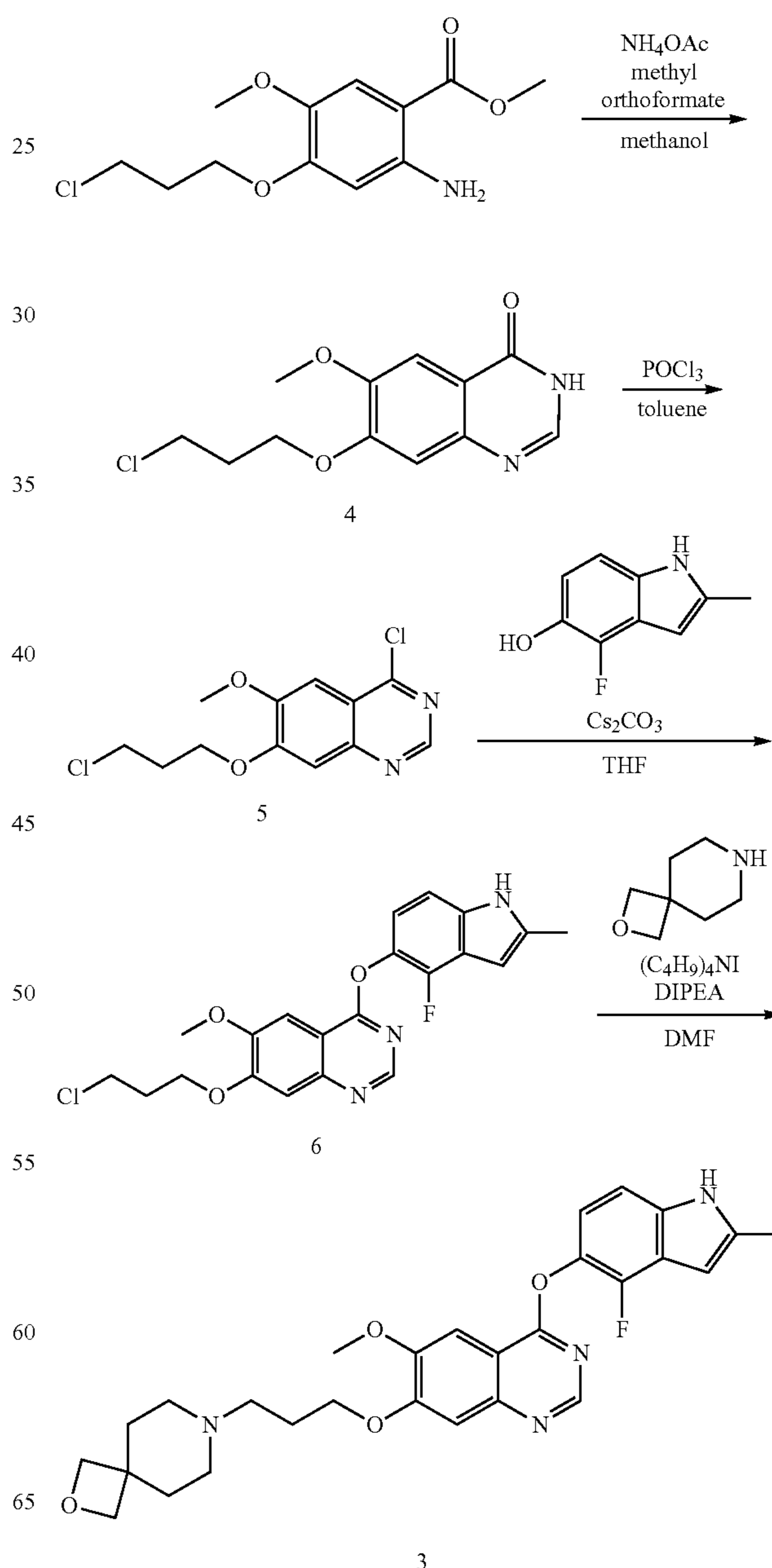
Scheme 2: Method B of synthesizing Compound 3.
