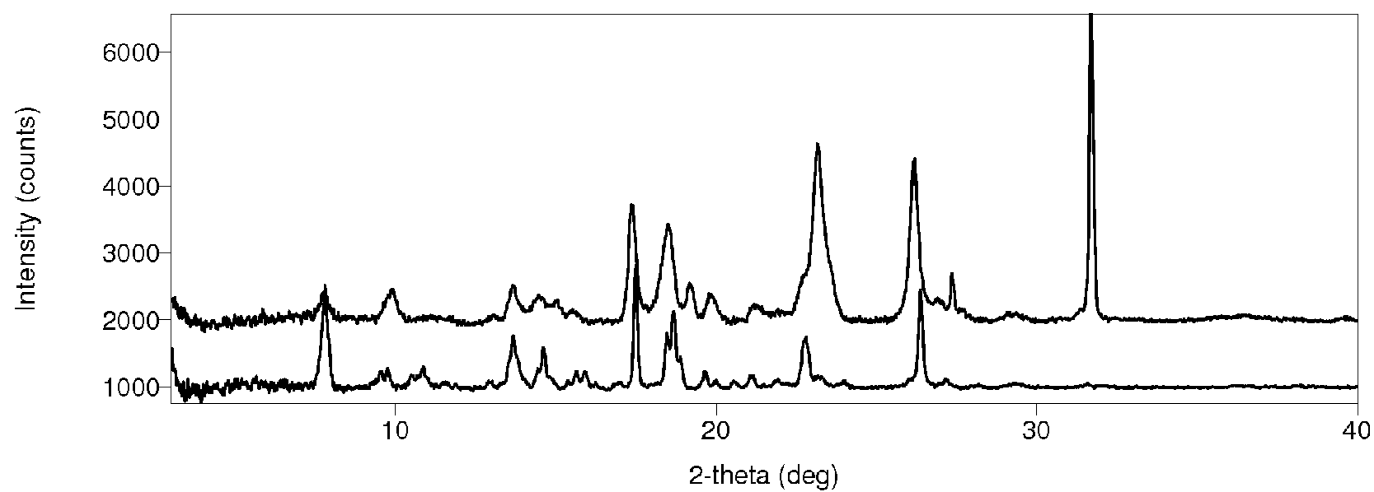
XRPD pattern of crystalline Form B of Compound 3 (bottom) and milling mixture of amorphous and crystalline Form B (top)
