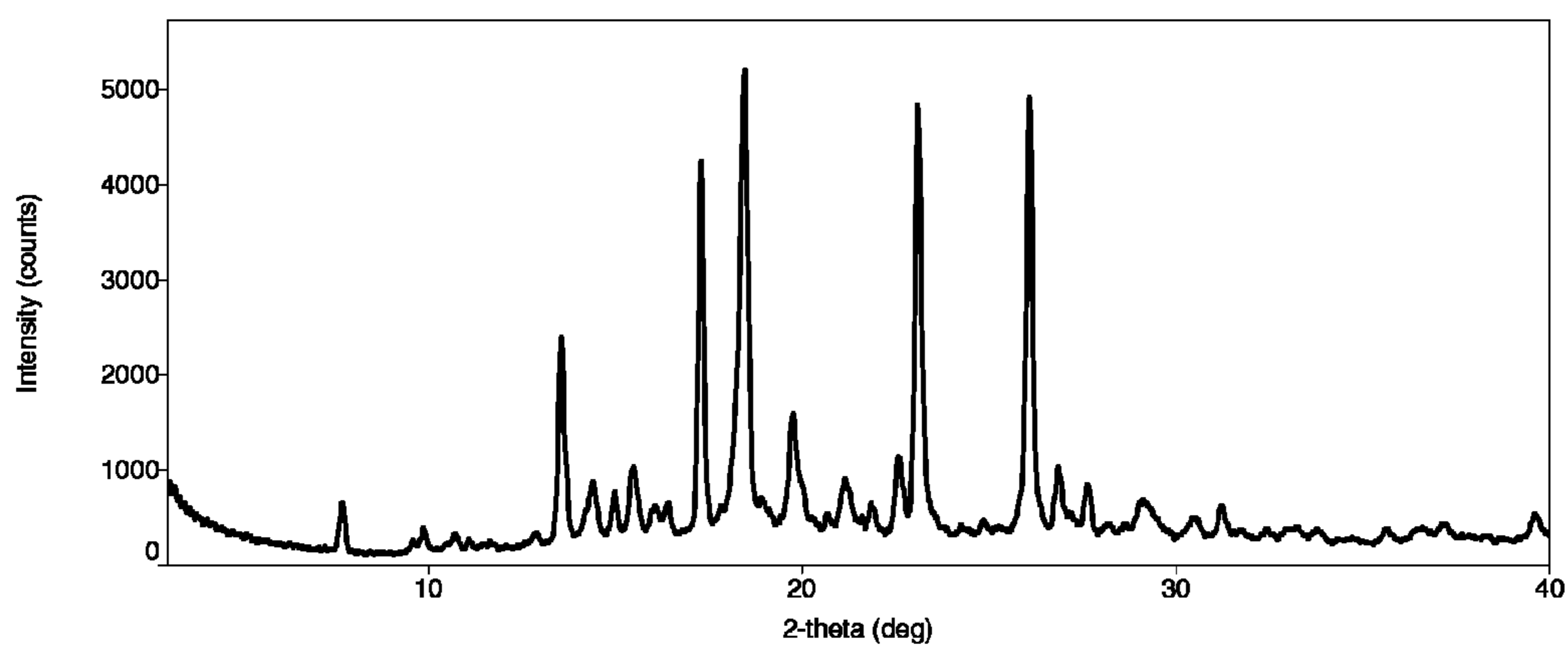
Representative XRPD pattern of crystalline Form B of Compound 3
