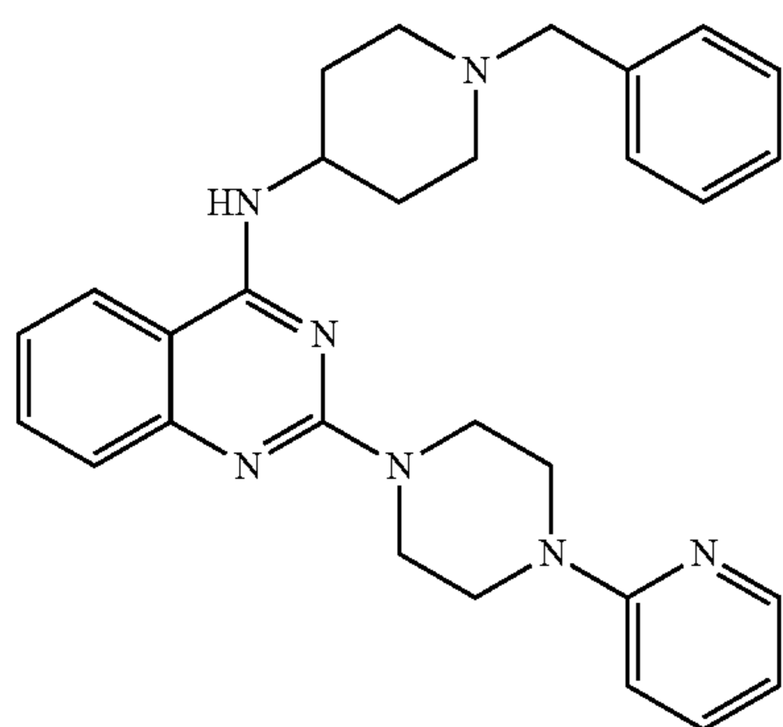
N-(1-benzylpiperidin-4-yl)-2-(4-(pyridin-2-yl)piperazin-1-yl)quinazolin-4-amine
