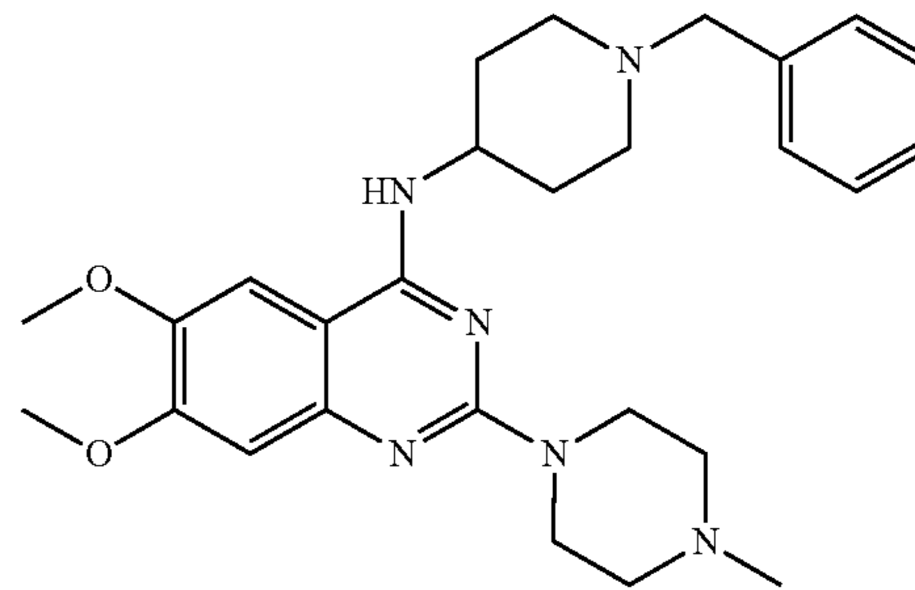
N-(1-benzylpiperidin-4-yl)-6,7-dimethoxy-2-(4-methylpiperazin-1-yl)quinazolin-4-amine
