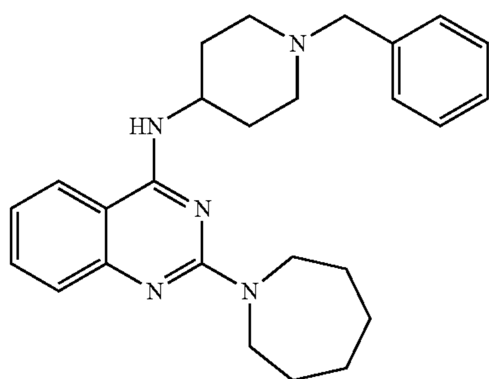
2-(azepan-1-yl)-N-(1-benzylpiperidin-4-yl)quinazolin-4-amine
