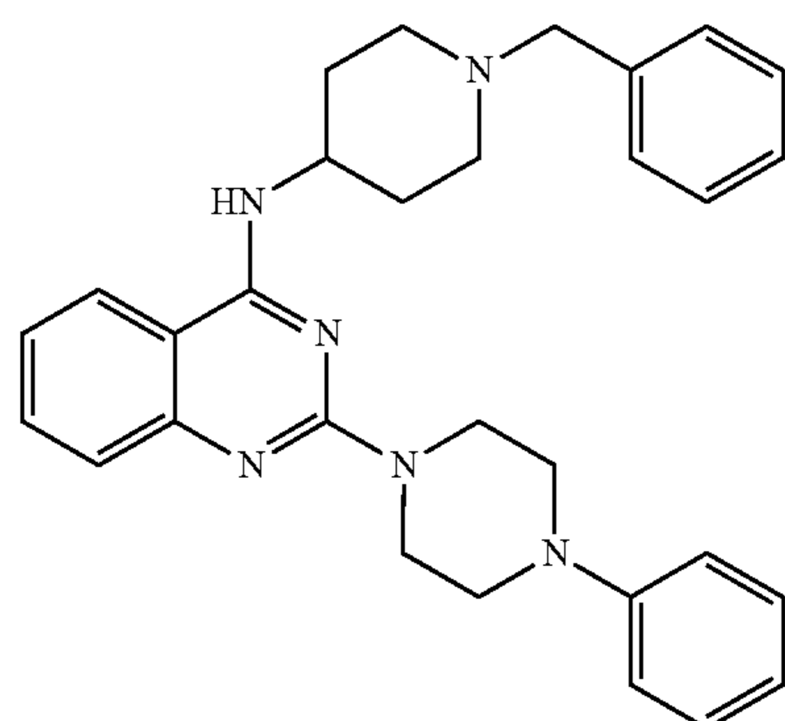
N-(1-benzylpiperidin-4-yl)-2-(4-phenylpiperazin-1-yl)quinazolin-4-amine
