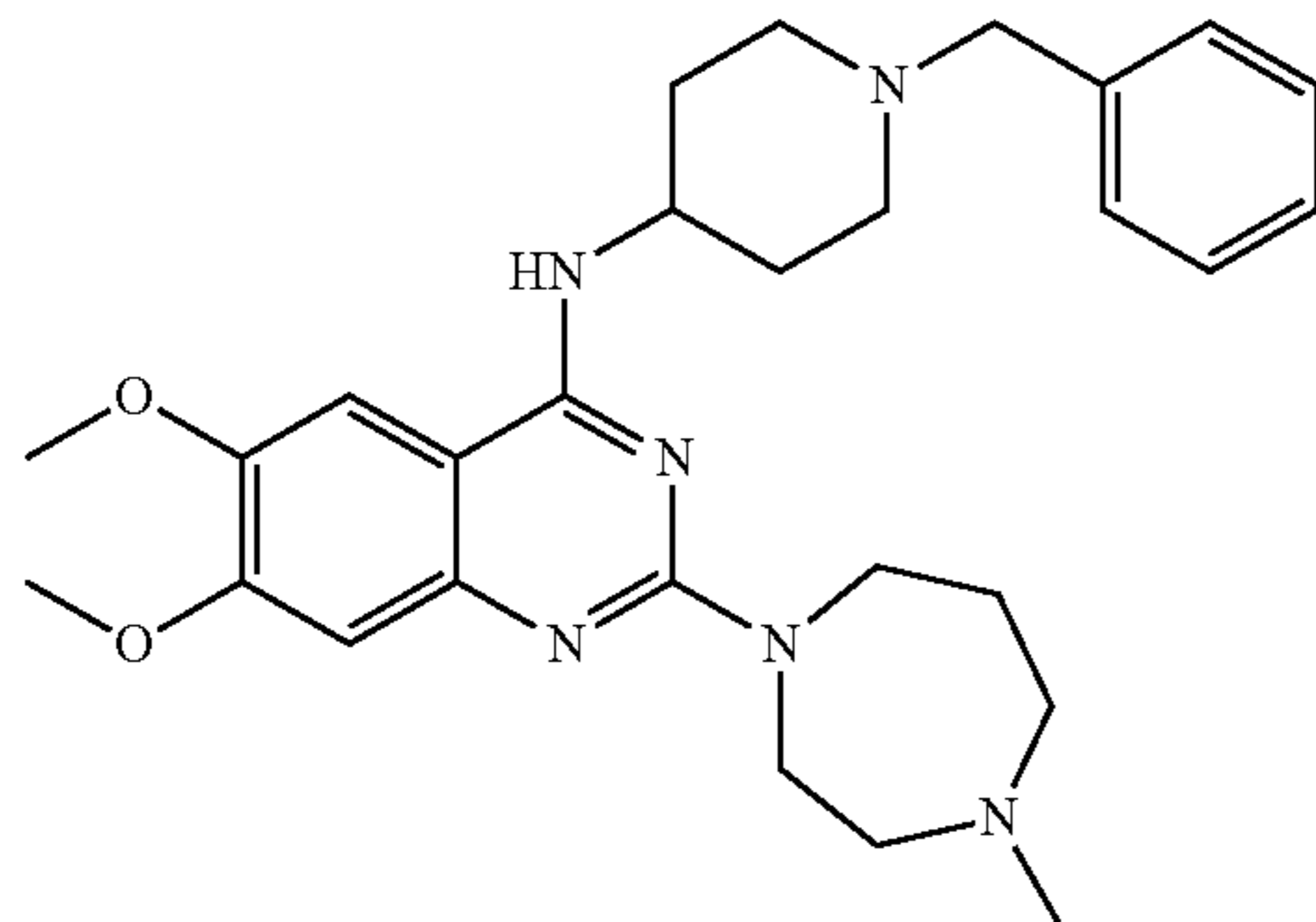
N-(1-benzylpiperidin-4-yl)-6,7-dimethoxy-2-(4-methyl-1,4-diazepan-1-yl)quinazolin-4-amine
