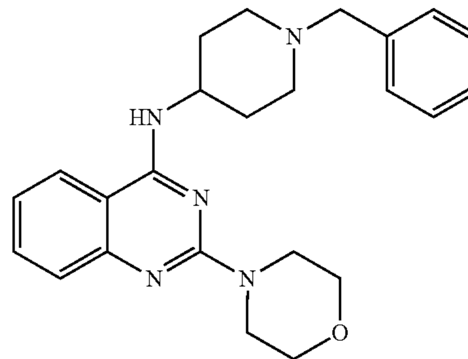
N-(1-benzylpiperidin-4-yl)-2-morpholinoquinazolin-4-amine
