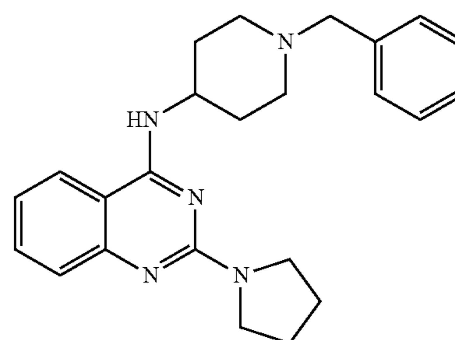
N-(1-benzylpiperidin-4-yl)-2-(pyrrolidin-1-yl)quinazolin-4-amine
