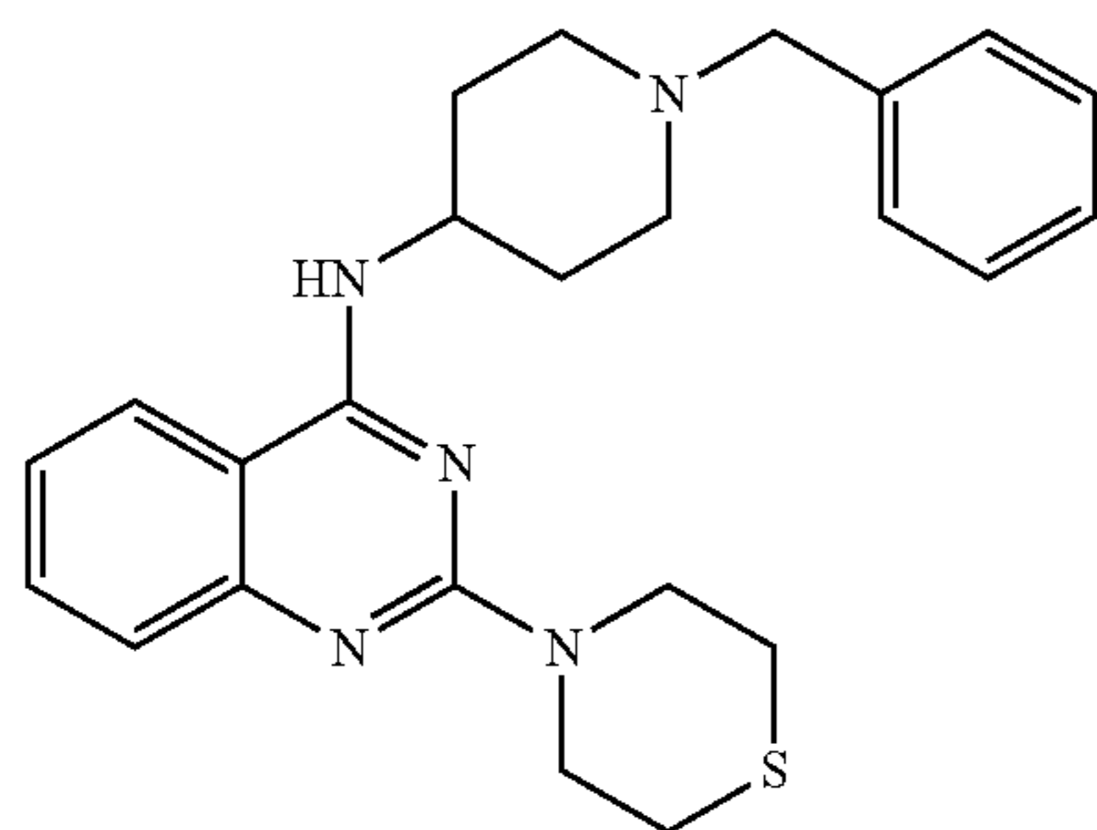
N-(1-benzylpiperidin-4-yl)-2-thiomorpholinoquinazolin-4-amine
