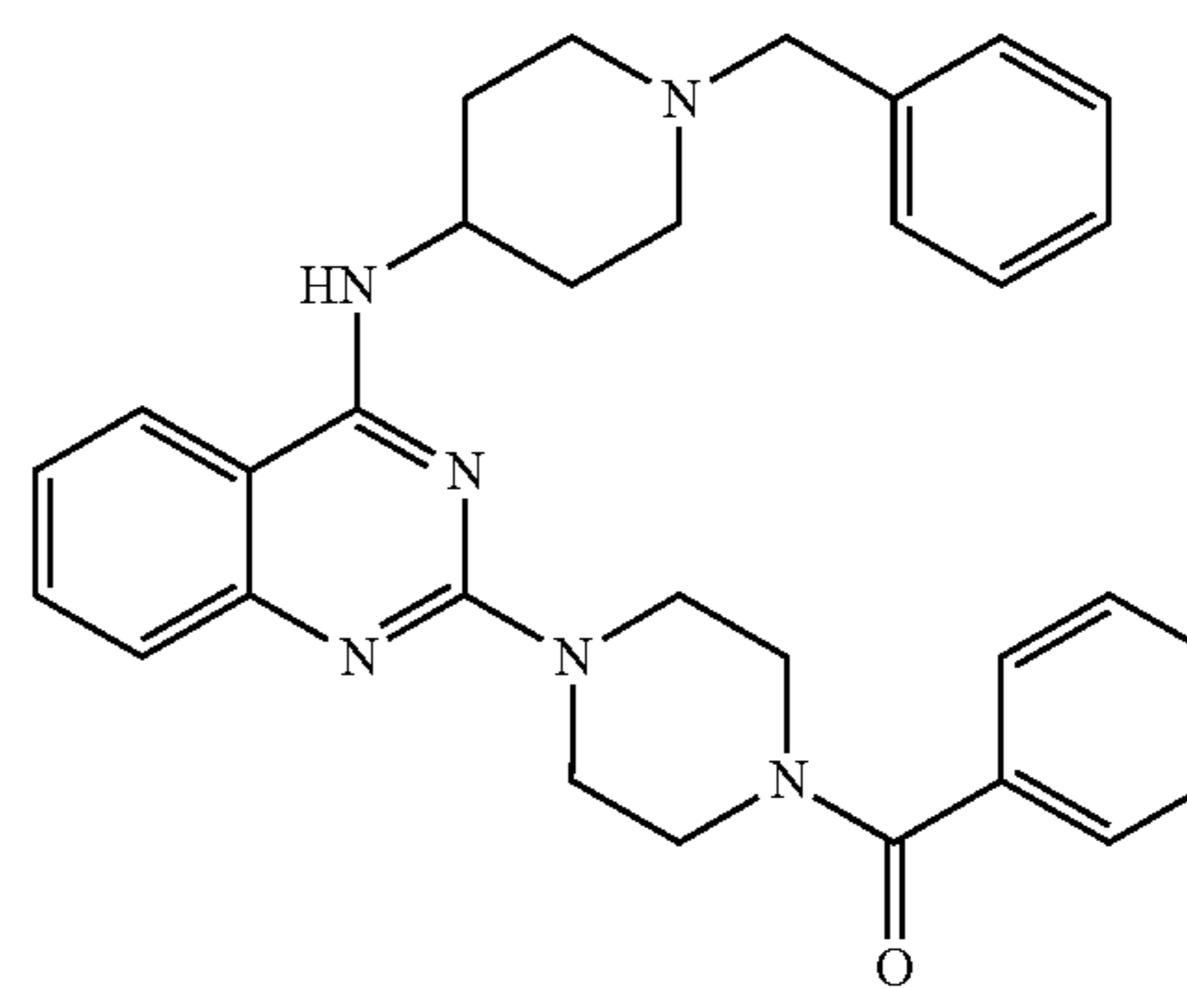
(4-(1-benzylpiperidin-4-ylamino)quinazolin-2-yl)piperazin-1-yl(phenyl)methanone
