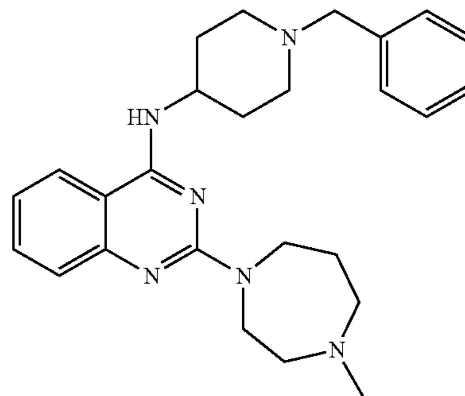
N-(1-benzylpiperidin-4-yl)-2-(4-methyl-1,4-diazepan-1-yl)quinazolin-4-amine
