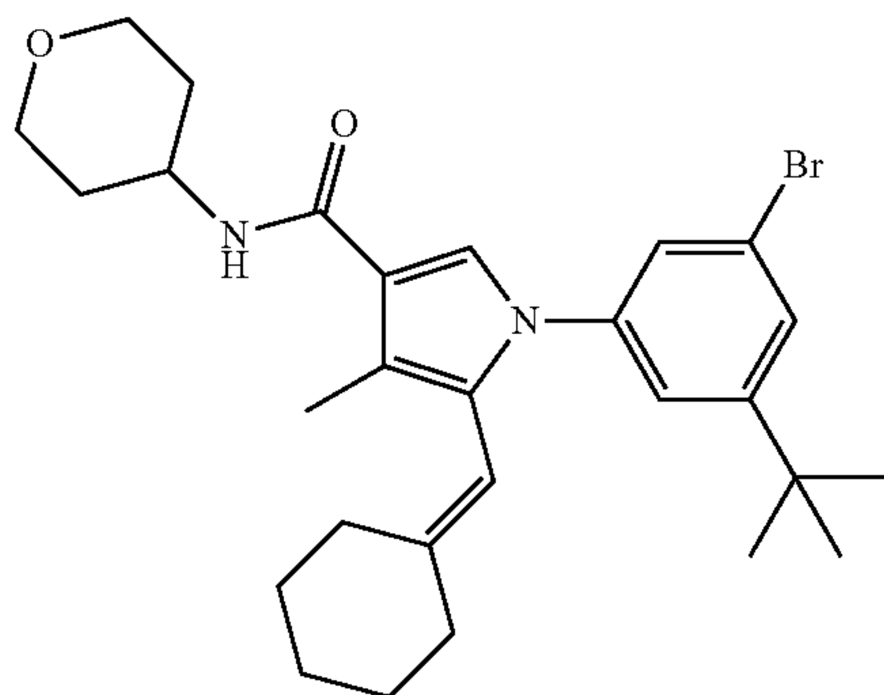
1-(3-Bromo-5-(tert-butyl)phenyl)-5-(cyclohexylidenemethyl)-4-methyl-N-(tetrahydro-2H-pyran-4-yl)-1H-pyrrole-3-carboxamide (2)
