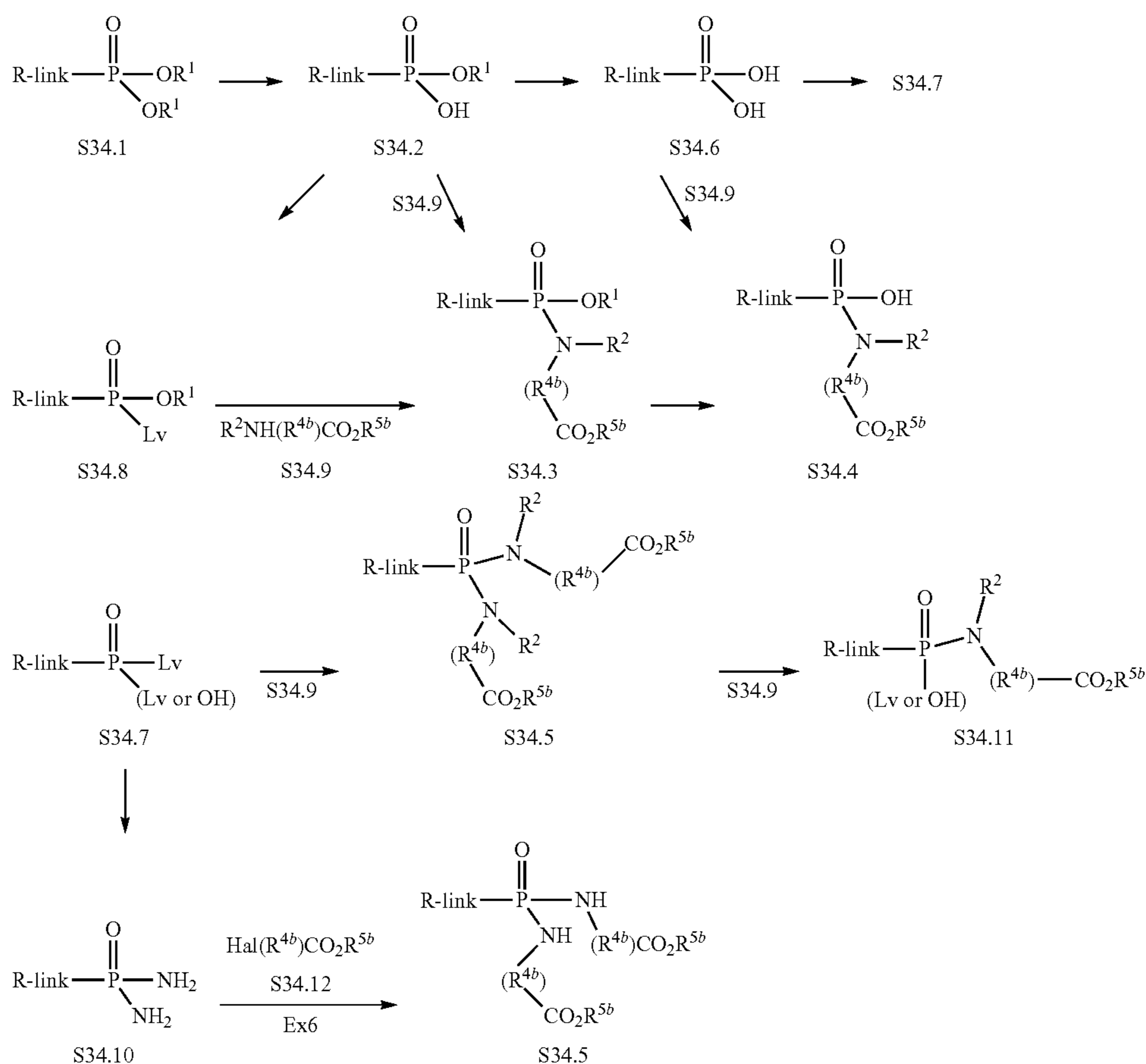
Scheme 34
