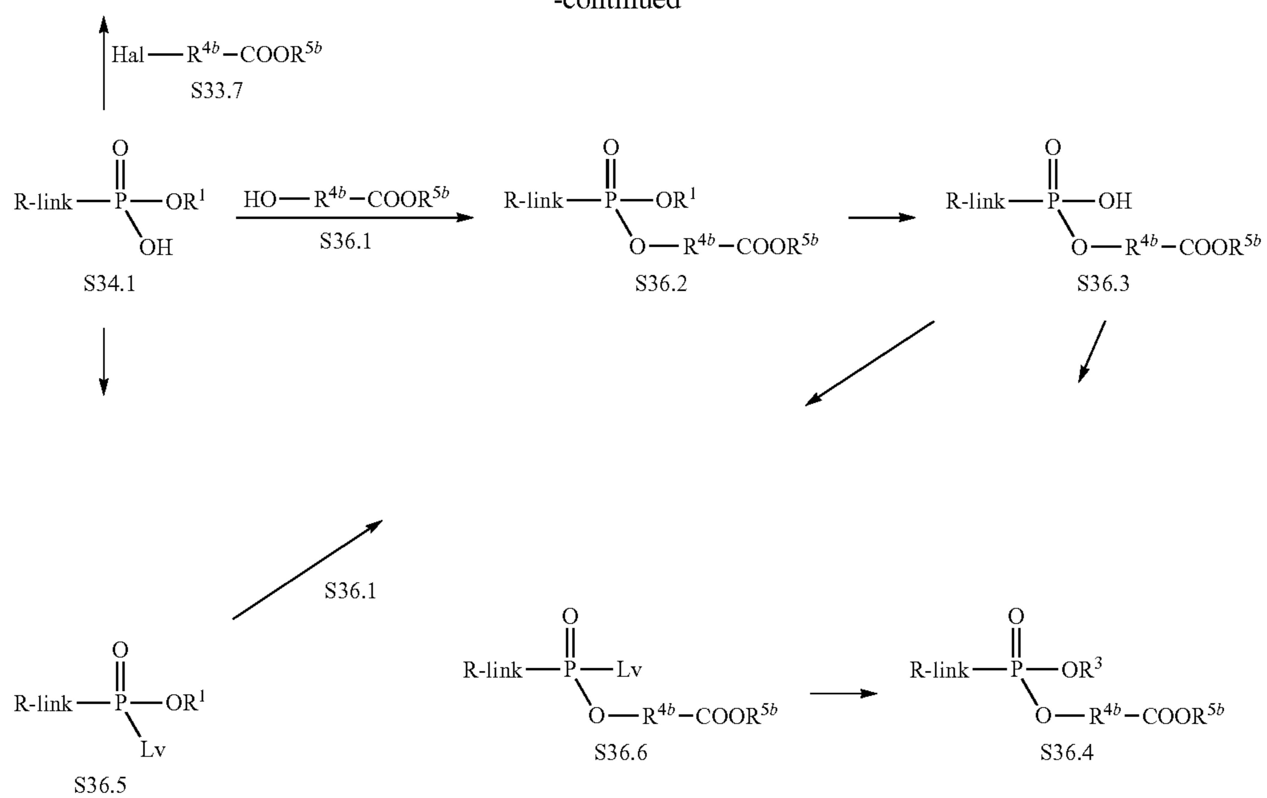
Scheme 36 Example 1
