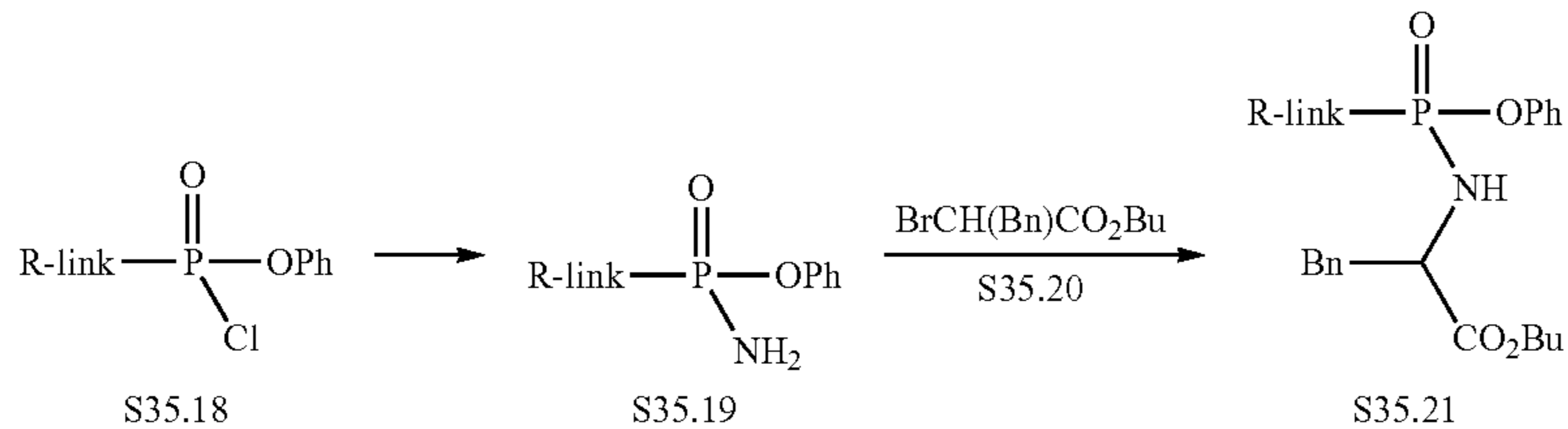
Scheme 35 Example 5
