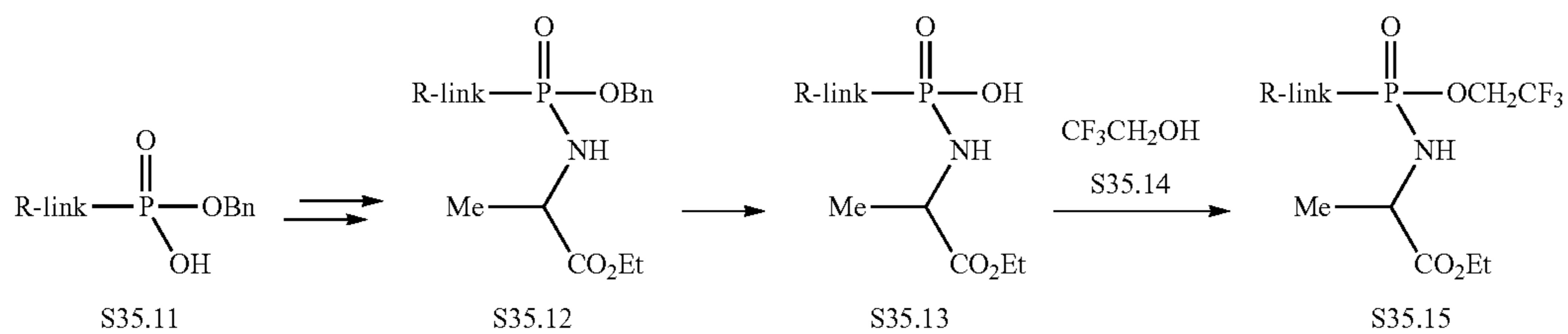
Scheme 35 Example 3
