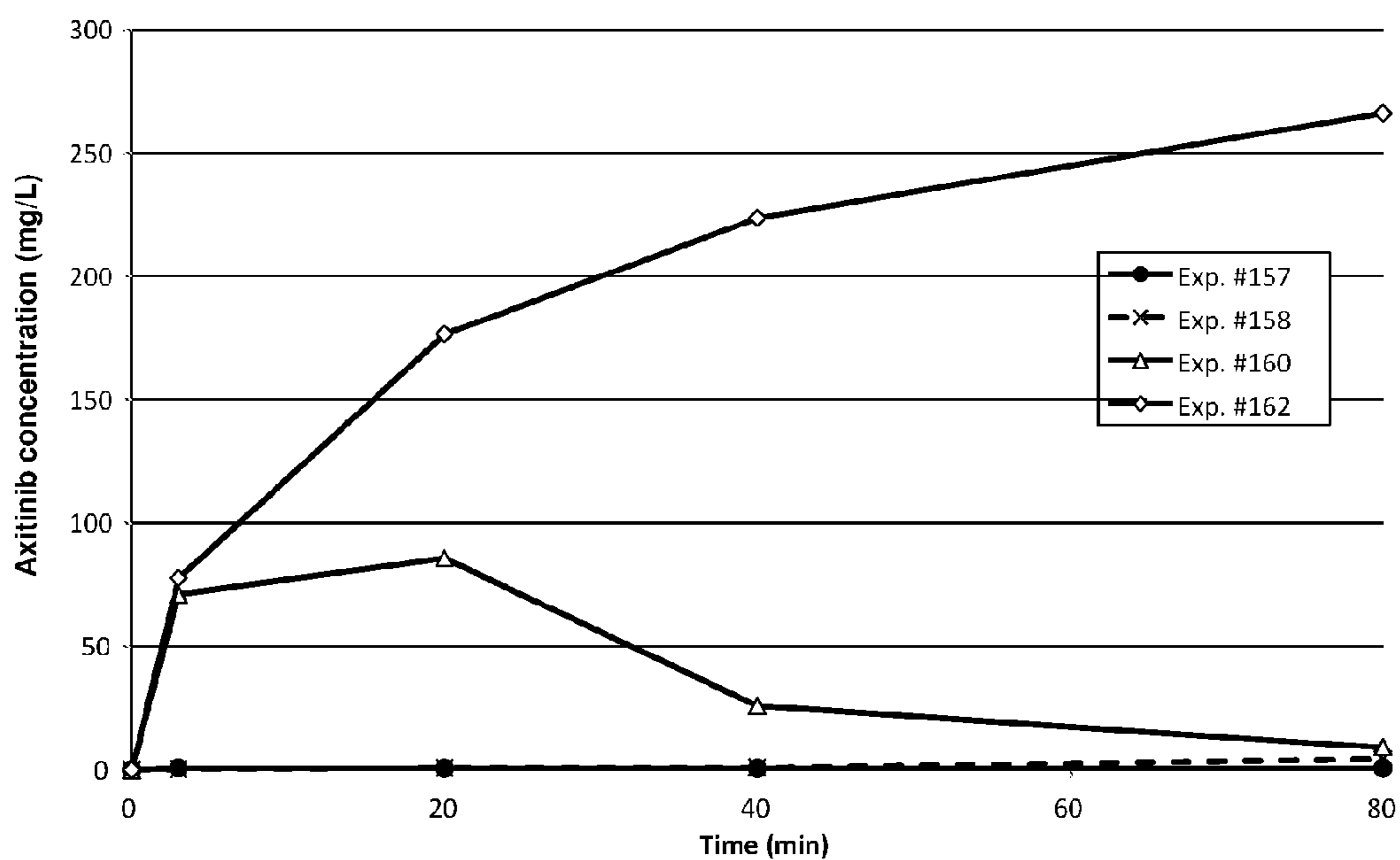
Apparent solubility of different axitinib powders in FaSSIF (pH6.5)
