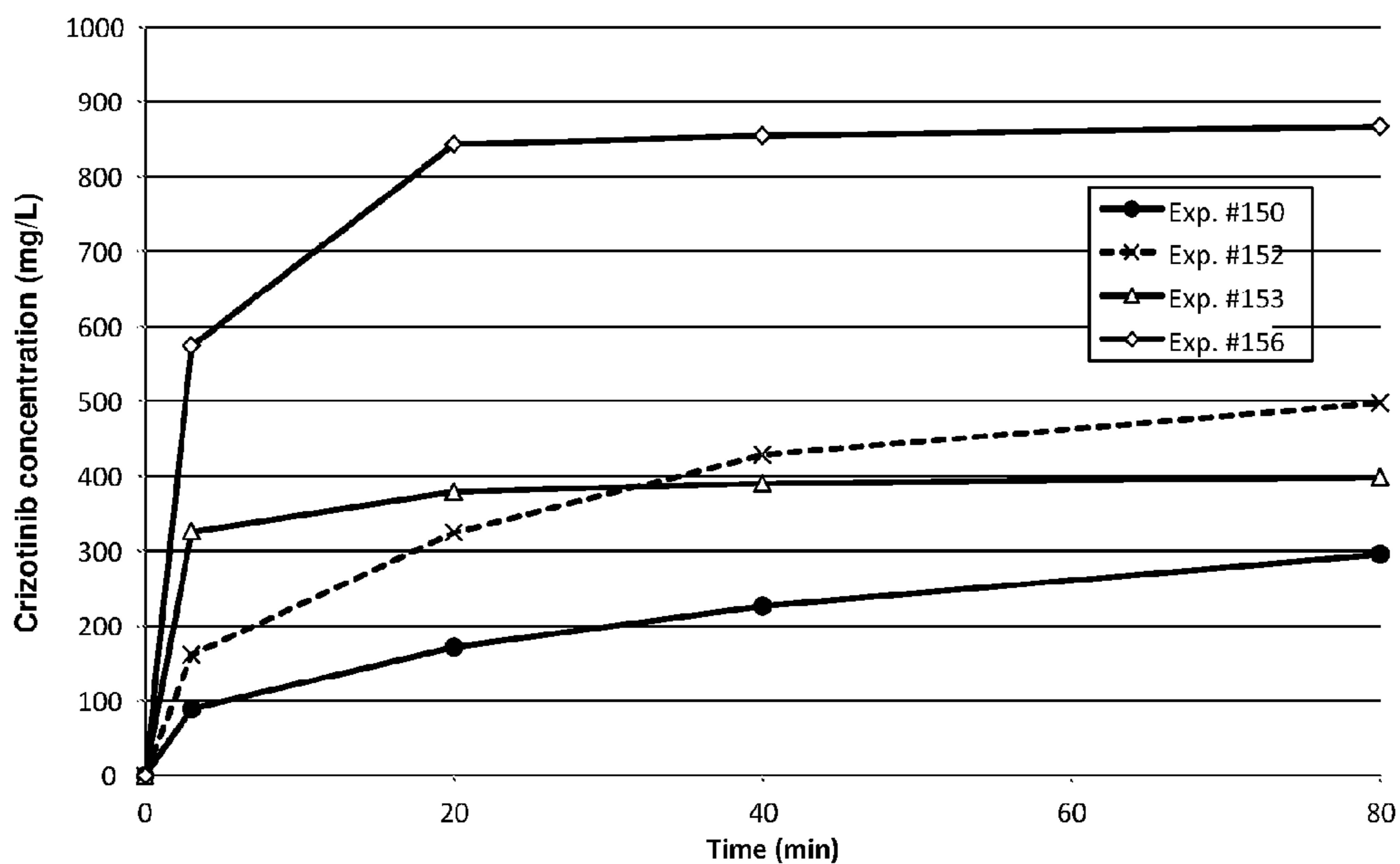
Apparent solubility of different crizotinib powders in FaSSIF (pH 6.5)
