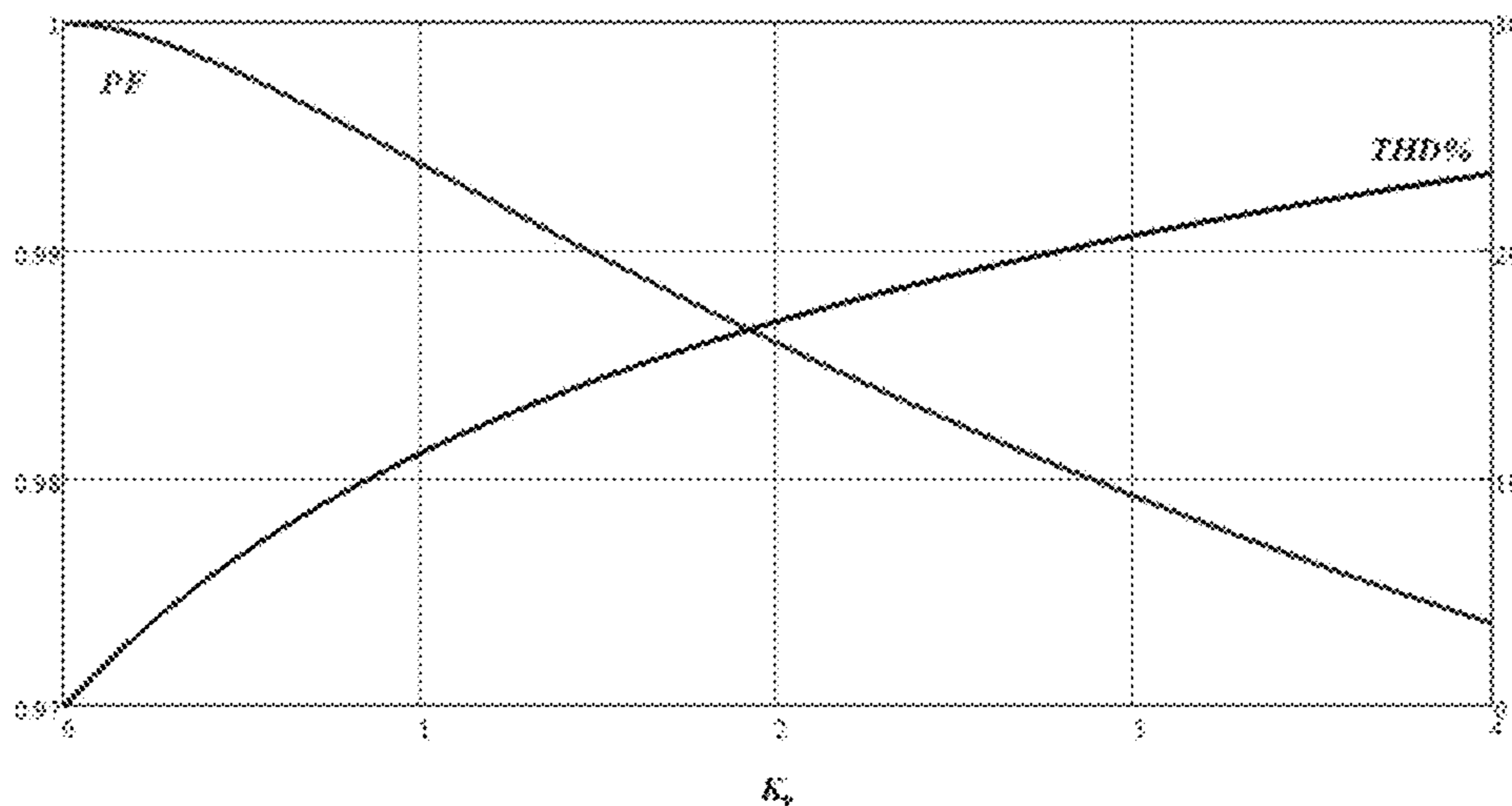
Figure 3 (Prior Art)
