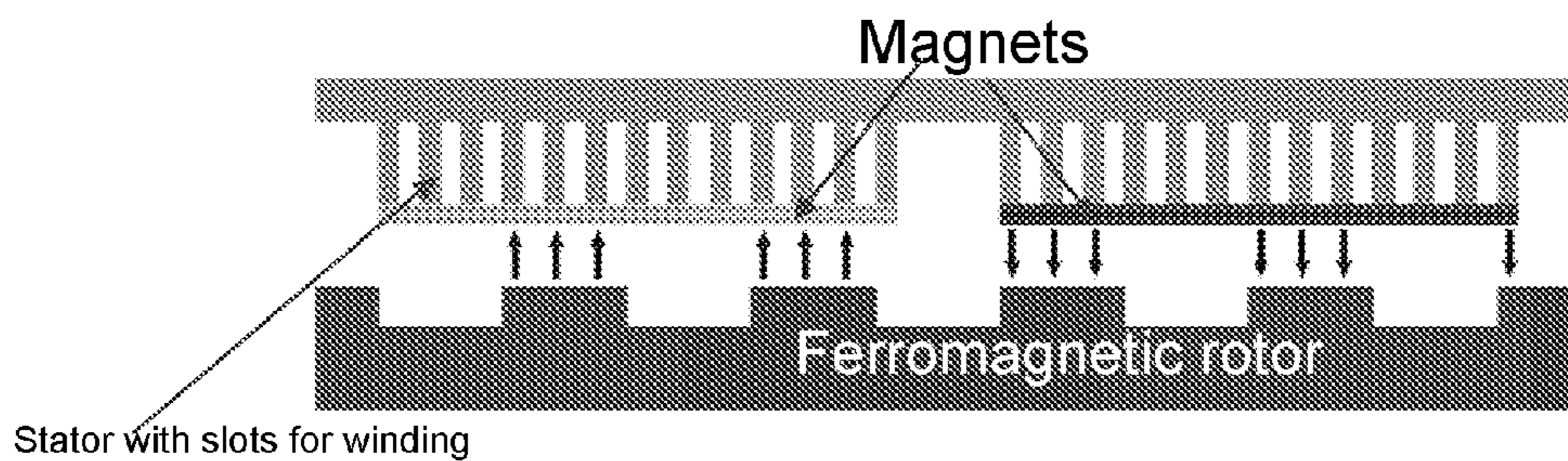
Figure 3. Longitudinal Section of a Permanent Magnet Lorentz Machine
