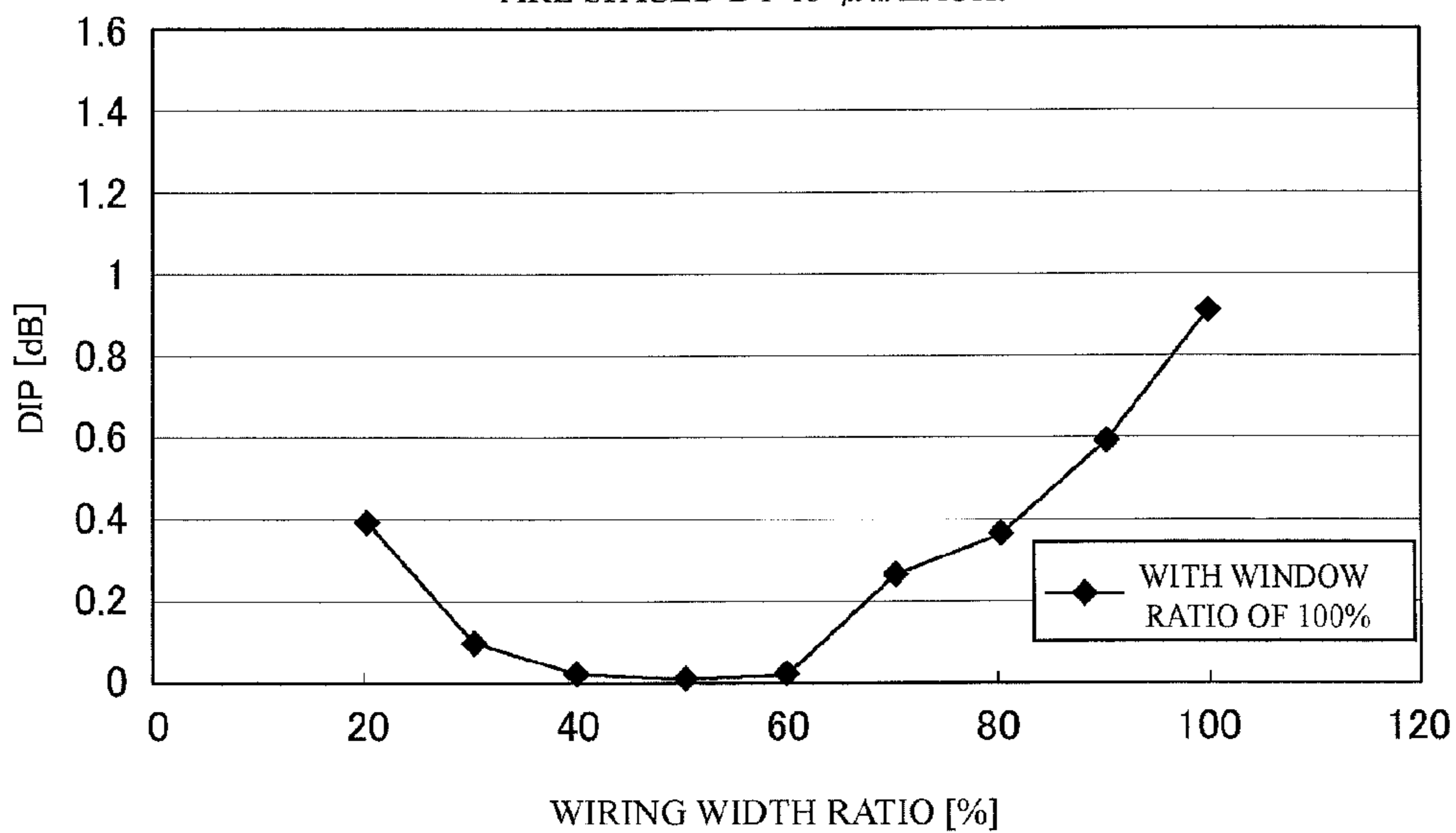
WIRING WIDTH RATIO AND DIP IN TRANSMISSION LOSS SECTIONS 45BA AND 43BA AND WIRES 27 AND 29 ARE SPACED BY 15 \mu\text{m} EACH.
