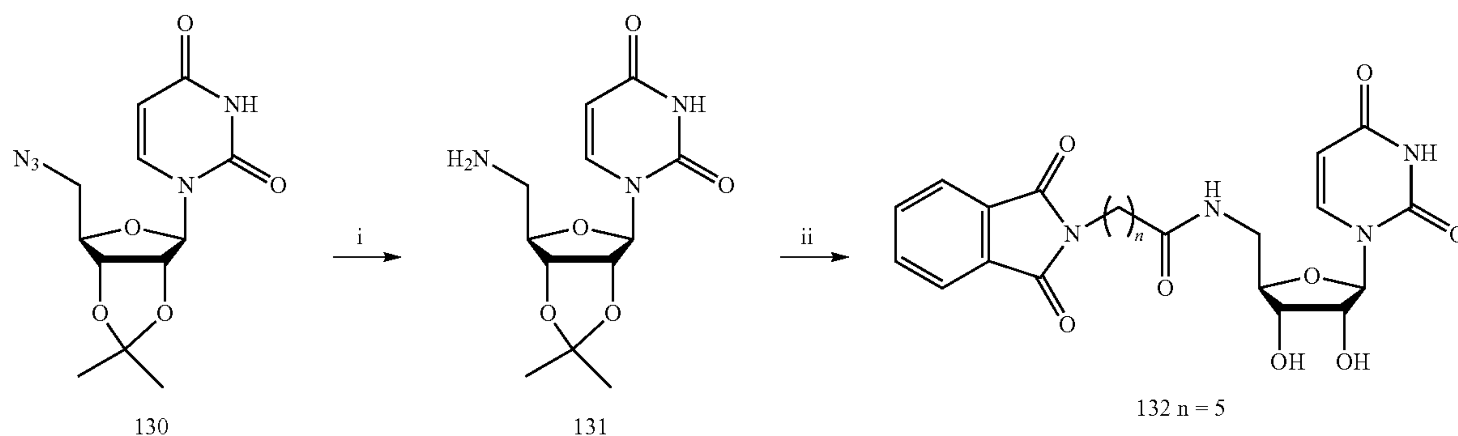
Scheme 6 a
