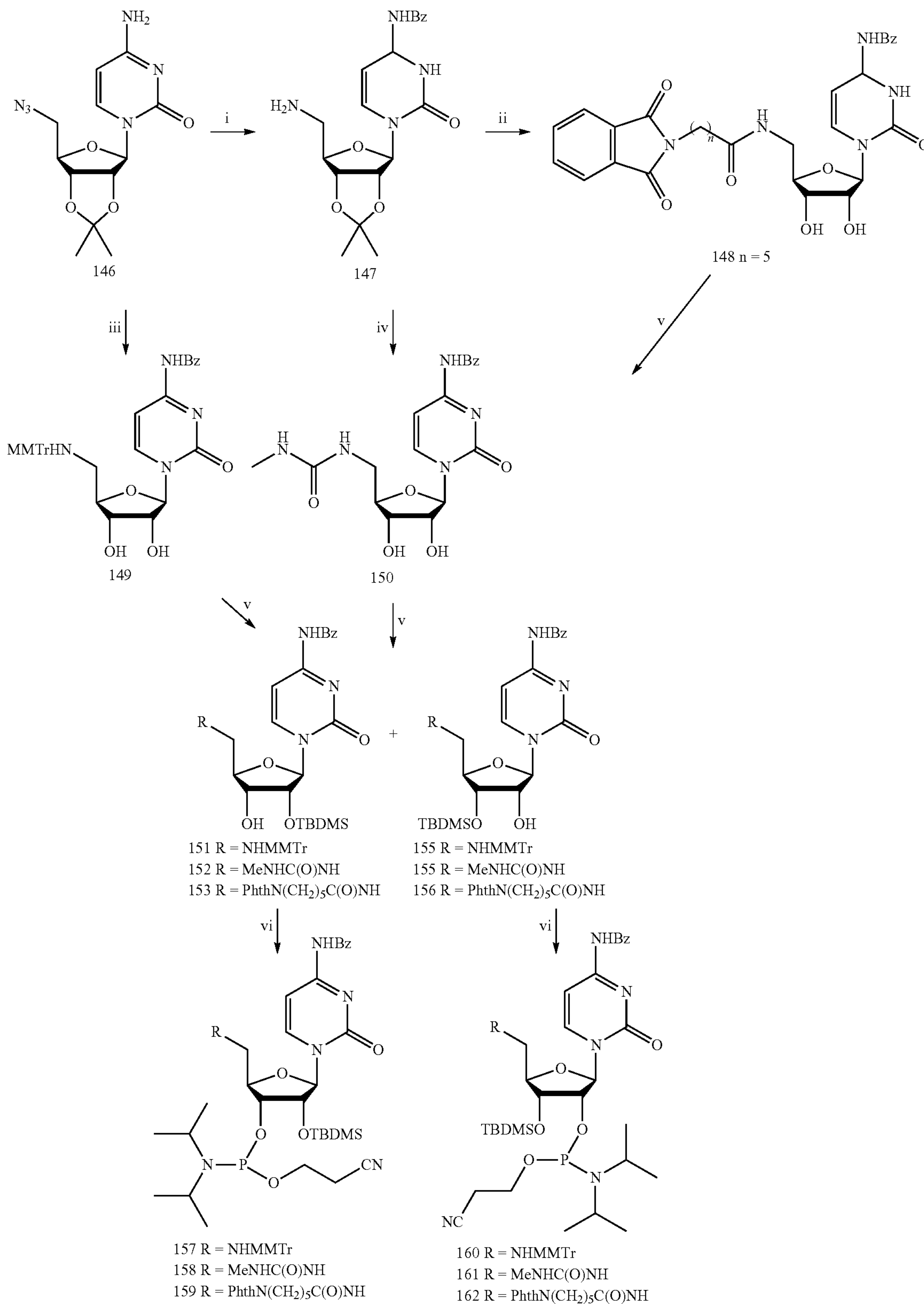
Scheme 7 a
