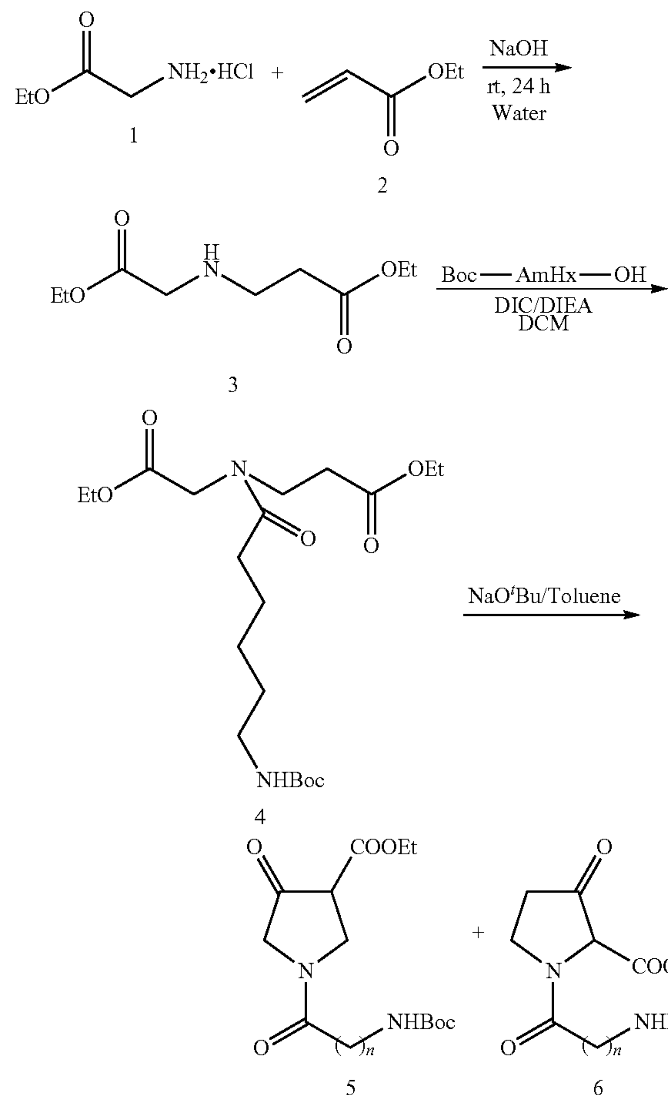
Scheme 1. Synthesis of cis-(-(3S,4R)-pyrrolidine diol
