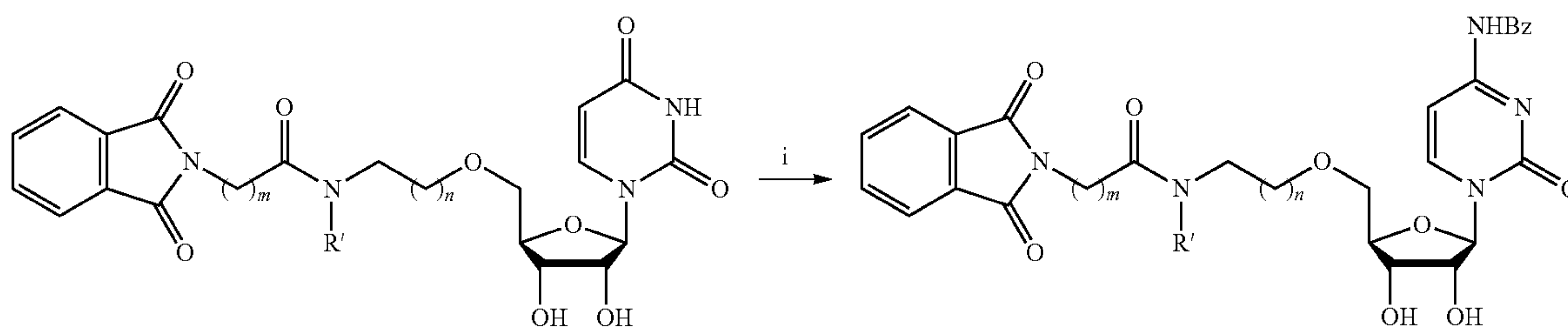
Scheme 5 a
