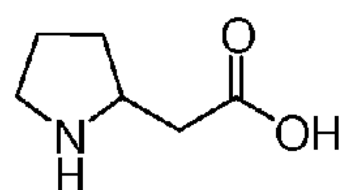
\beta -Homoproline
