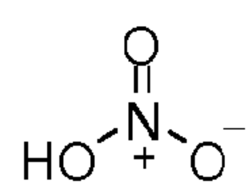
Nitrate
