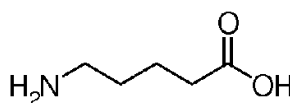
5-Aminovaleric acid
