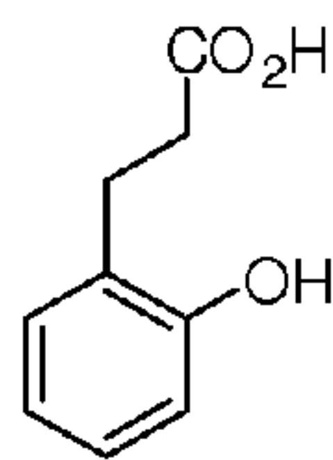
Melilotic acid
