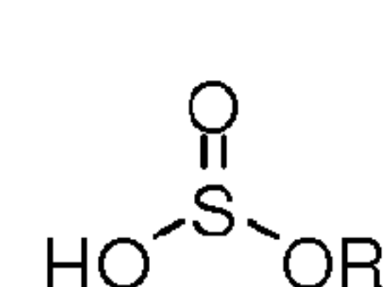
Sulfite
