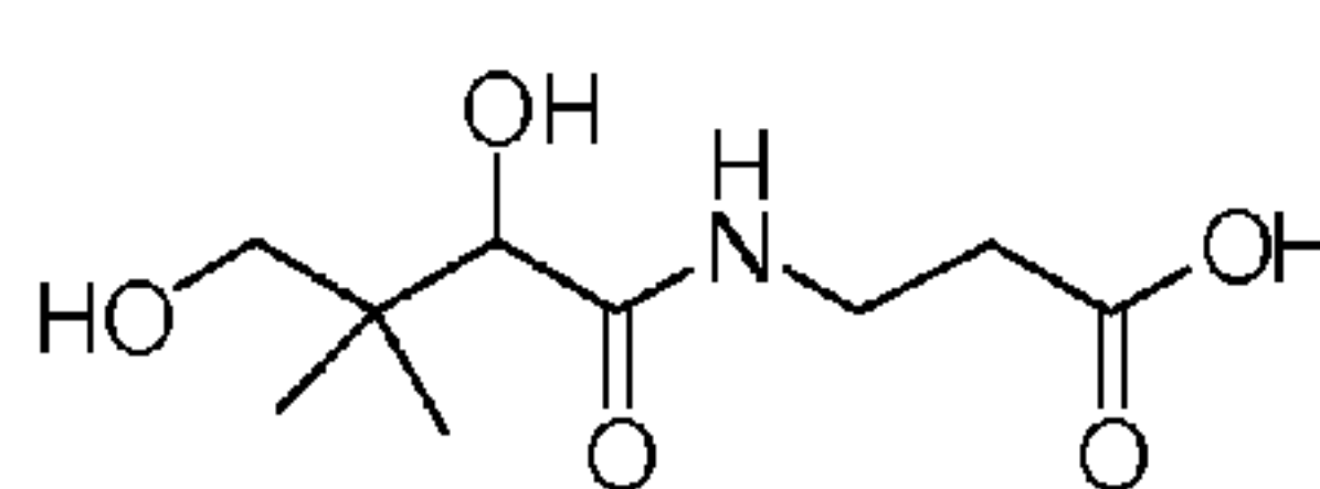
Pantothenic acid
