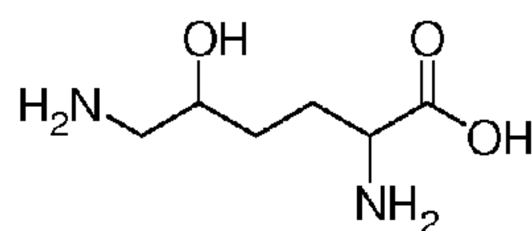
5-Hydroxylysine
