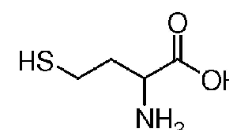
Homocysteine
