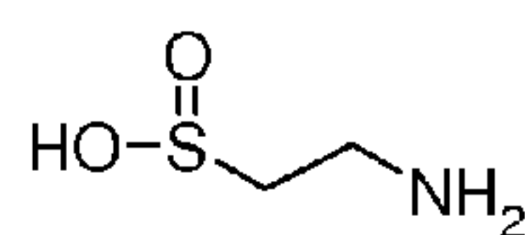
Hypotaurine
