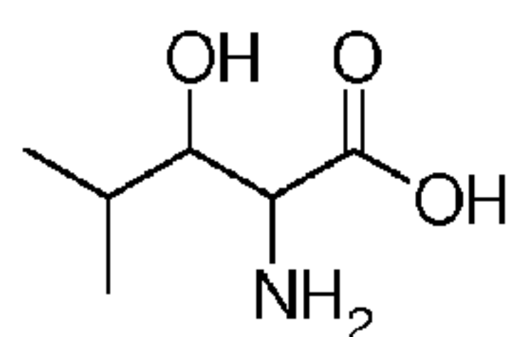
3-Hydroxyisoleucine
