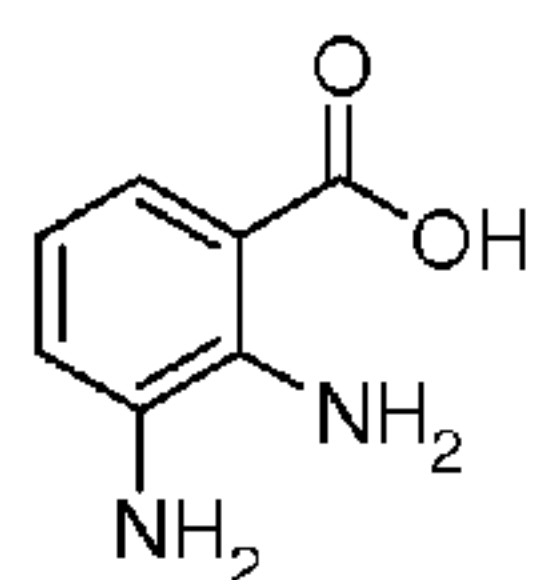
2,3-Diaminobenzoic acid
