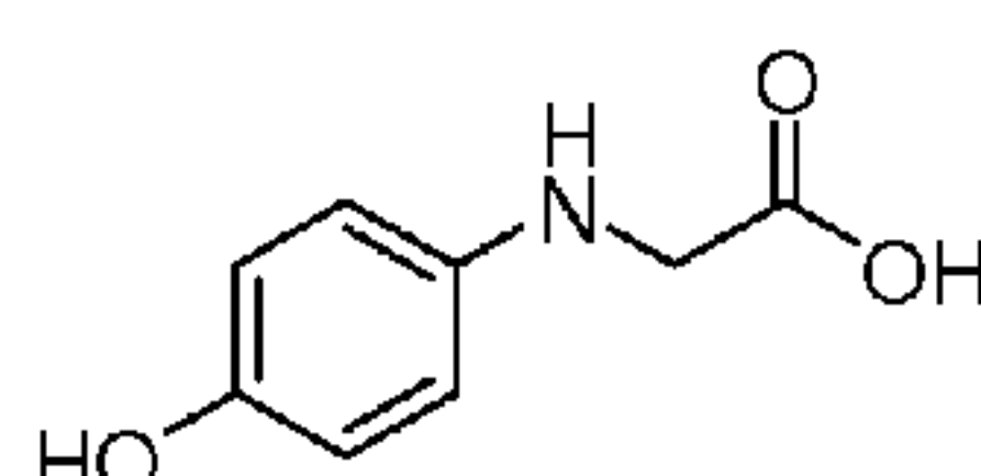
N -(4-Hydroxyphenyl)glycine
