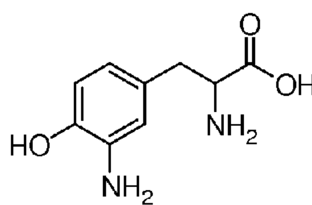
3-Amino-tyrosine
