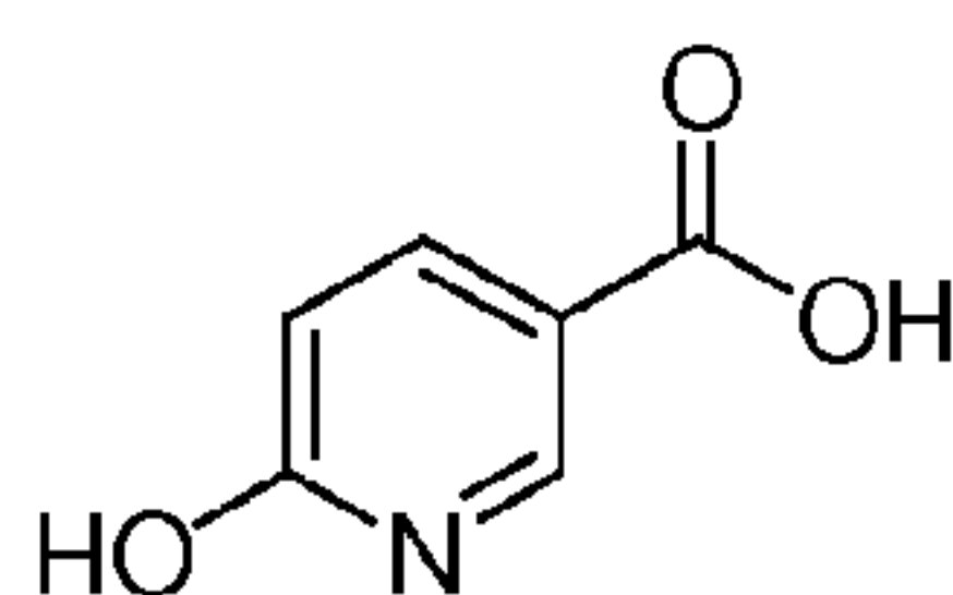
6-hydroxynicotinic acid
