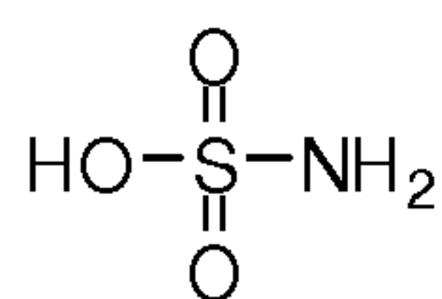
Sulfamate
