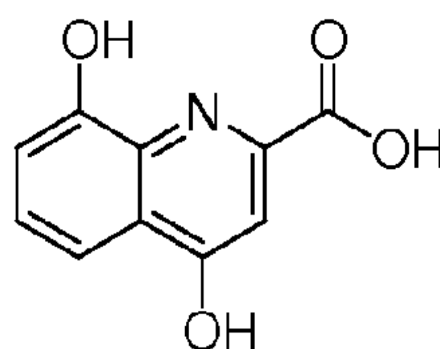
xanthurenic acid
