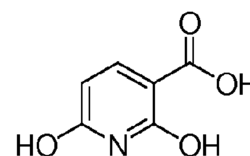
2,6-dihydroxynicotinic acid
