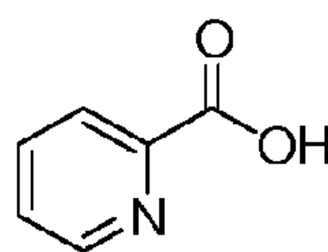
picolinic acid
