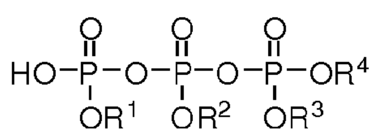
Triphosphate
