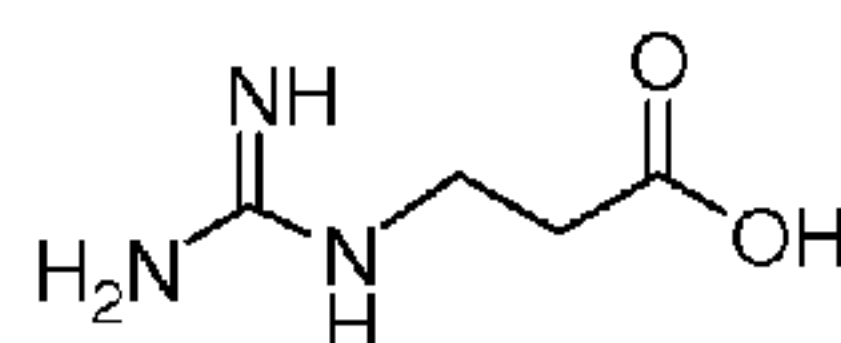
3-Guanidinopropionic acid
