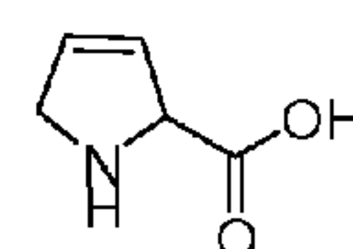
3,4-Dehydro-proline
