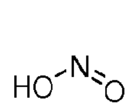
Nitrite
