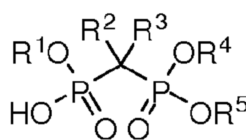
Biphosphonate
