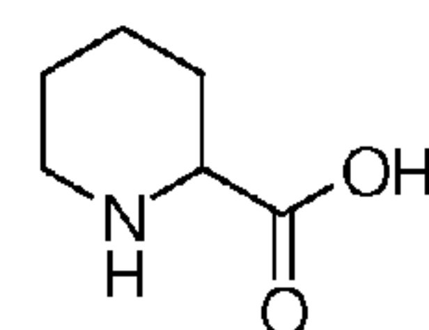
Pipecolic acid
