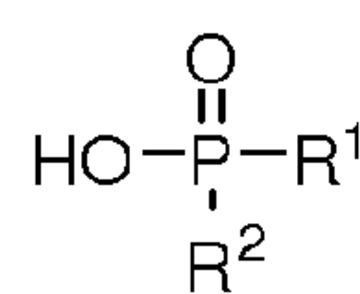
Phosphinate
