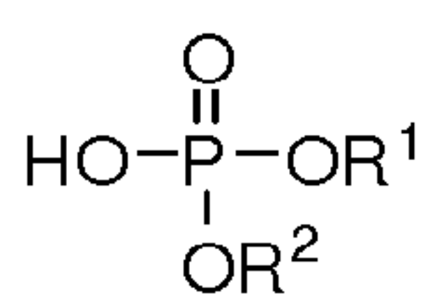
Phosphate
