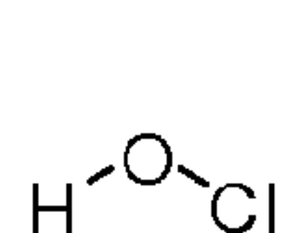
Hypochlorite
