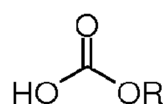
Carbonate
