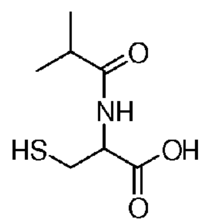
N-Isobutyryl-cysteine
