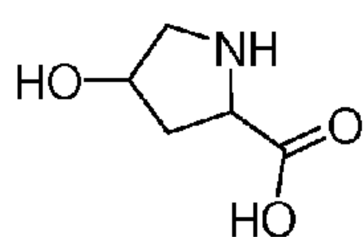
4-Hydroxyproline
