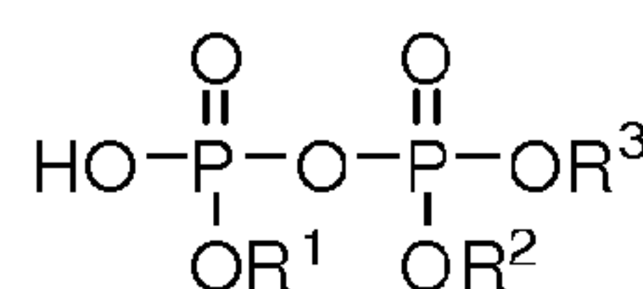
Diphosphate
