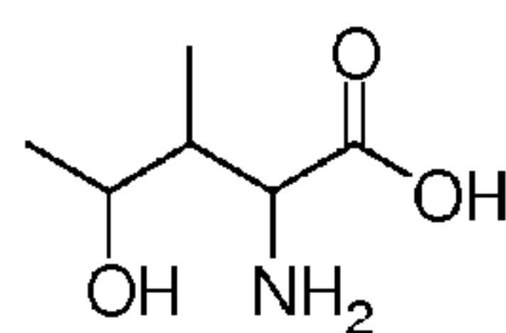
4-Hydroxyisoleucine
