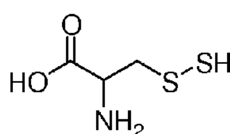
Thiocysteine
