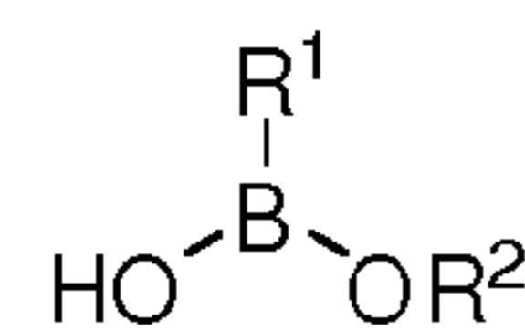
Boronate
