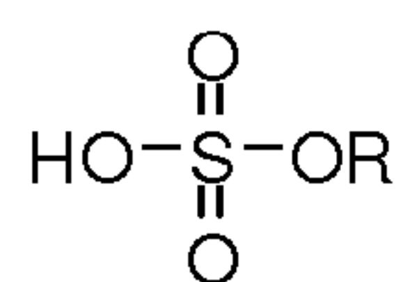
Sulfate
