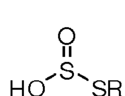
Thiosulfite
