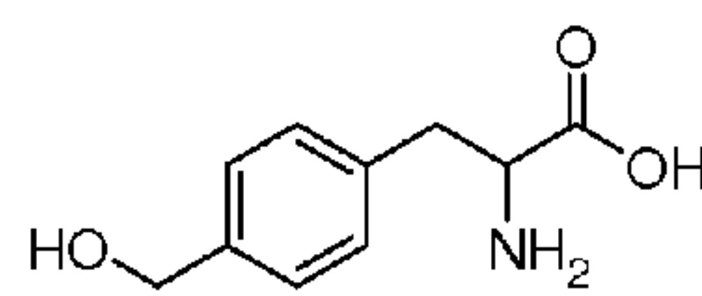
4-(Hydroxymethyl)-phenylalanine
