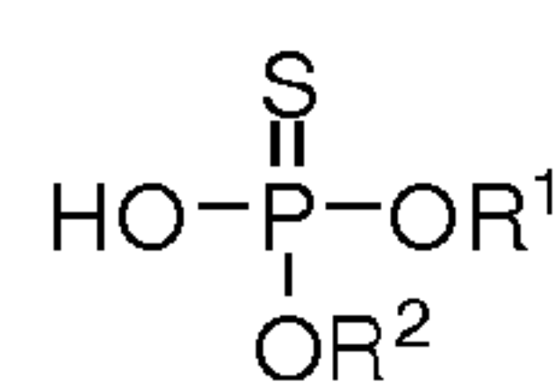
Phosphorothioate
