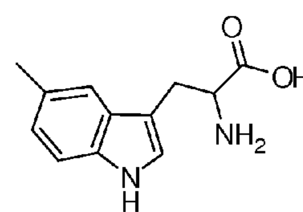
5-Methyl-tryptophan
