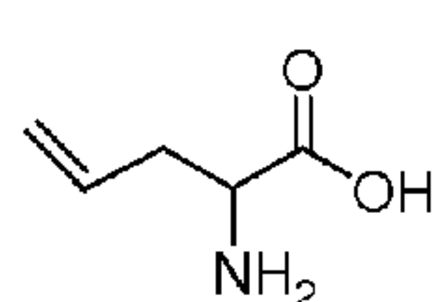
Allylglycine
