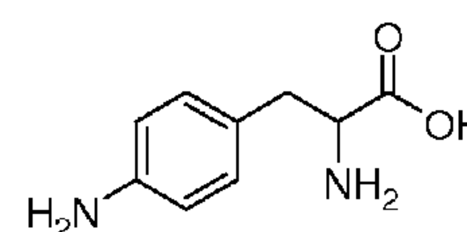
4-Amino-phenylalanine
