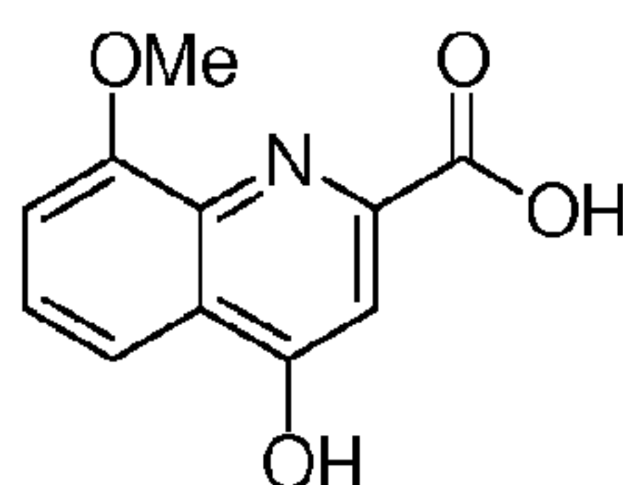
8-methoxykynurenic acid
