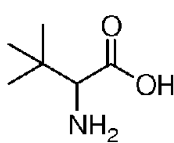
tert-Leucine
