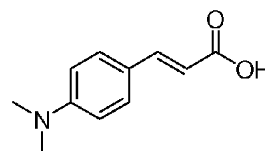
4-(Dimethylamino)cinnamic acid
