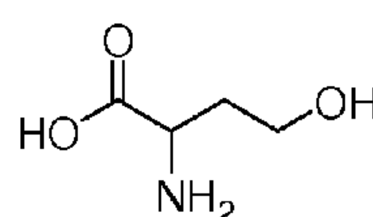
Homoserine
