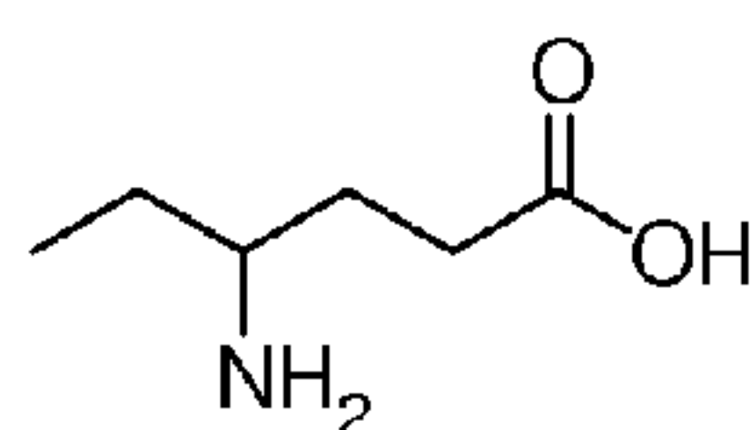
3-Aminopentanoic acid
