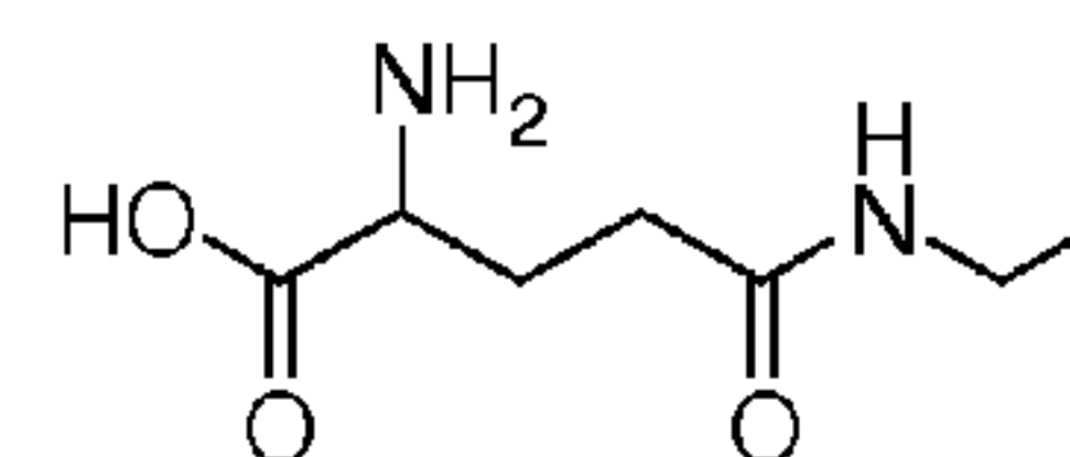
Theanine
