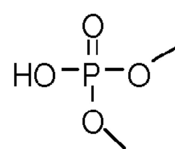
Dimethylphosphate
