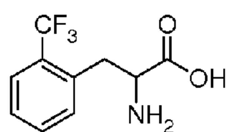
2-(Trifluoromethyl)-phenylalanine
