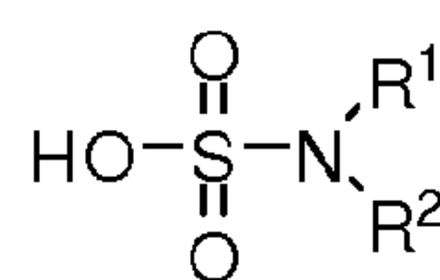
Sulfamate
