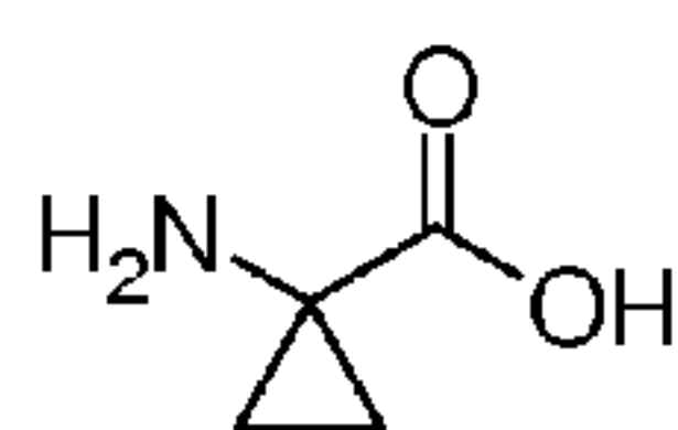
1-Aminocyclopropyl-1-carboxylic acid
