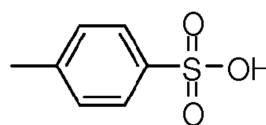
Tosylate
