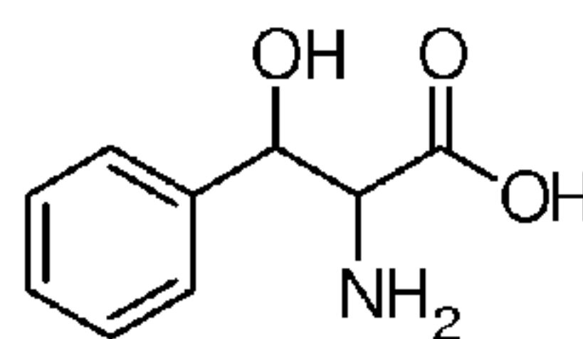
3-Phenylserine
