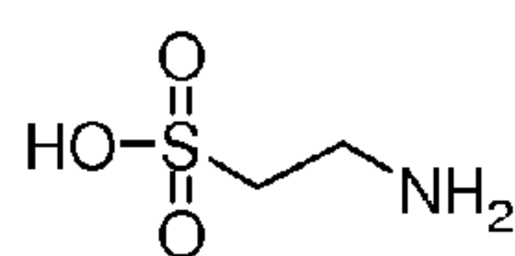
Taurine
