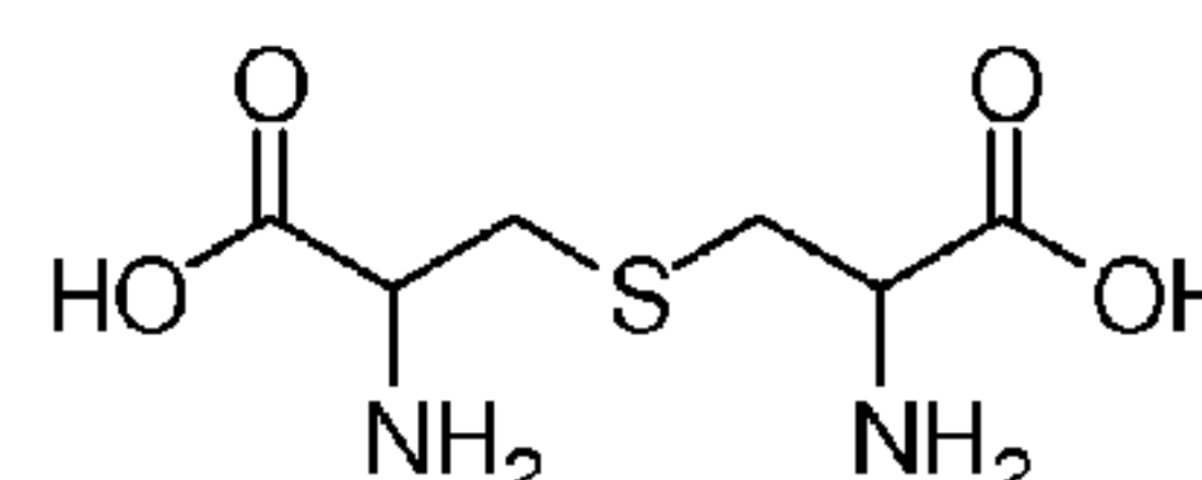
Lanthionine
