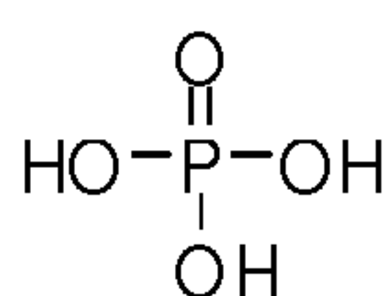
Phosphate
