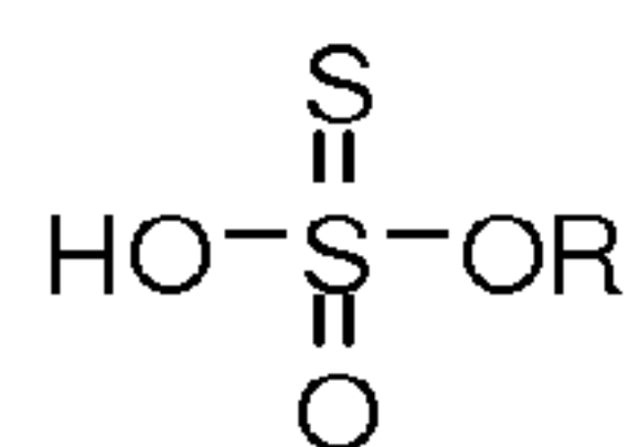
Thiosulfate
