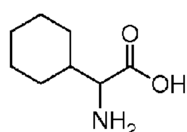
Cyclohexylglycine
