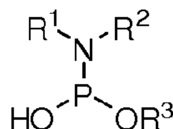
Phosphoramidite
