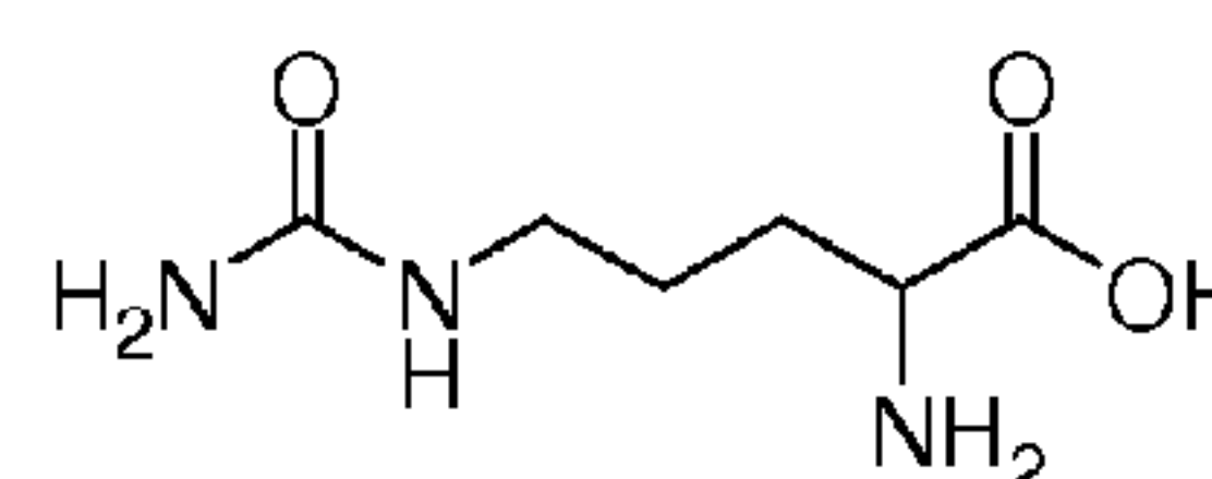
Citrulline
