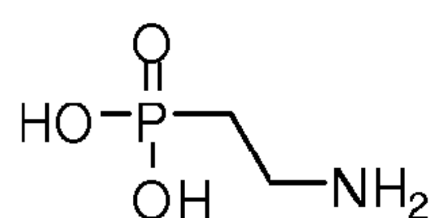
2-Aminoethyl- phosphonate
