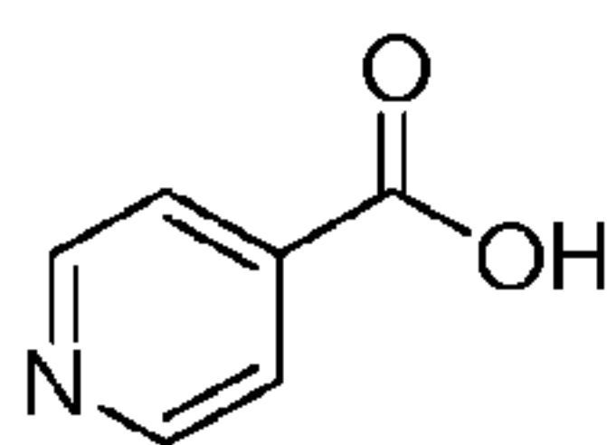
isonicotinic acid
