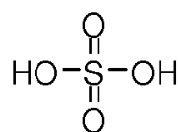
Sulfate
