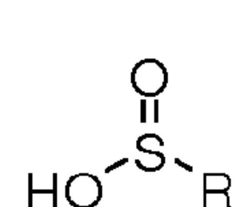
Sulfinate
