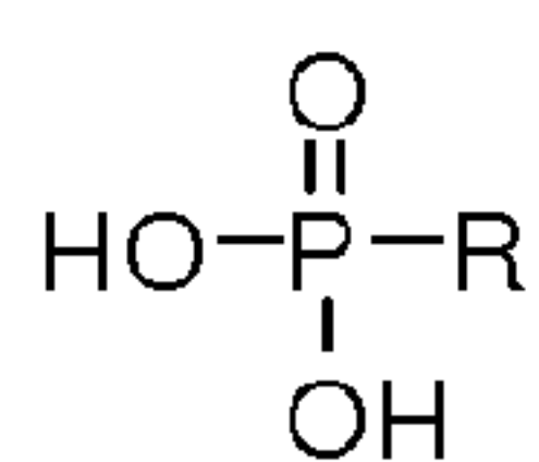
Phosphonate
