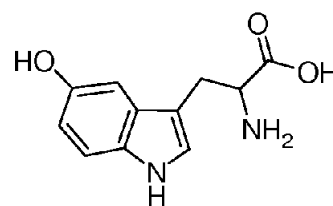
5-Hydroxy-tryptophan
