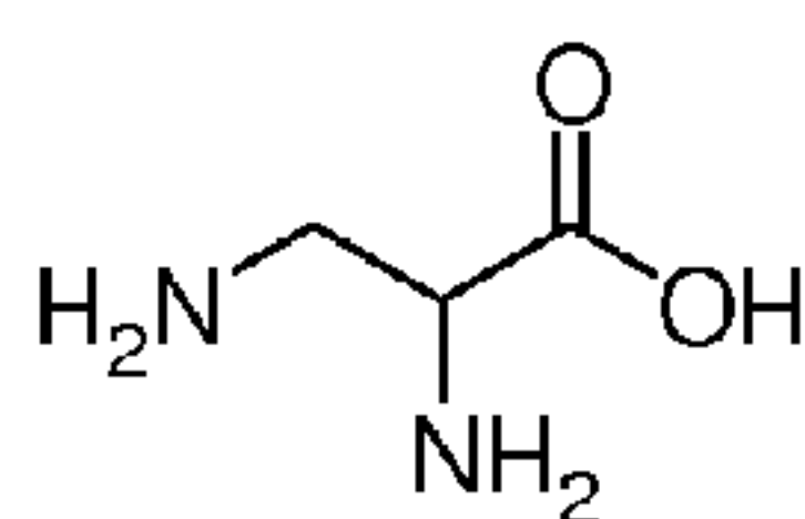
2,3-Diaminopropionic Acid
