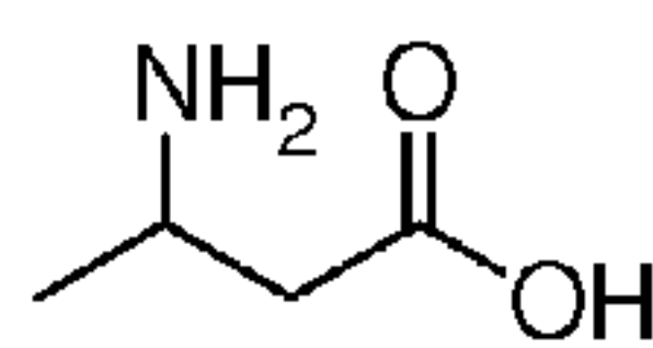
\beta -Homoalanine
