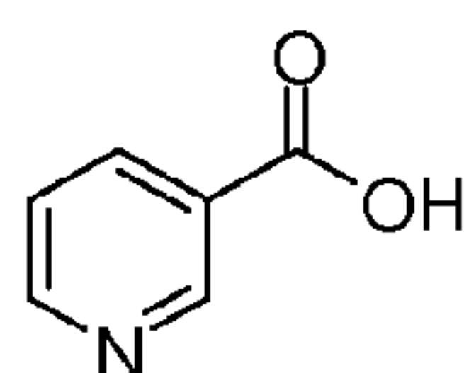
nicotinic acid
