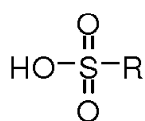
Sulfonate
