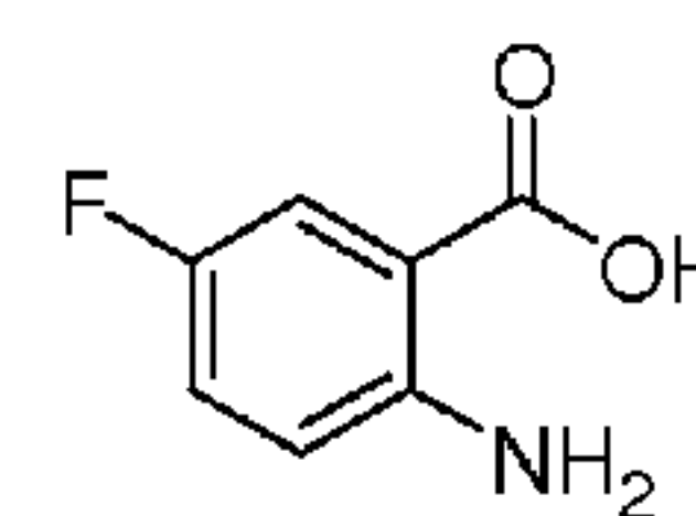
2-Amino-5-fluorobenzoic acid
