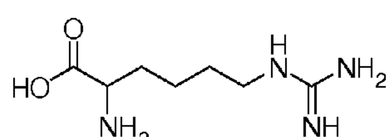
Homoarginine
