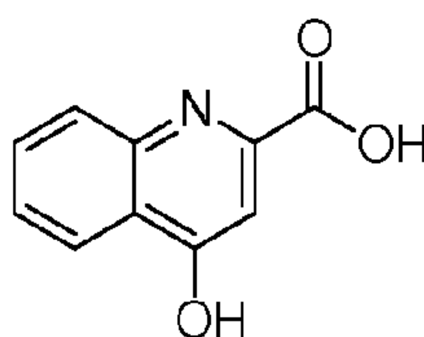
kynurenic acid
