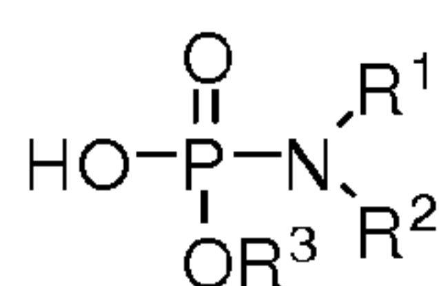
Phosphoramidate
