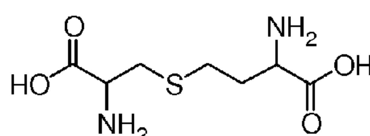
Cystathionine
