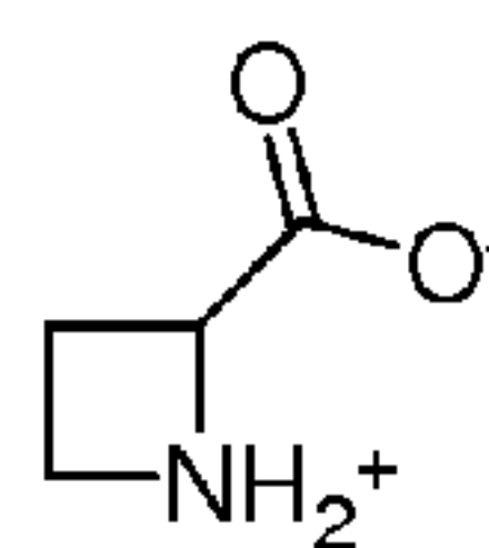
Azetidine-2-carboxylic acid
