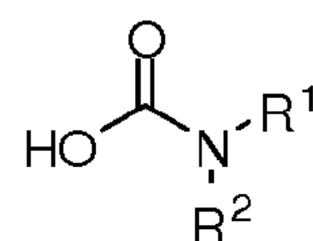
Carbamate
