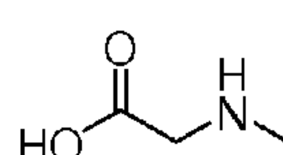
Sarcosine
