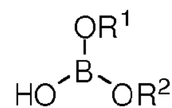
Borate
